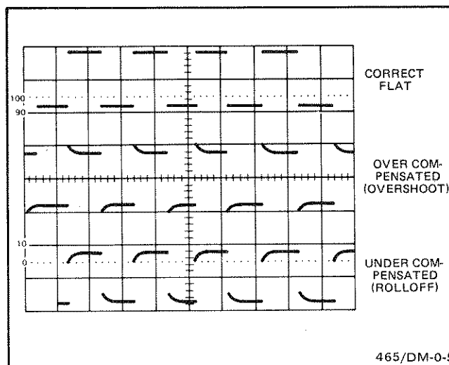
Figure 10. Probe compensation.
