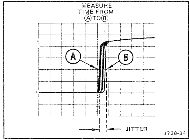
Figure 21. Pulse jitter.
