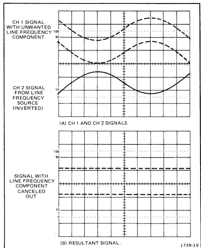
Figure 14. Common-mode rejection.
