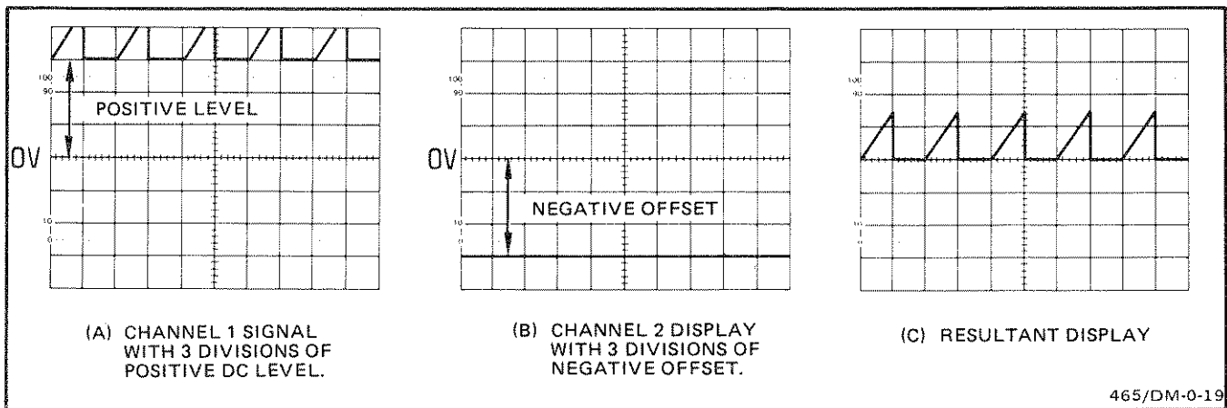
Figure 13. Algebraic addition.
