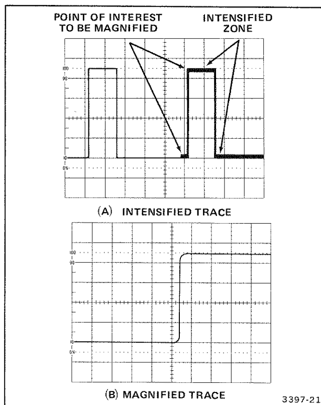
Figure 20. Delayed-sweep magnification.
