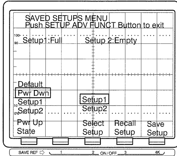
Figure 2-13: Save Setup Menu
