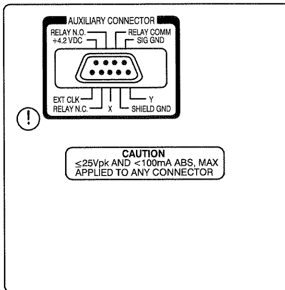
Figure 3-47: Auxiliary Connection
