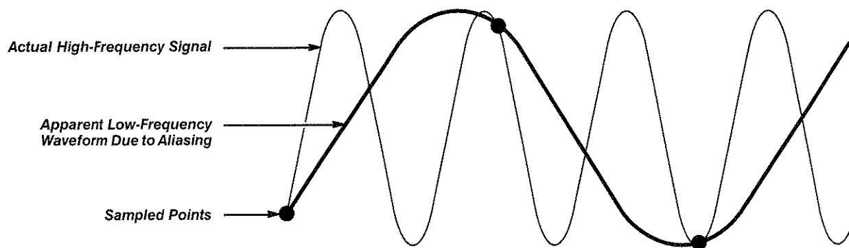
Figure 3-18: Aliasing
