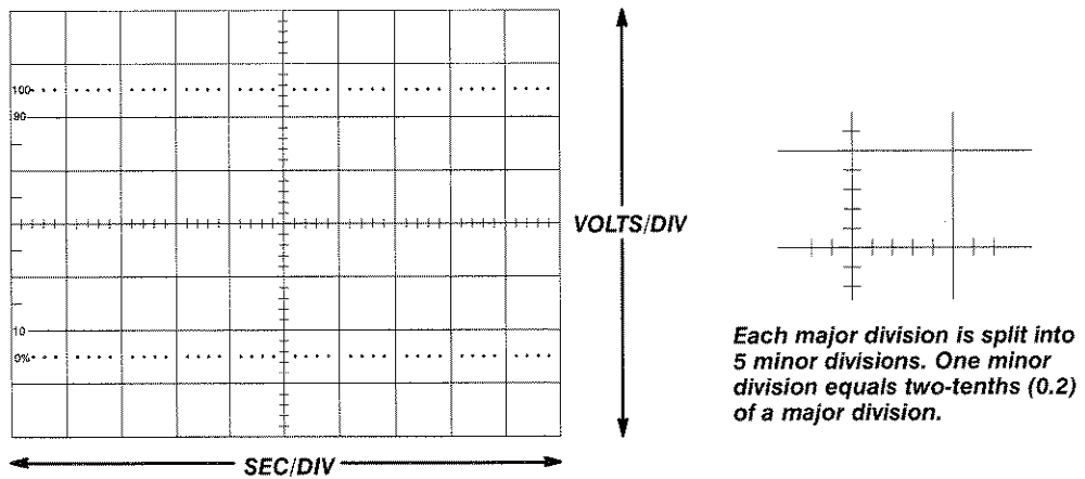
Figure 3-29: Measuring with the CRT Graticule
