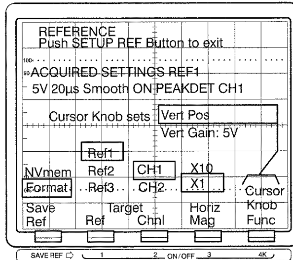
Figure 2-9: Format Reference Menu
