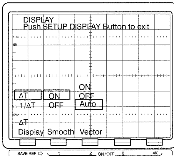
Figure 2-8: Display Menu
