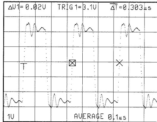
Figure 3-35: Period Measurement
