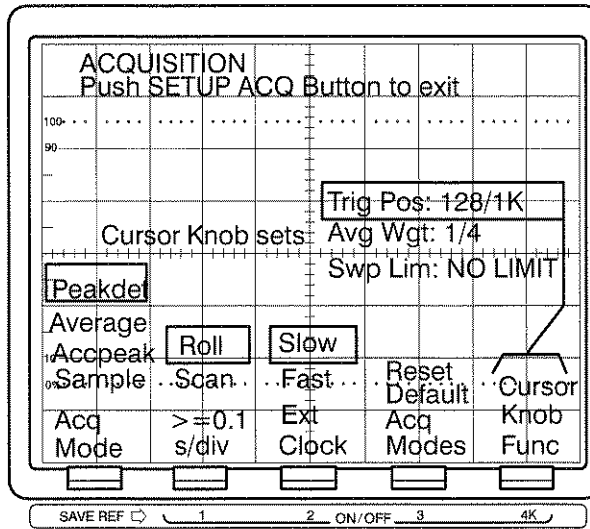
Figure 2-7: Acquisition Menu
