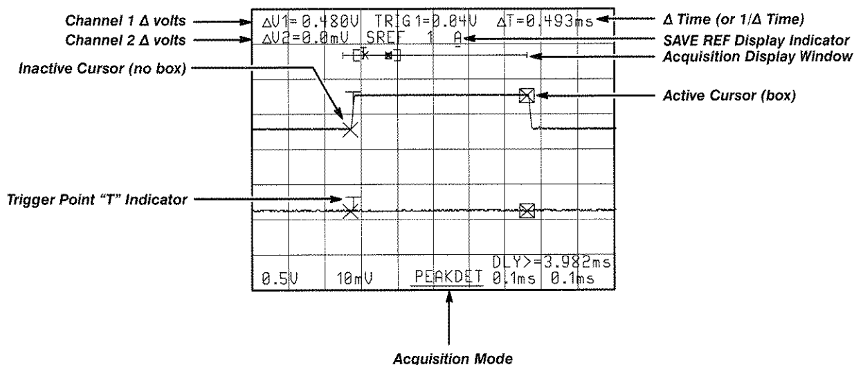
Figure 2-5: Digital (STORE) Mode Display
