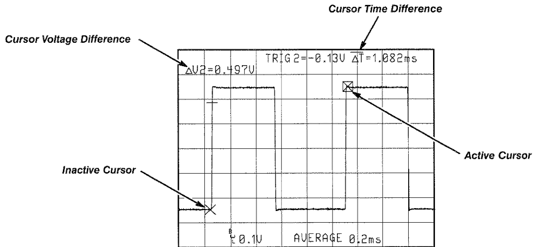
Figure 3-30: Cursor Measurements
