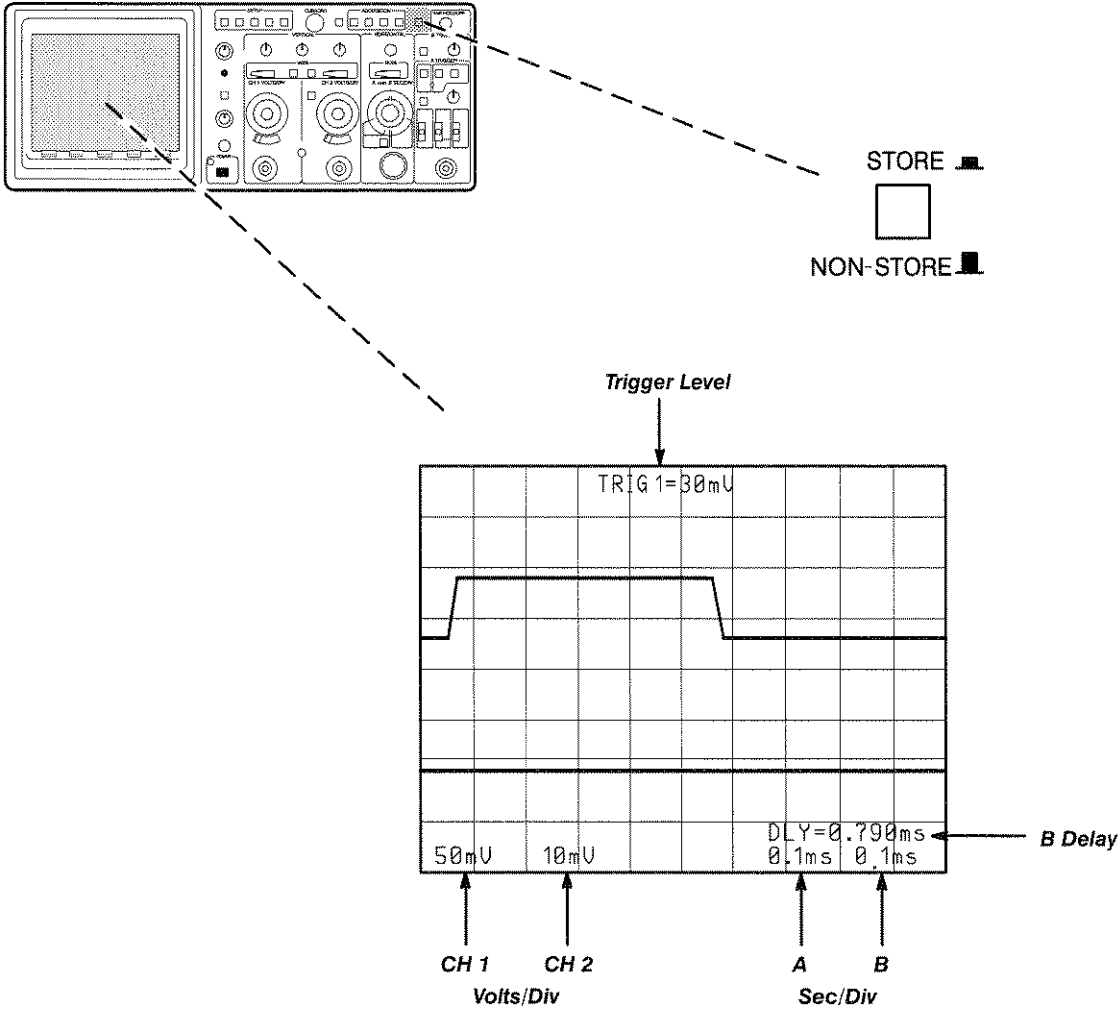
Figure 2-4: Analog (NON-STORE) Mode Display
