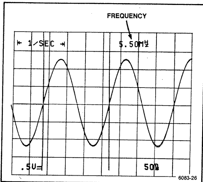
Figure 6-12. Frequency measurement.
