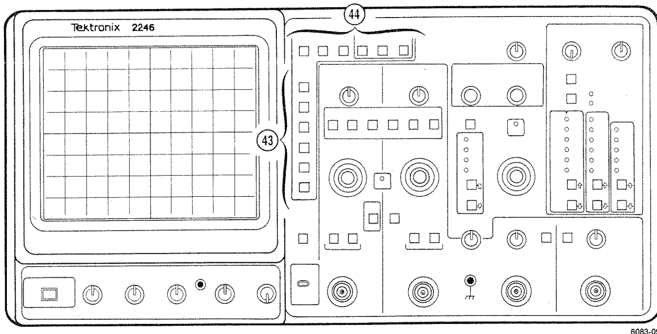
Figure 3-7. Menu Controls.
