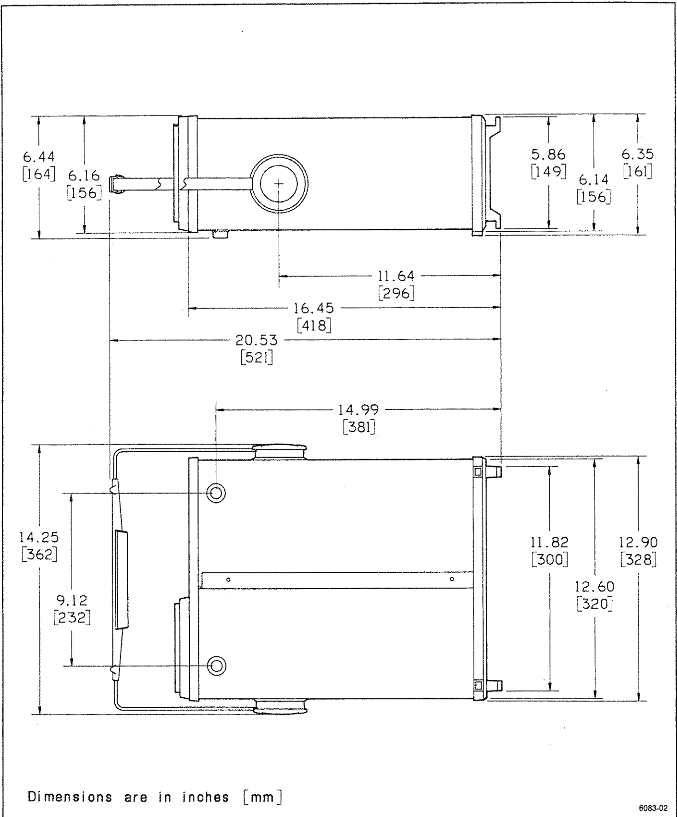
Figure 1-1. Dimensional drawing.
