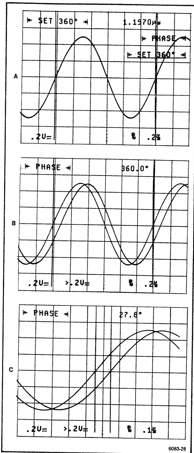
Figure 6-14. Making a phase difference measurement.
