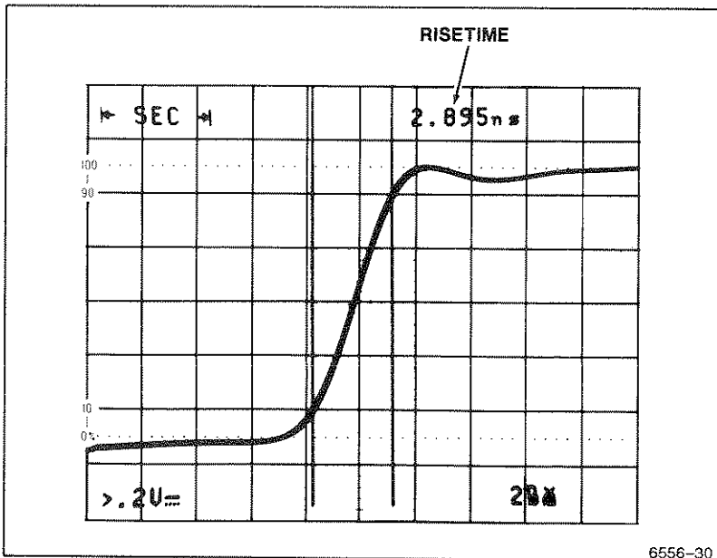
Figure 5-7. Rise time measurement.
