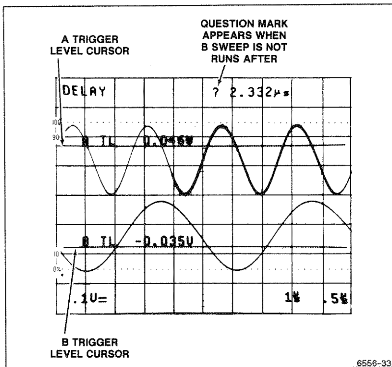
Figure 5-10. A and B Track Trig Lvl cursors.
