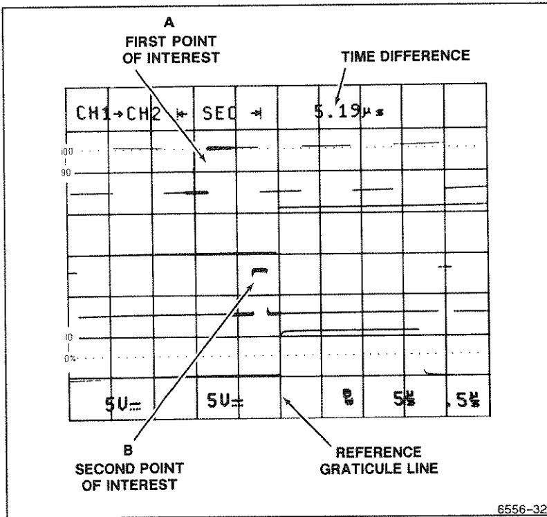
Figure 5-9. Time difference between the two delays.
