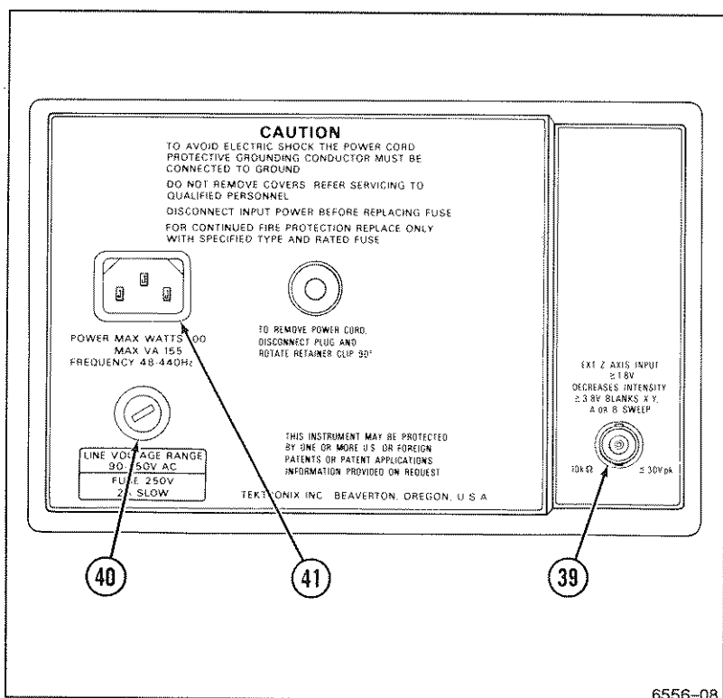
Figure 2-6. Rear panel.
