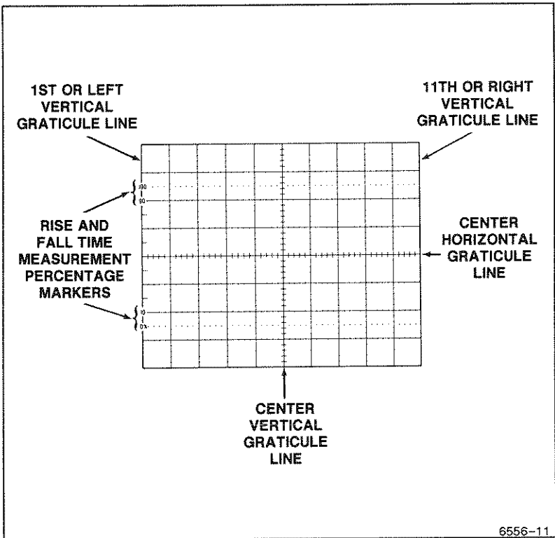
Figure 3-2. Graticule measurement markings.
