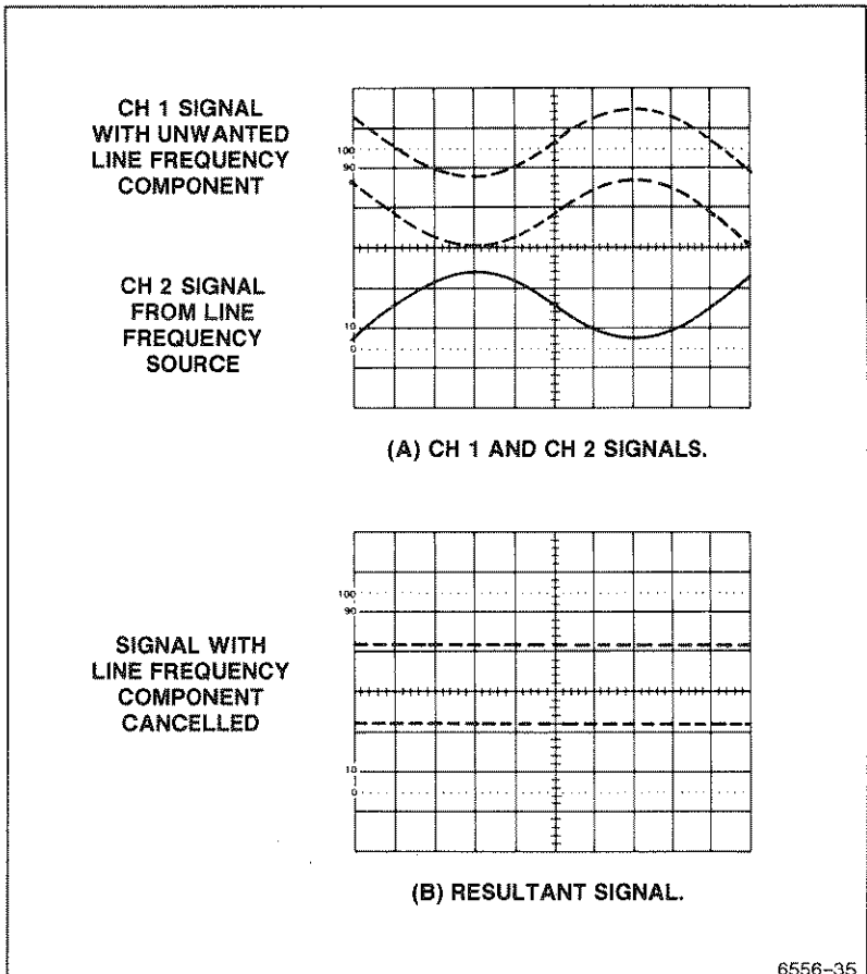
Figure 5-12. Eliminating common-mode signals.
