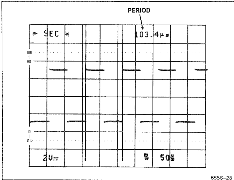
Figure 5-5. Period measurement.
