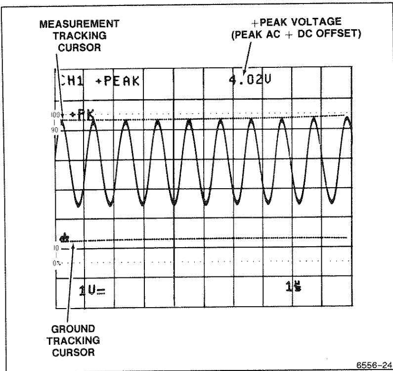
Figure 5-1. +PEAK voltage measurement and tracking cursors.
