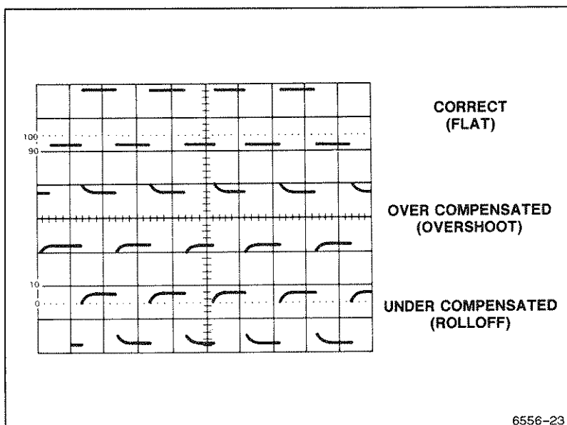
Figure 4-1. Probe compensation.
