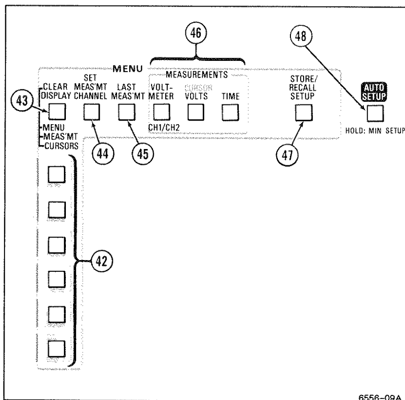
Figure 2-7. Menu controls.
