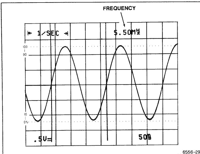
Figure 5-6. Frequency measurement.
