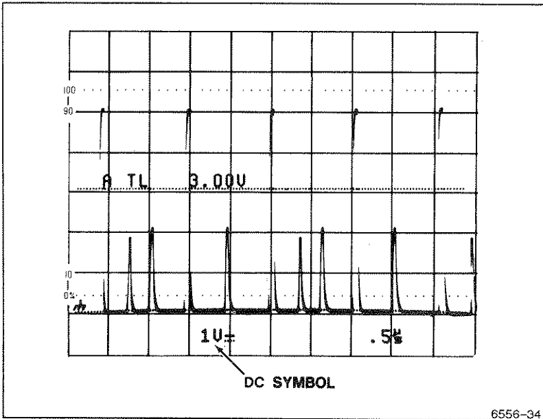
Figure 5-11. Setting a specific trigger level.
