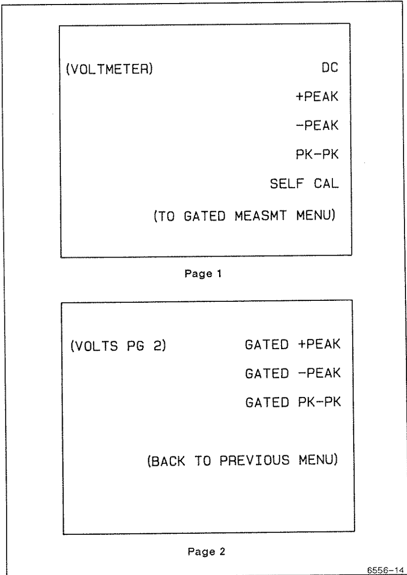
Figure 3-5. Voltmeter and Gated Measmt menus.
