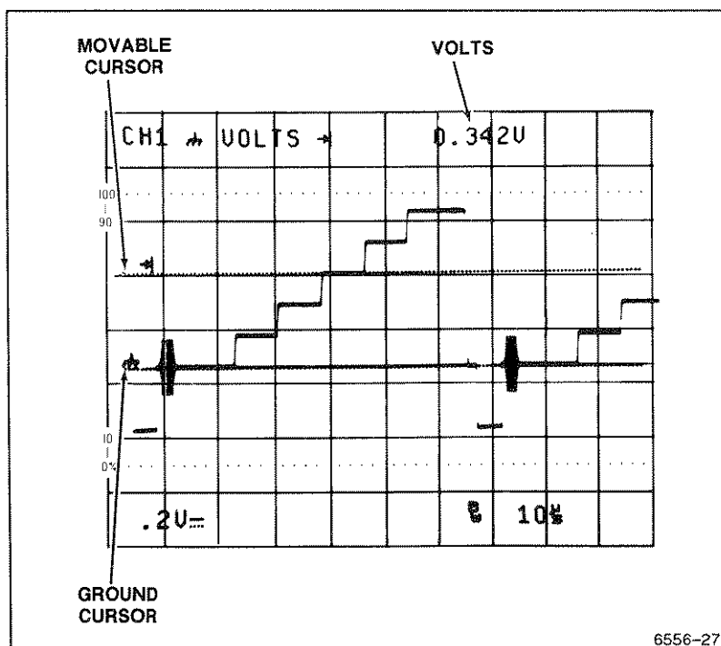
Figure 5-4. Voltage measurement.
