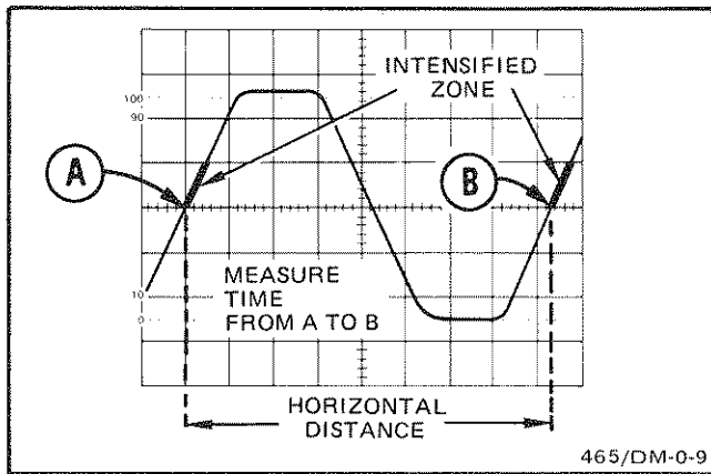
Fig. 26. Time duration.
