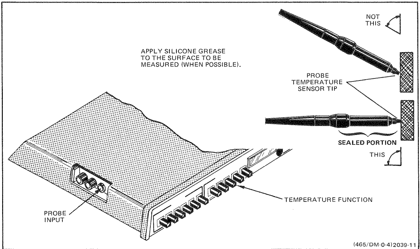
Fig. 10. Temperature.
