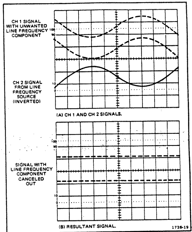
Figure 17. Common-mode rejection.
