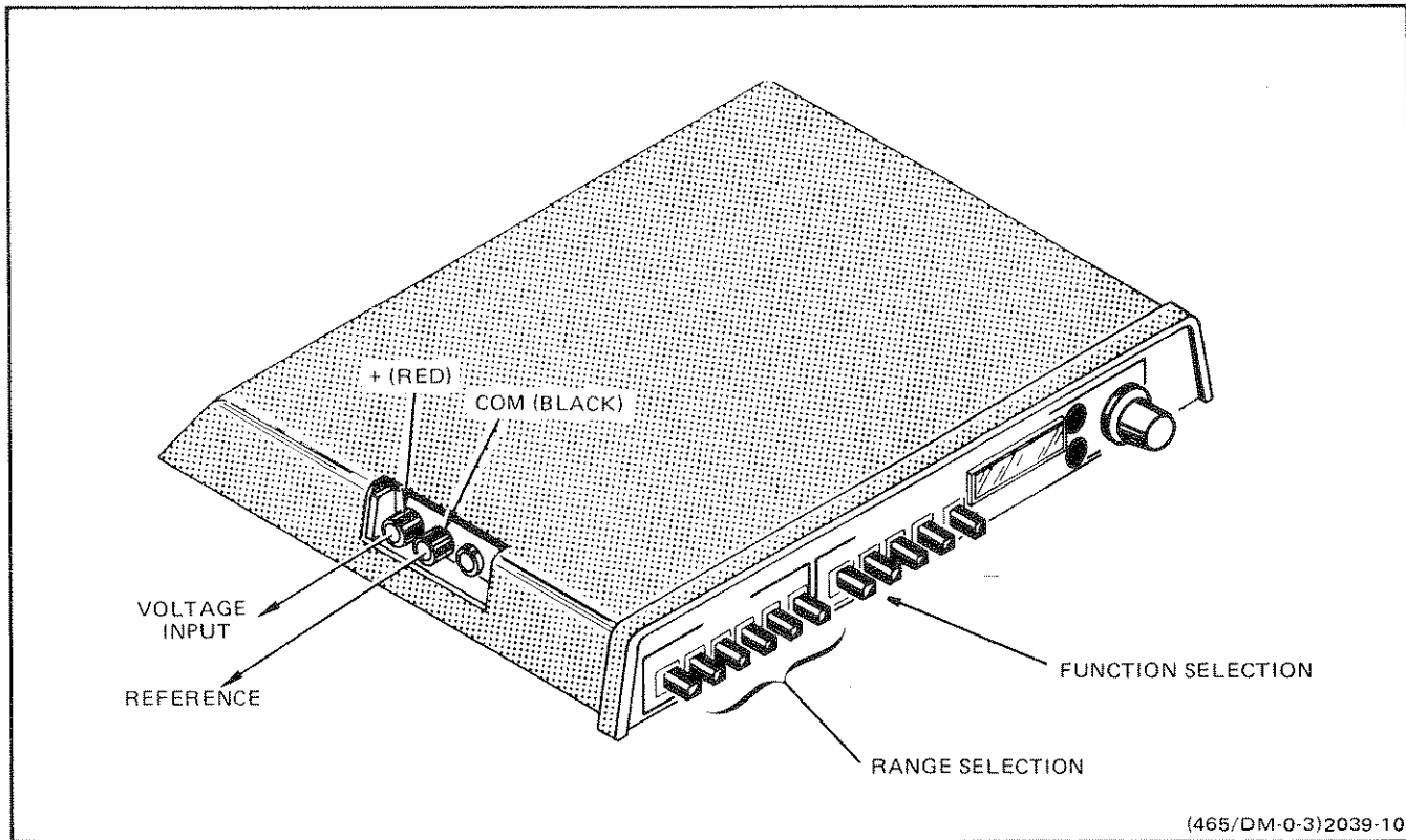
Fig. 9. Volts.
