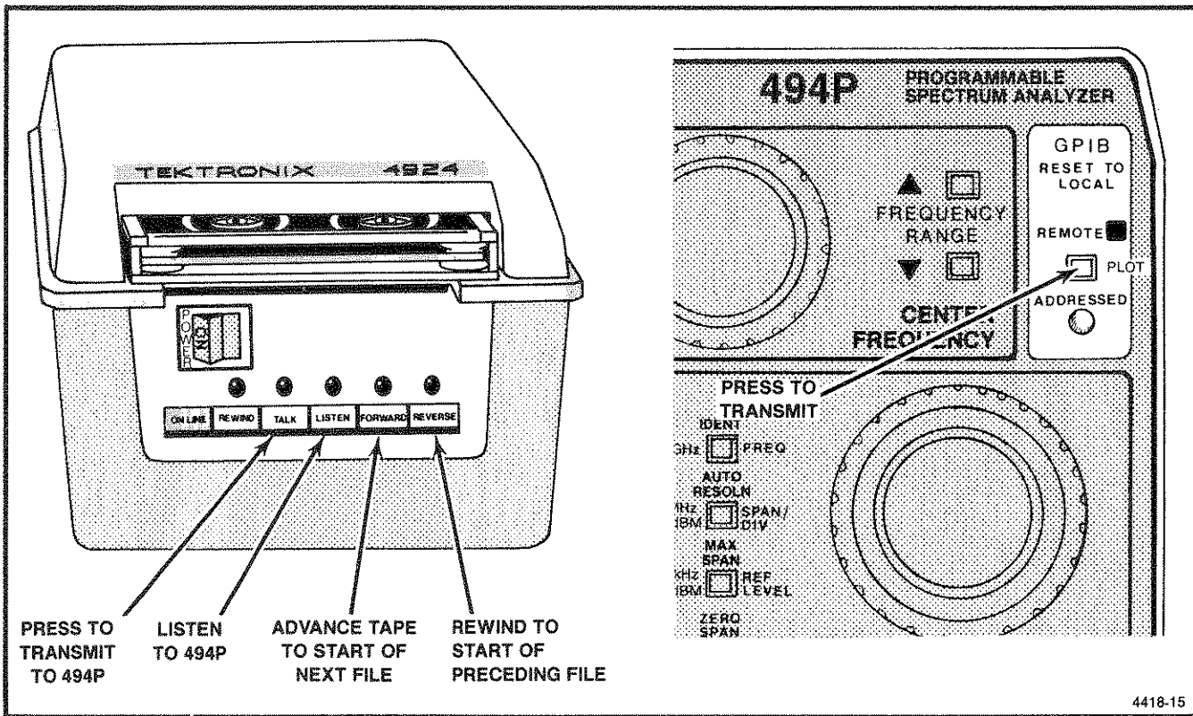
Figure 6-14. Controls on the 4924 and 494P that are used for the Talk/Listen Only transfers.
