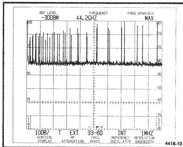
Figure 6-9. Typical display from an external mixer.
