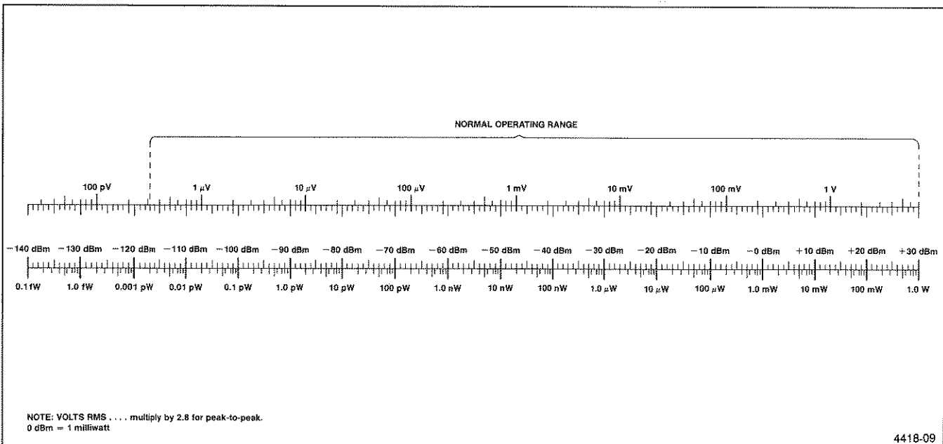
Figure 6-1. Volts-dBm-Watts conversion chart for 50 Ω impedance.
