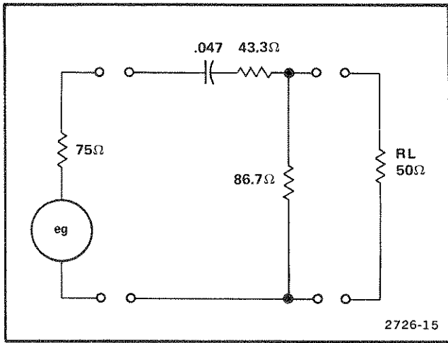
Figure 6-2. Circuit of a 75 to 50 Ω matching pad (ac coupled).
