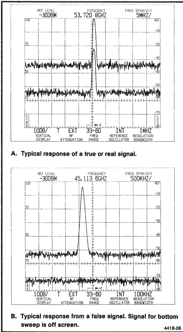
Figure 5-4. Using IDENT feature to identify a real or true response.
