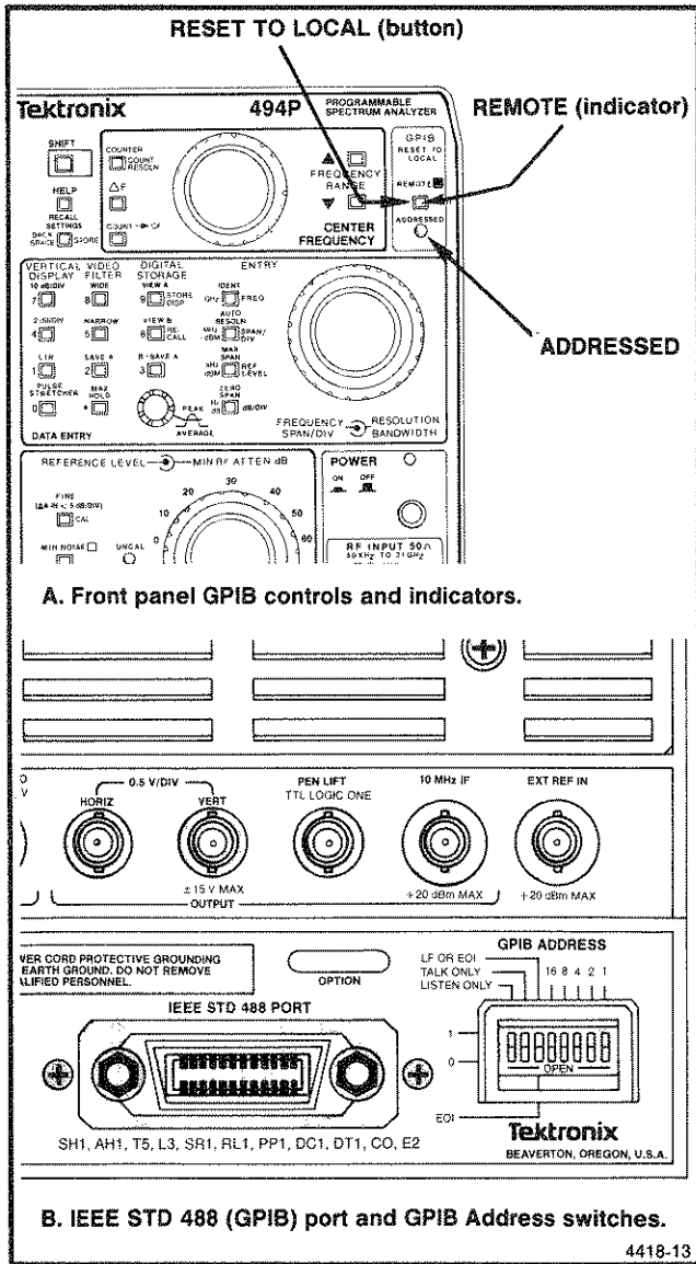
Figure 6-10. GPIB selectors and indicators unique to the 494P.
