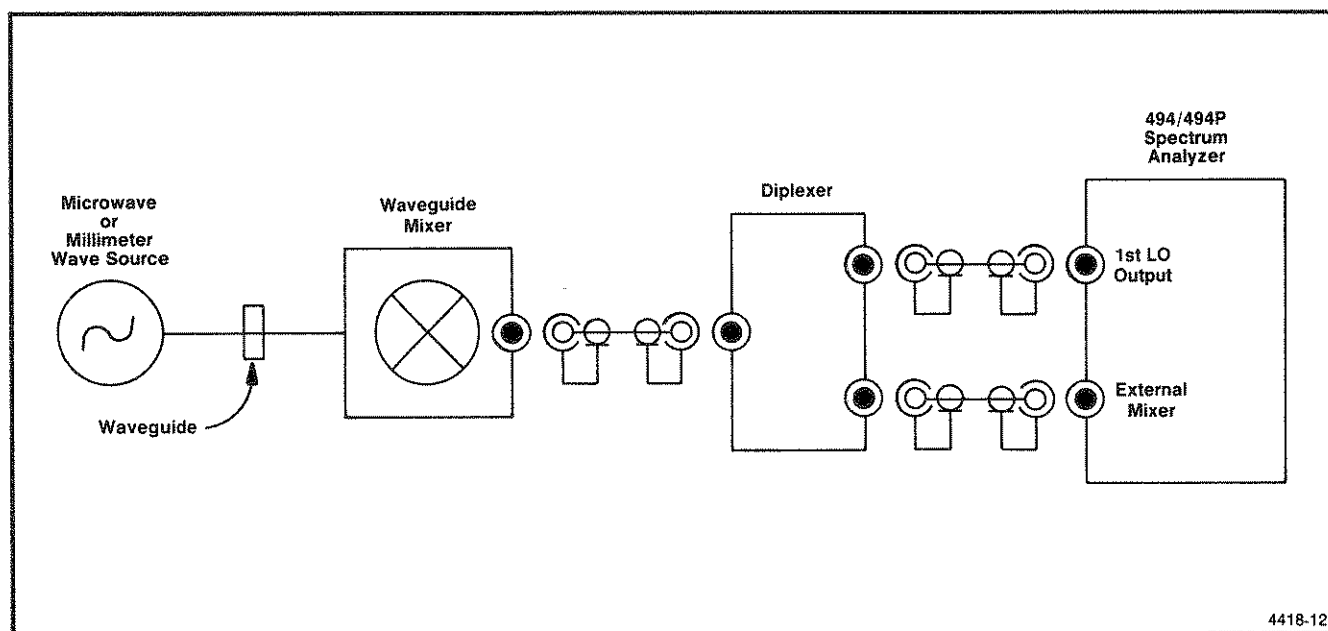
Figure 6-8. Diagram showing external waveguide mixer installation.
