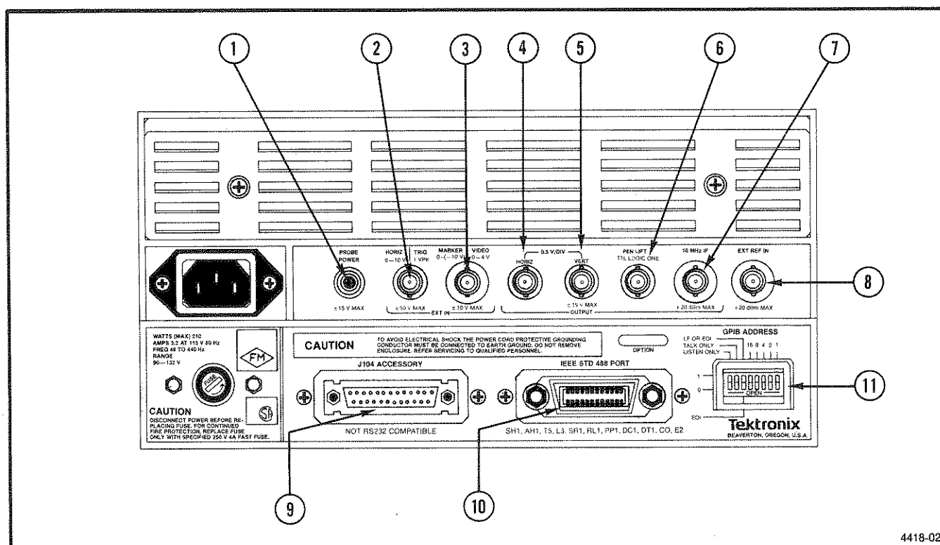
Figure 4-2. Rear panel connectors on the 494/494P.
