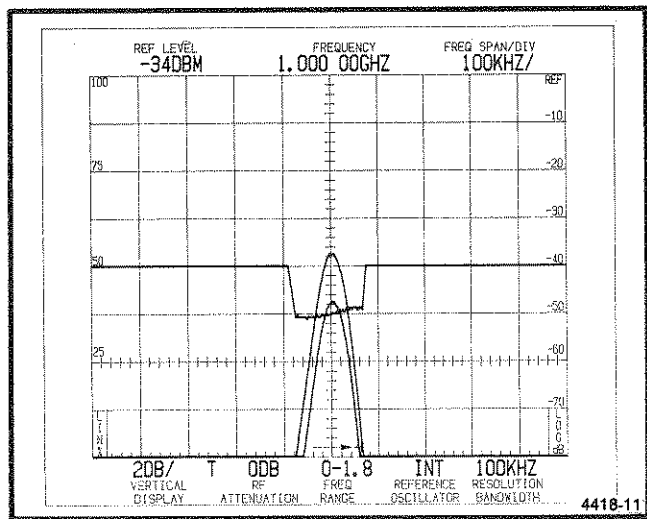
Figure 6-7. Using B-SAVE A to observe the differential between SAVE A and B displays.
