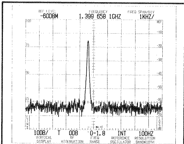
A. Spurious and IM obscured in the noise.
