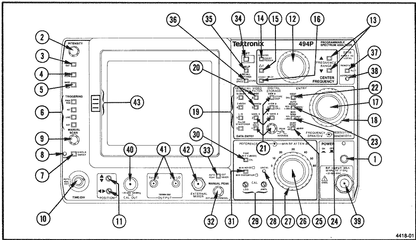
Figure 4-1. Front panel selectors, controls, and connectors.
