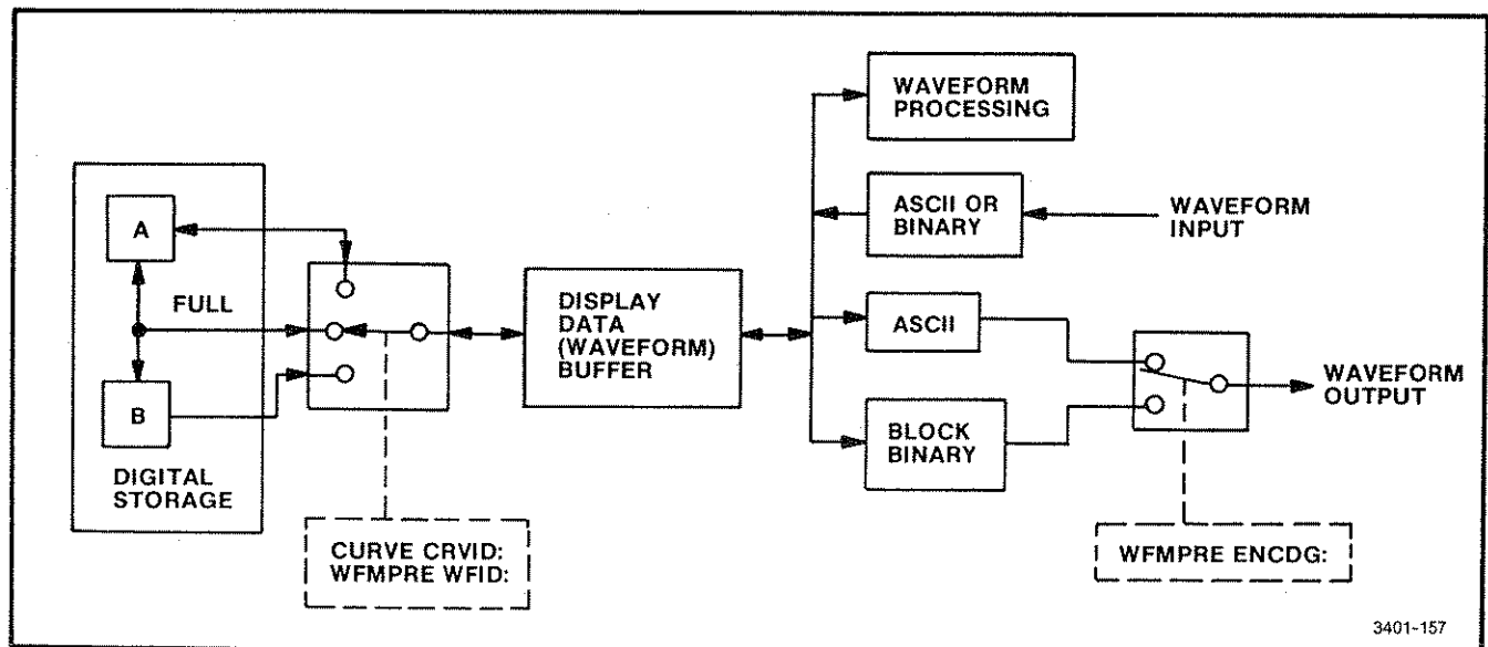
Figure 8-3. How multiple use of the display data buffer is controlled.
