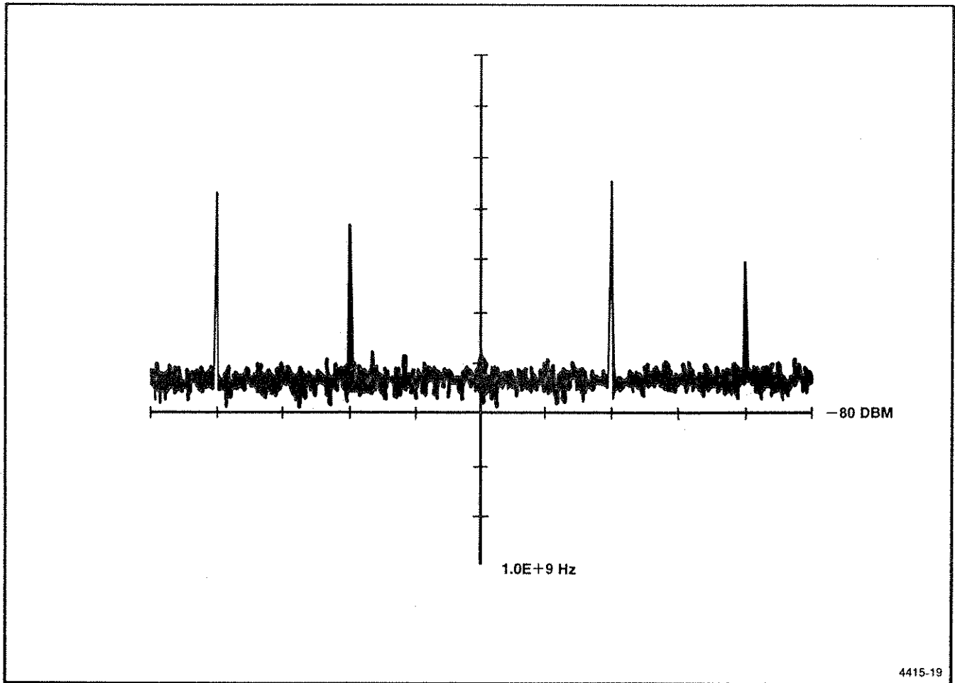
Figure 8-2. A simple plot of a spectrum acquired from the 494P.
