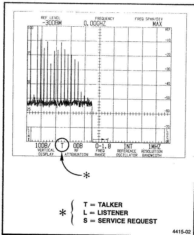
Figure 1-2. Status of active GPIB functions.
