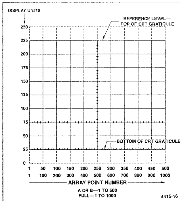
Figure 5-1. Waveform data related to the display.
