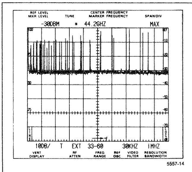
Figure 6-12. A typical display from an external mixer.
