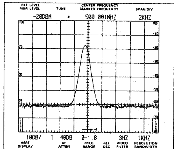
B. Same display with Video Filter activated.
