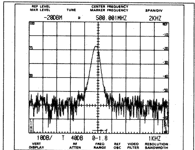
A. Spurii and IM obscured in the noise.
