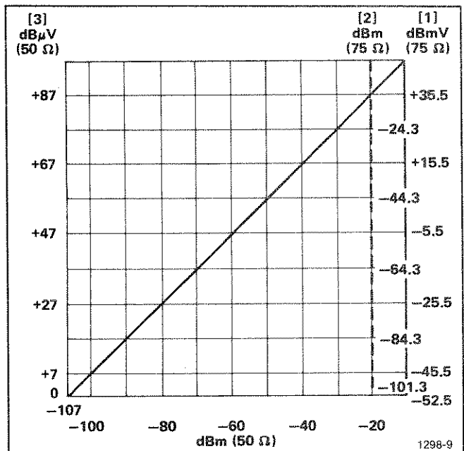
Figure 6-2. Graph illustrating the relationship between dBm, dBmV, and dBμV (matching attenuator included where necessary). When the alternate 75 Ω input is used, the reference level readout is correct for any units without additional conversions.
