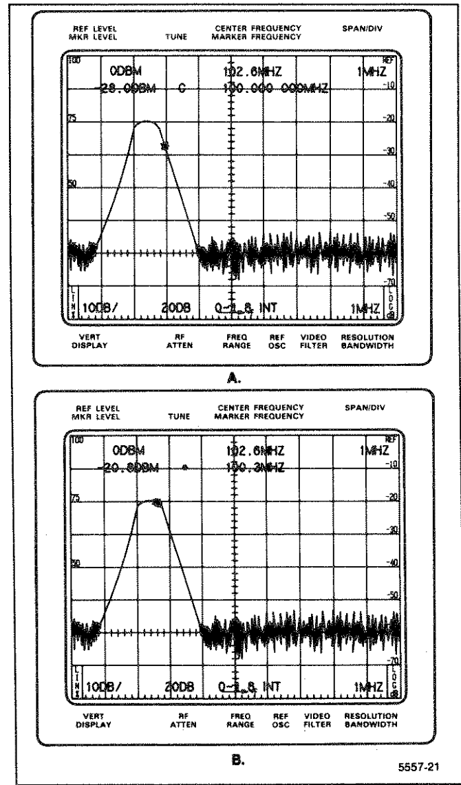
Figure 6-8. Simulated display of stored displays with signal counts. (A) Display when the marker has just been assigned/reassigned to the trace. (B) Display after the marker is tuned.
