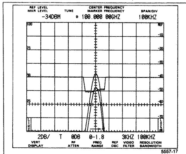
Figure 6-6. Typical display using B-SAVE A to observe the difference between SAVE A and B displays.
