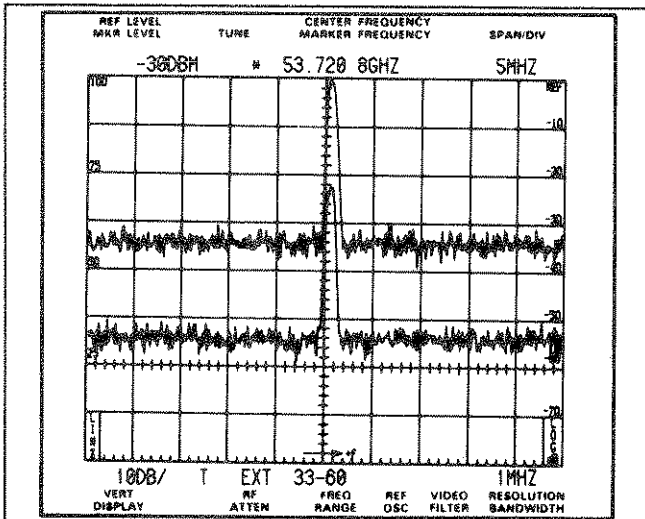
A. Typical response of a true or real signal.
