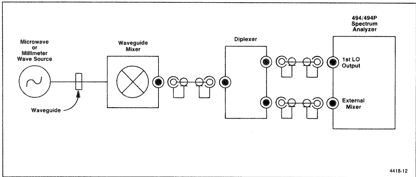
Figure 6-11. Block diagram showing external waveguide mixer installation.
