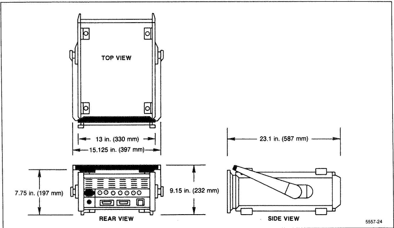
Figure 2-1. Dimensions.
