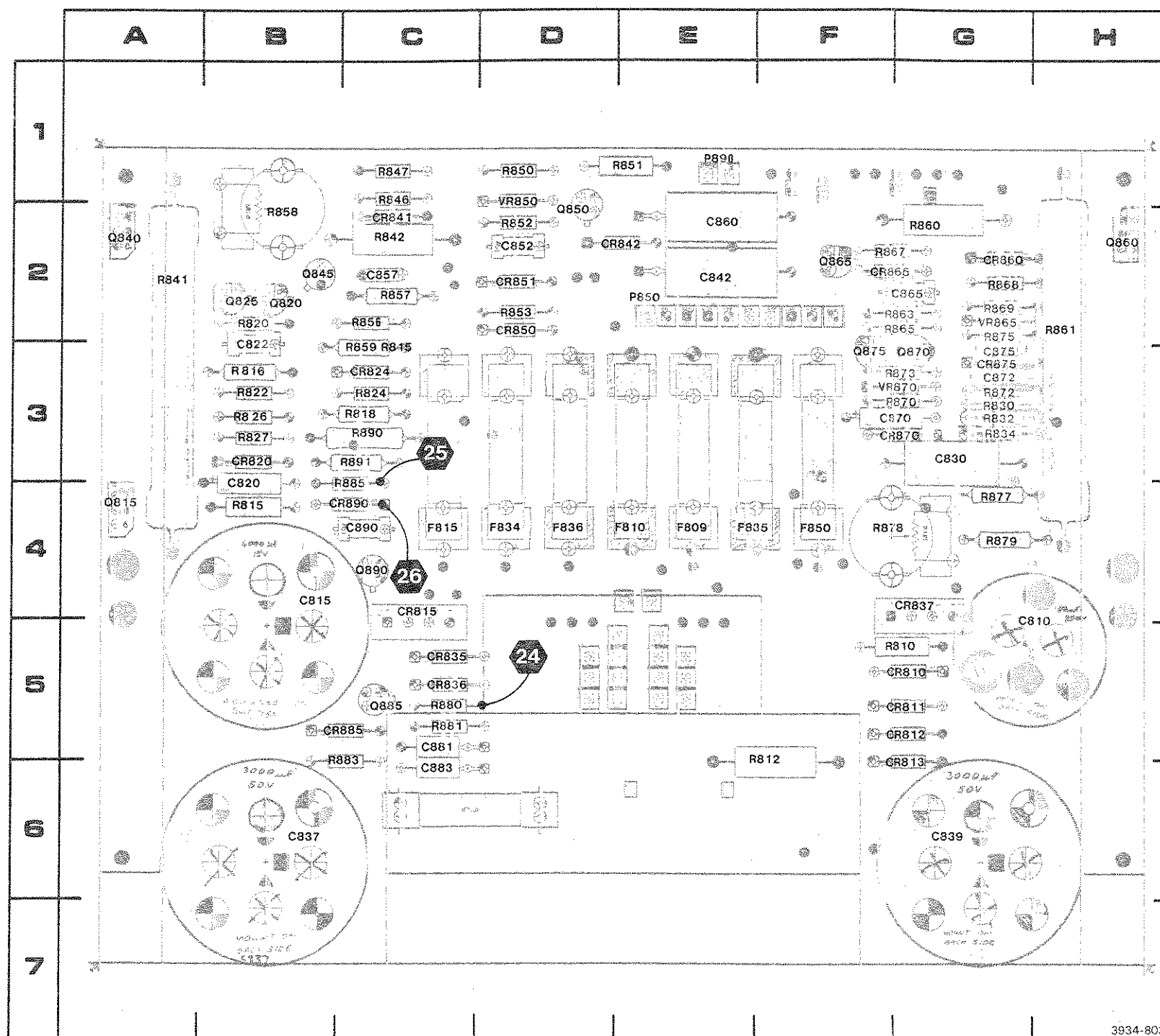
Figure 8-5. A2-LV Power Supply circuit board assembly.
