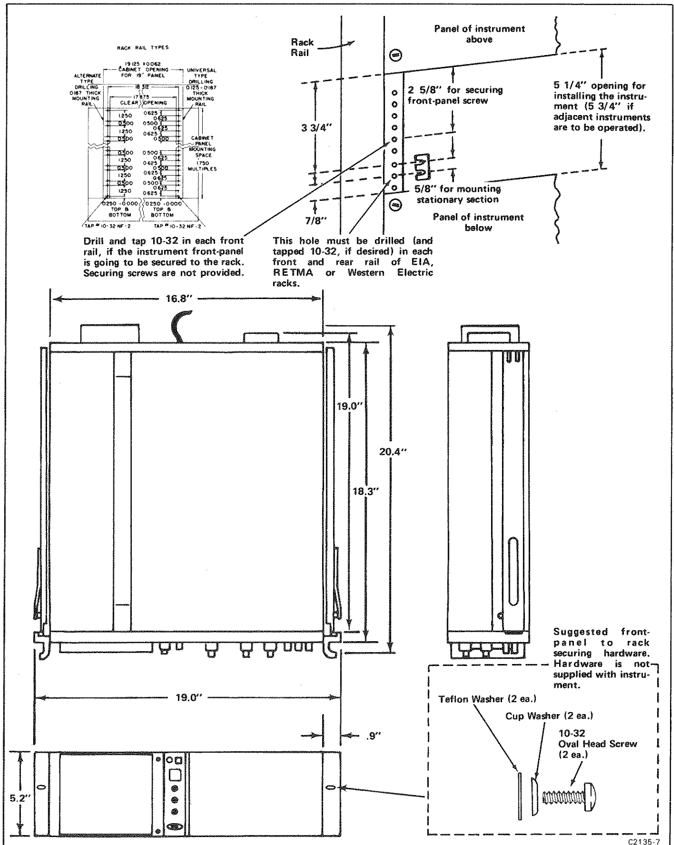
Fig. 4-3. Dimensional diagram.
