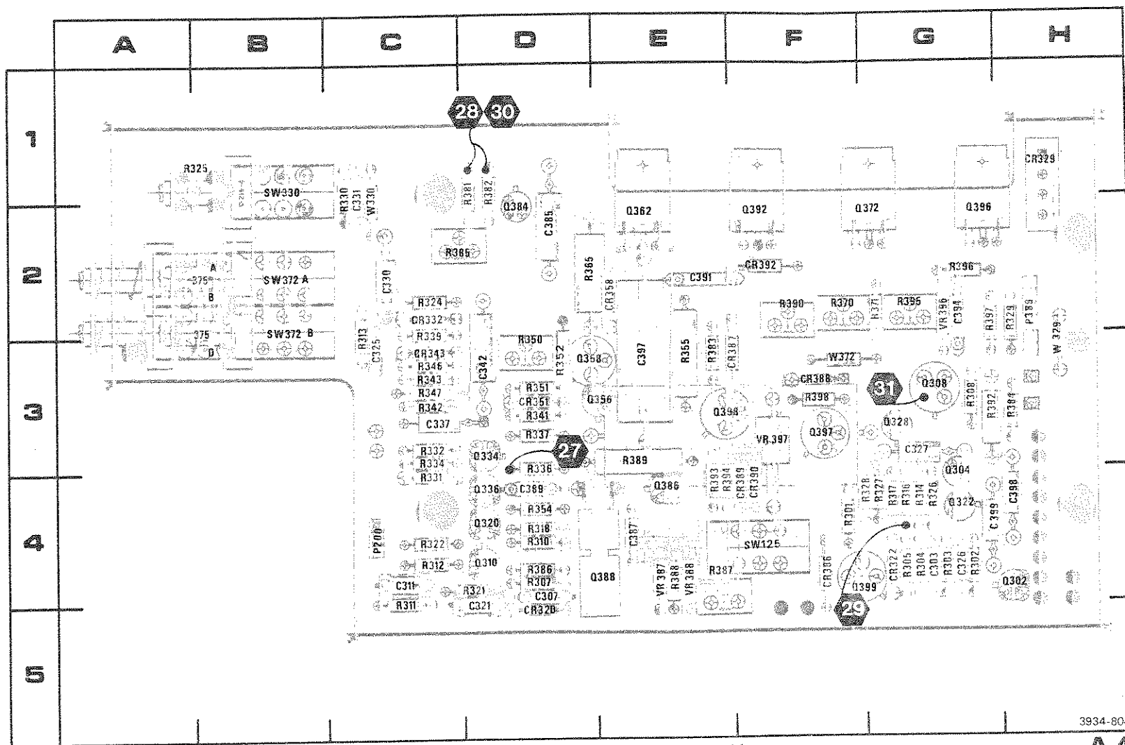
Figure 8-6. A4-Storage circuit board assembly.
