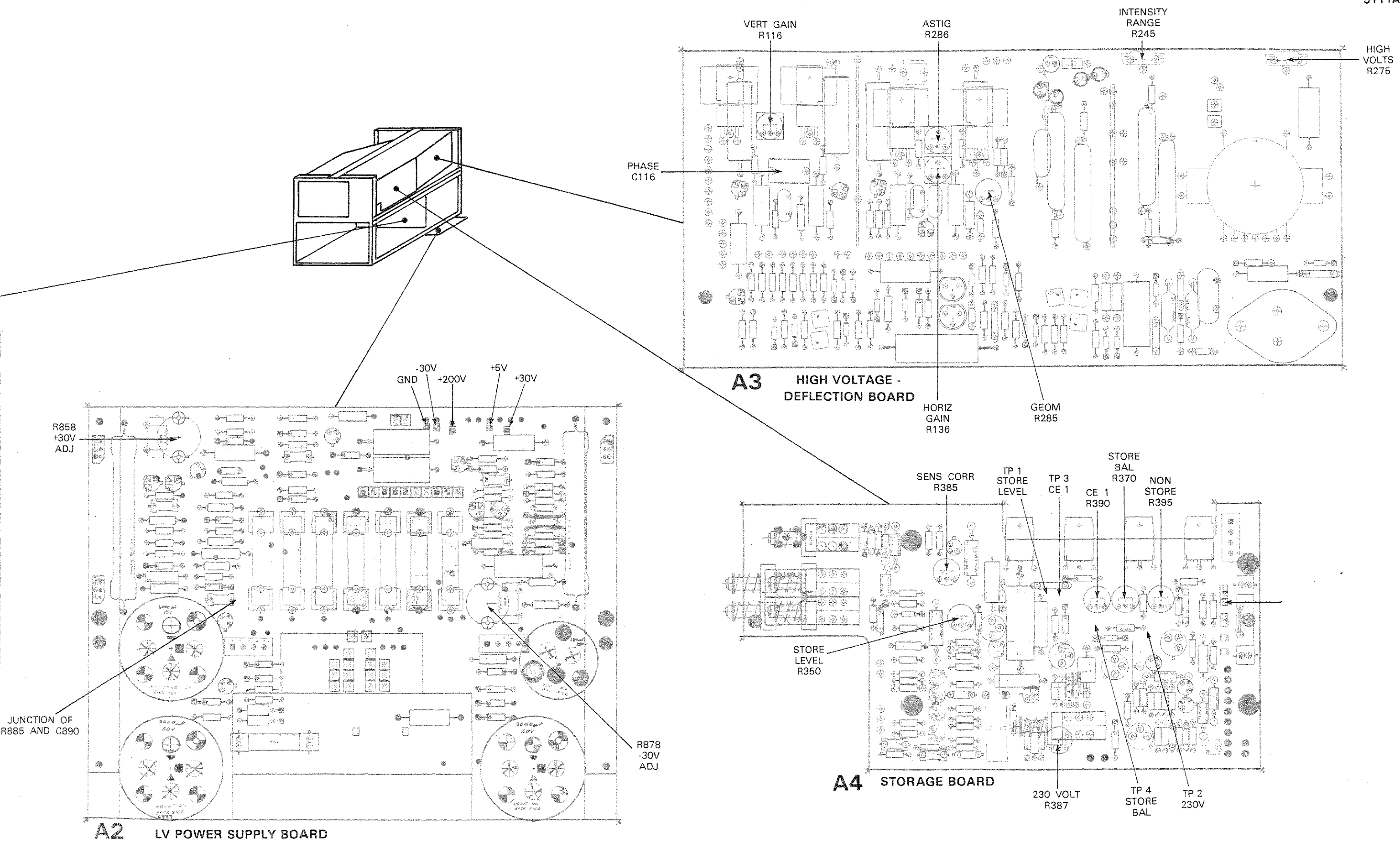
Figure 8-2. Test Point and Adjustment Locations.
