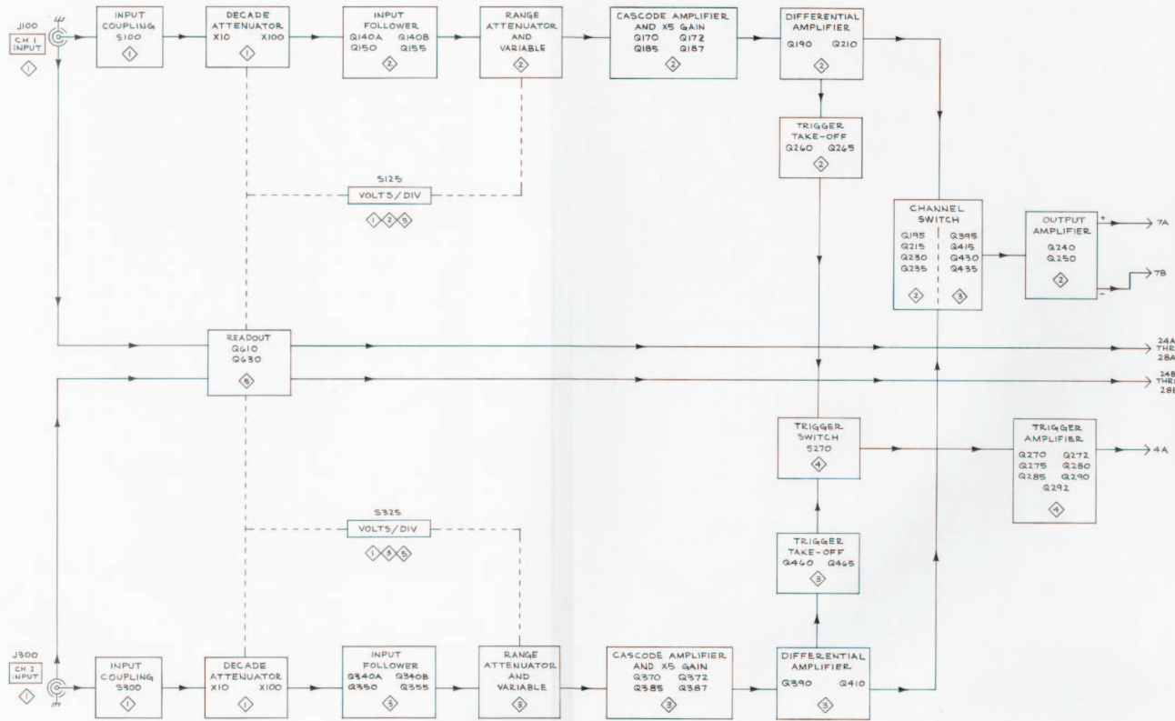
Block Diagram 5A48
