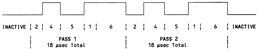
Figure 270-2: Sample Waveform TTL BNC Output
