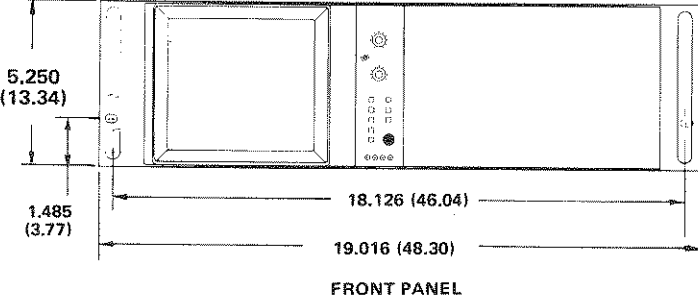
Fig. 3-6. Dimensional drawing.
