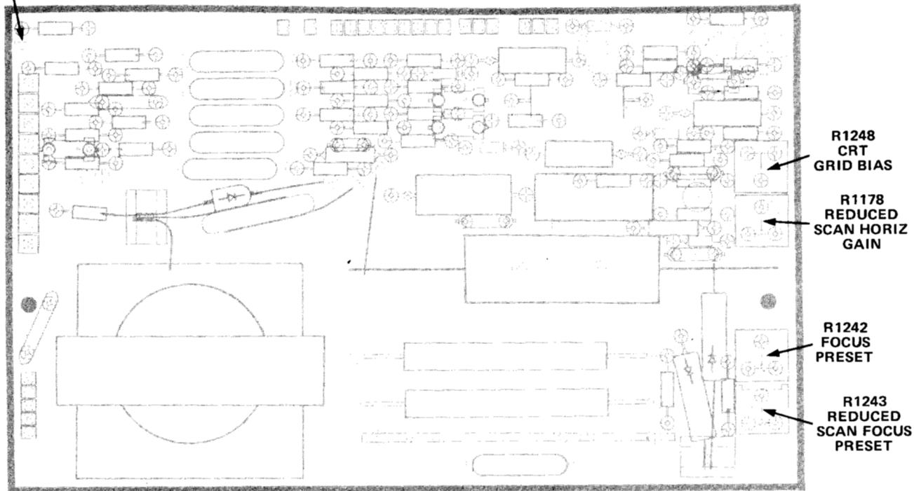
Figure 8-18. High-Voltage board.
