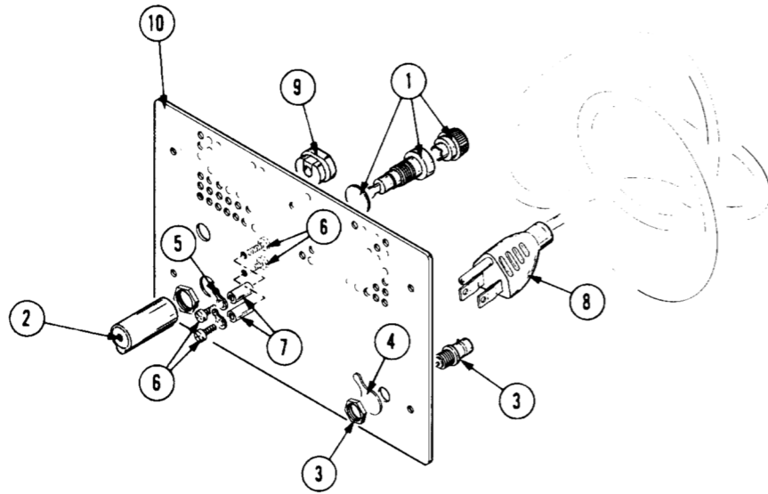
7633/R7633 OSCILLOSCOPE
