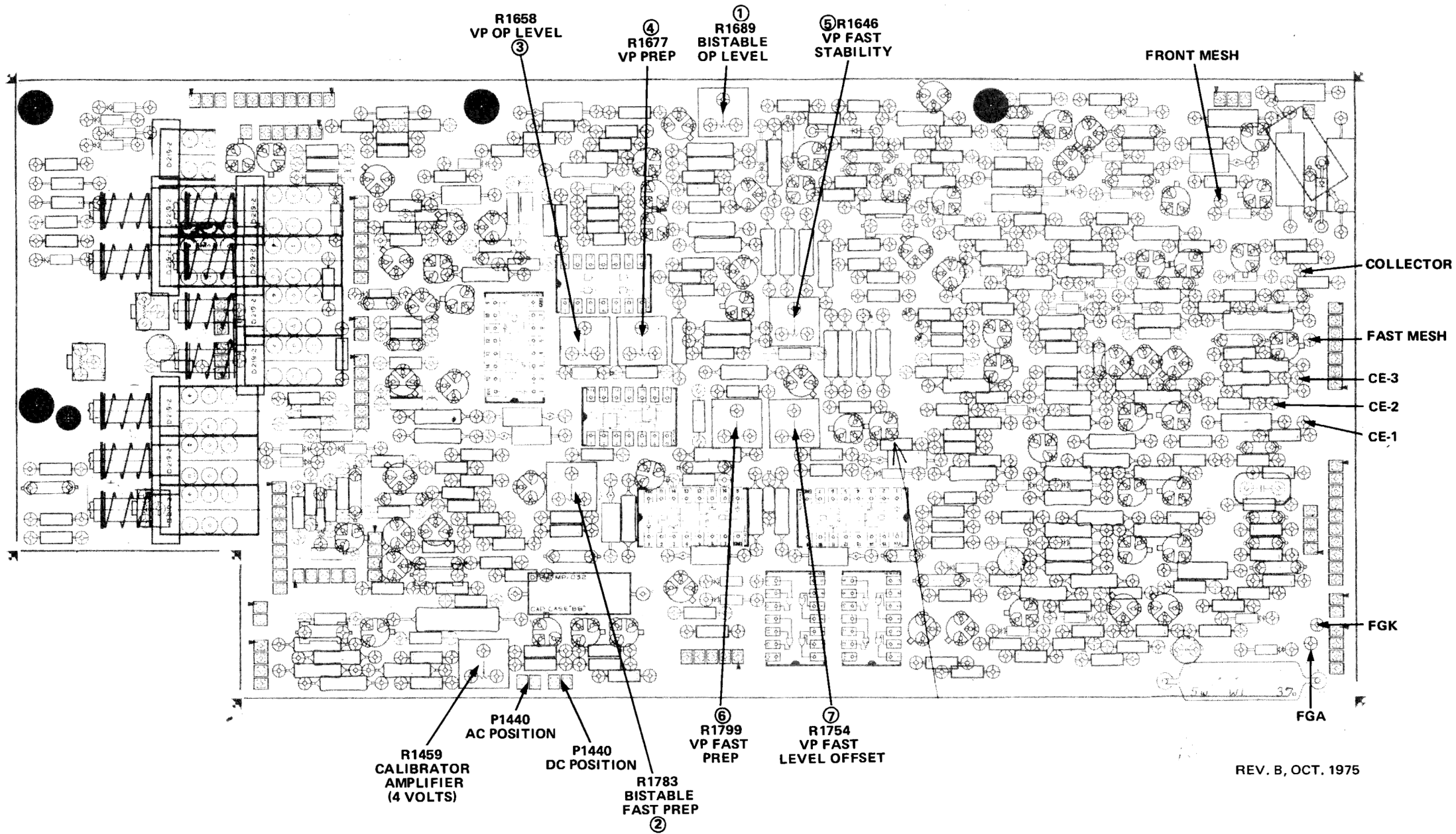
Figure 8-24. Storage board.
