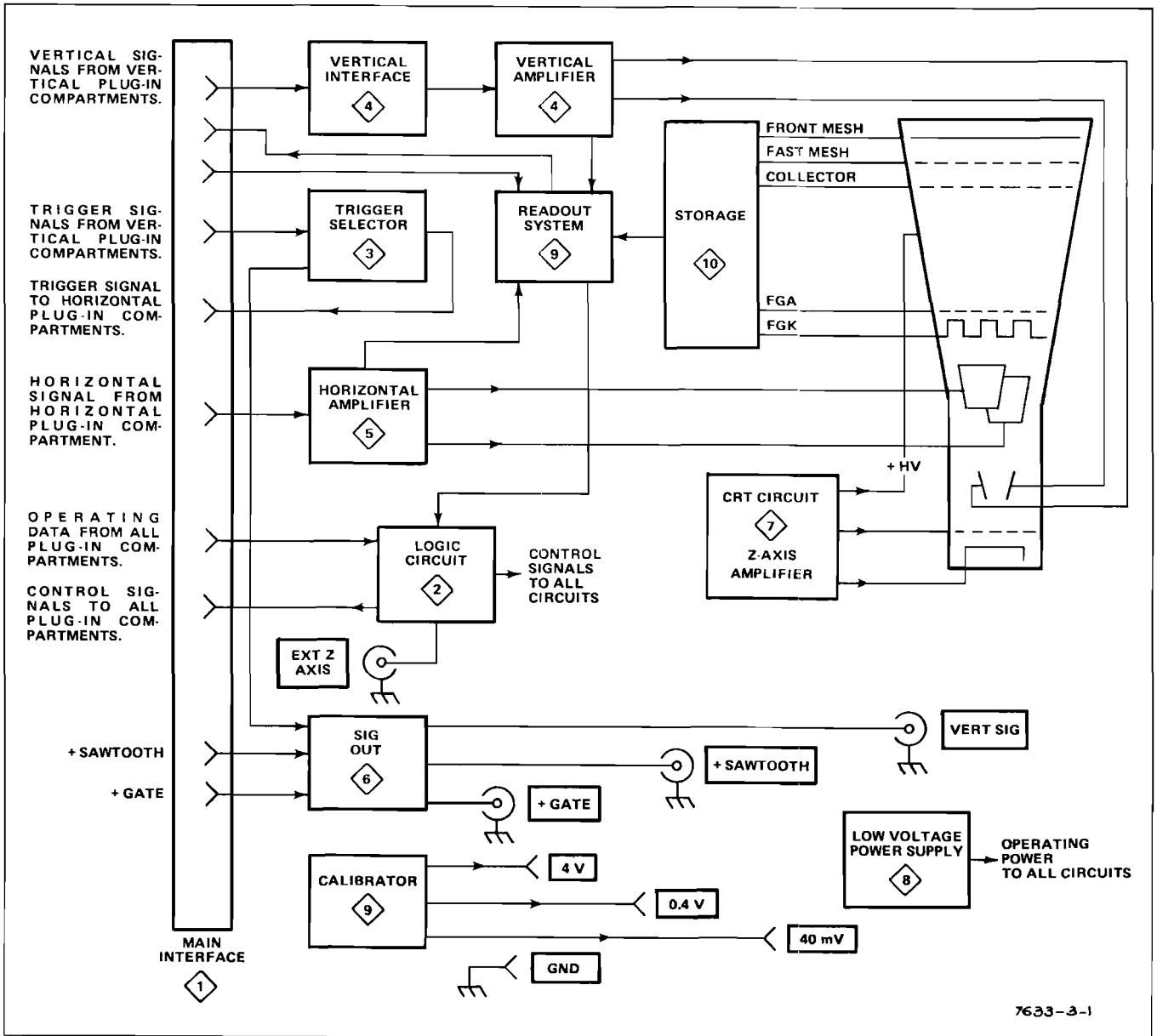
Figure 3-1. Block diagram 7633.
