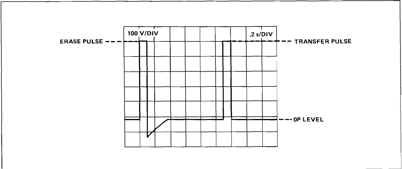
Figure 5-9. Idealized Erase and Transfer waveform.
