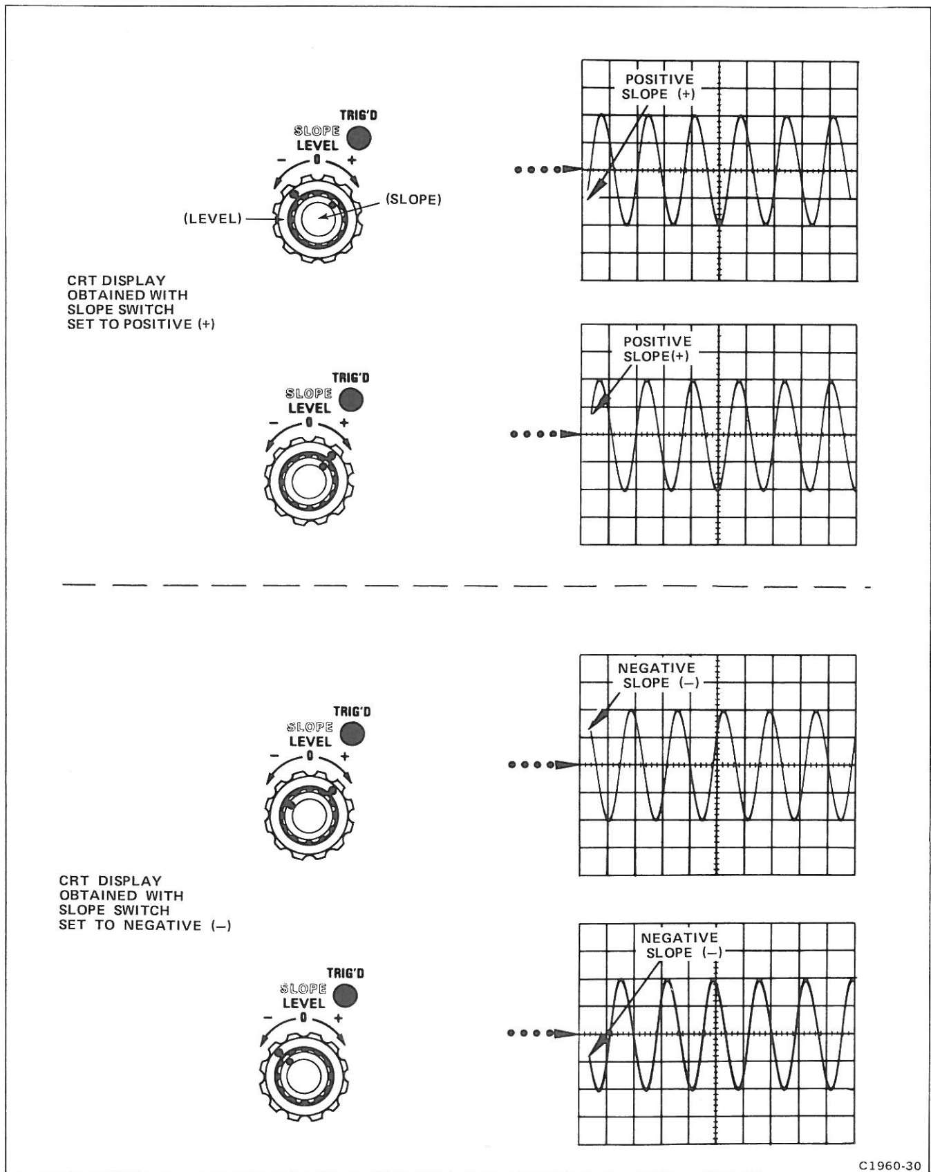
Fig. 1-3. Effects of LEVEL control and SLOPE switch on crt display.
