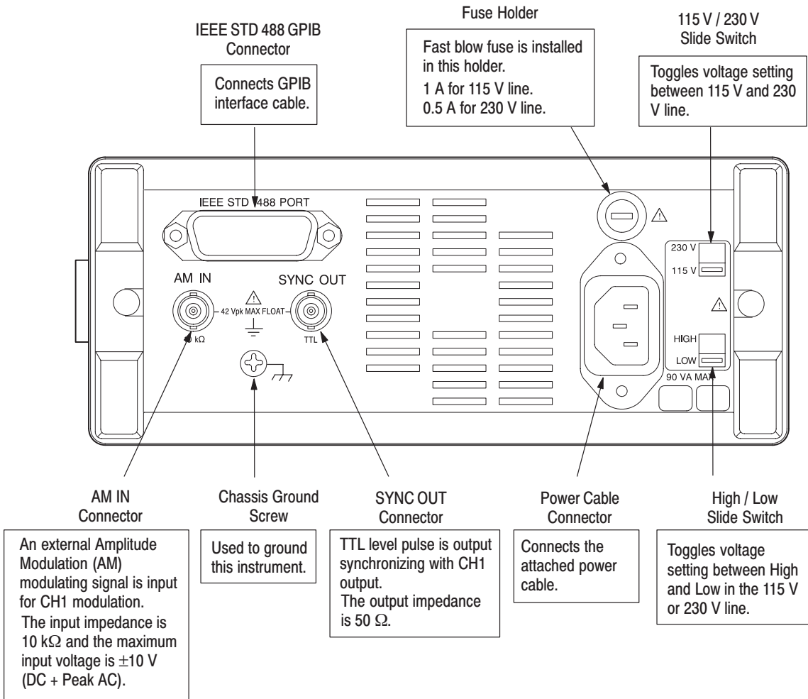
Figure 2–2: Rear Panel
