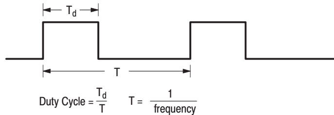
Figure 3-8: Pulse Duty
