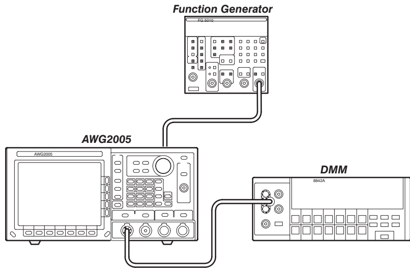
Figure E-10: External AM Operation Initial Test Hookup
