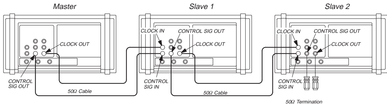
Figure 4C-9: AWG2005 Parallel Operation
