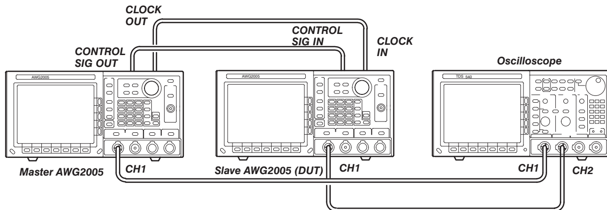
Figure E-21: Slave Operation Initial Test Hookup
