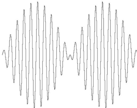
Figure 3-9: 100% Amplitude Modulation
