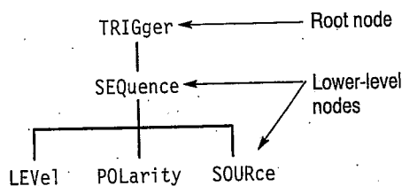
Figure 2-1: Example of SCPI subsystem hierarchy tree
