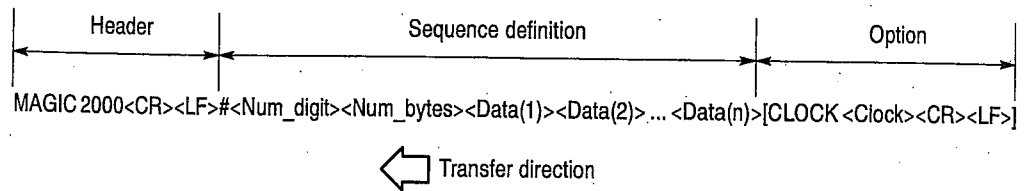
Figure 2-8: The Pattern File format
