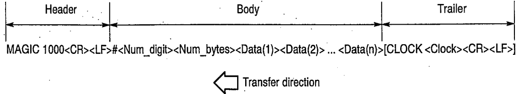
Figure 2-7: The Waveform File format
