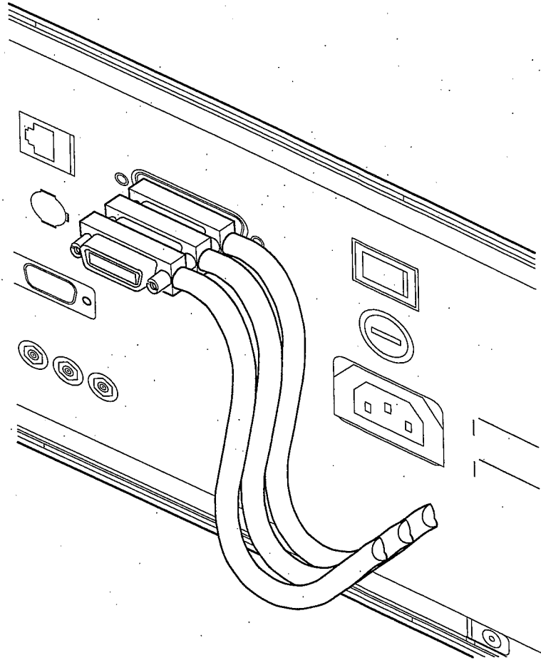
Figure 1-6: How to stack GPIB connectors
