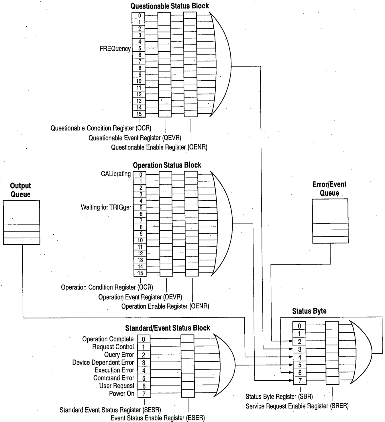
Figure 3-1: Error and Event handling process overview
