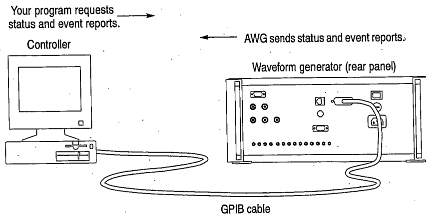
Figure 1-3: The status reporting function provides for event driven programs
