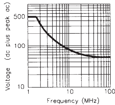
Figure 5: Typical voltage derating versus frequency
