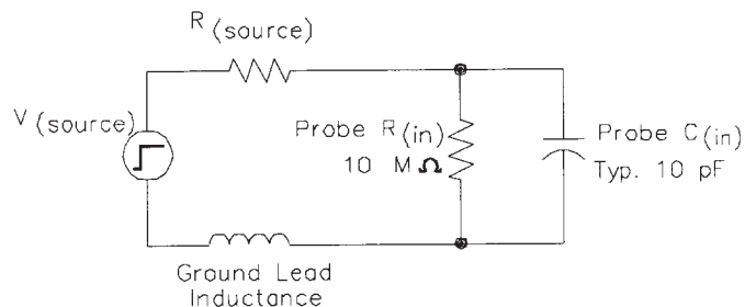
Figure 1: Schematic representation of probe
