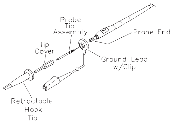
Figure 9: Probe tip assembly
