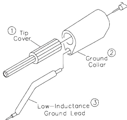
Figure 3: Low-inductance lead
