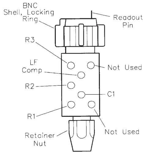
Figure 6: Location of compensation adjustments
