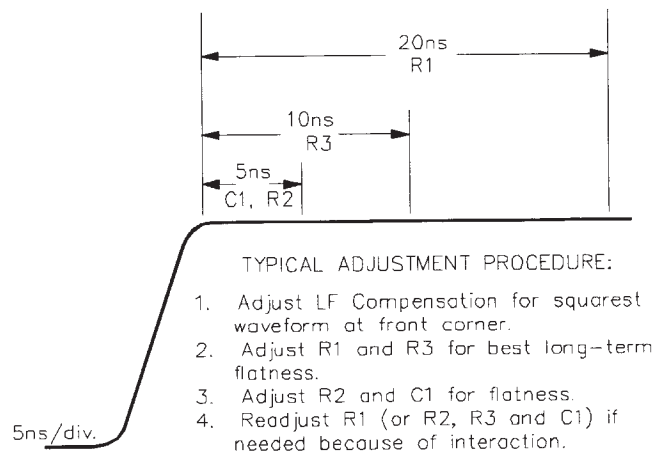
Figure 7: Effect of compensation adjustments
