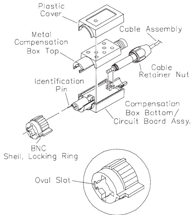
Figure 8: Compensation box assembly
