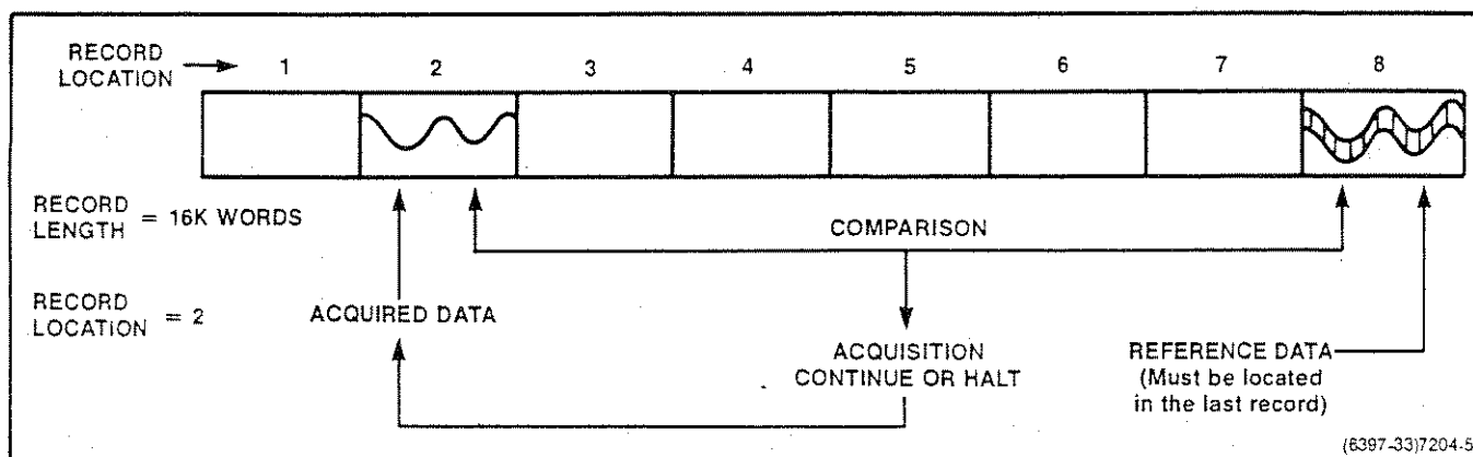
Fig. 3-20. COMP-IN trigger mode representation.
