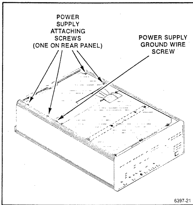
Fig. D-3. Power supply removal.
