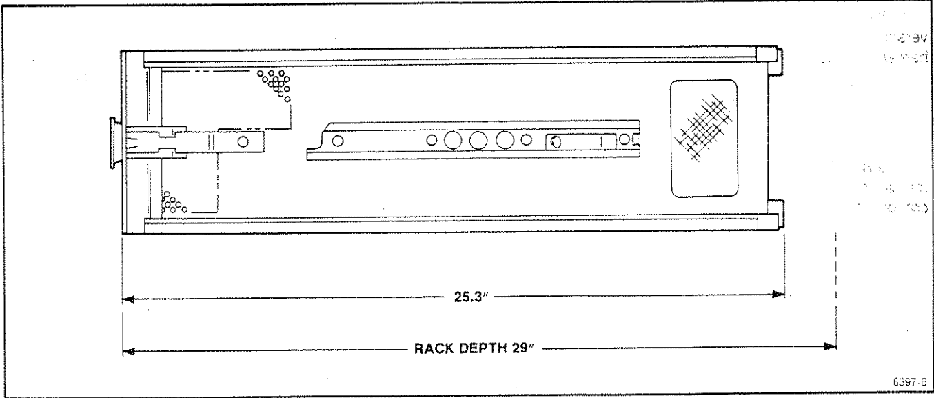
Fig. D-11. Instrument rackmounting length and clearance.
