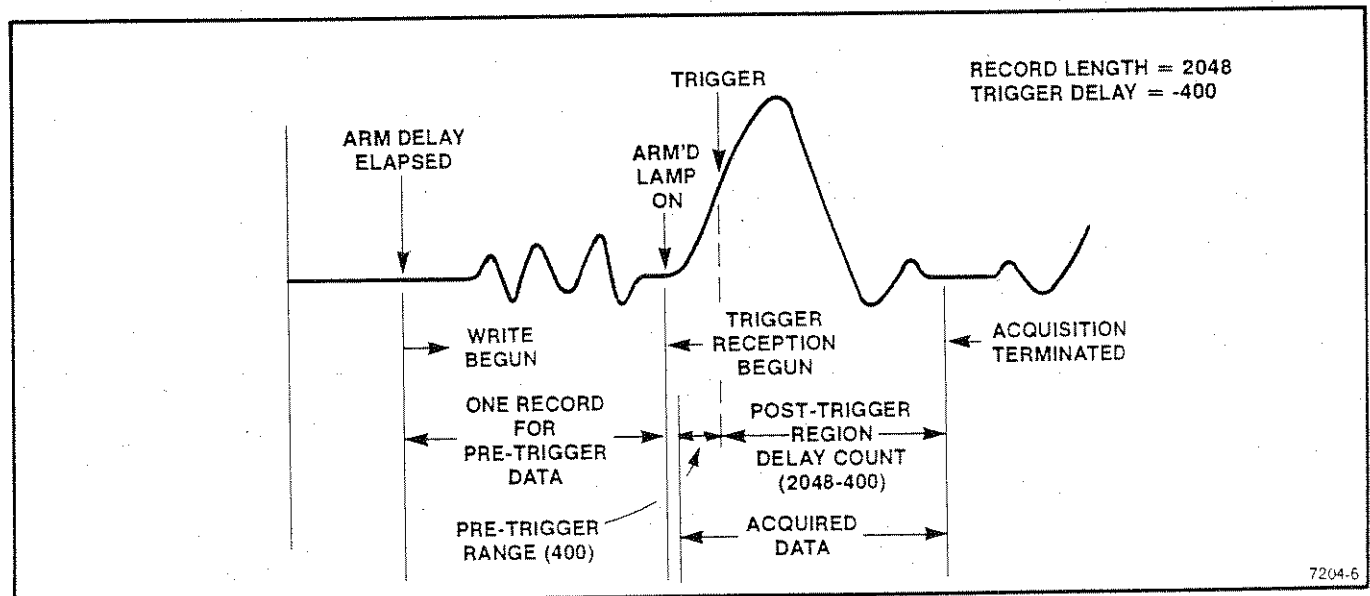
Fig. 3-22. Pre-trigger operation.
