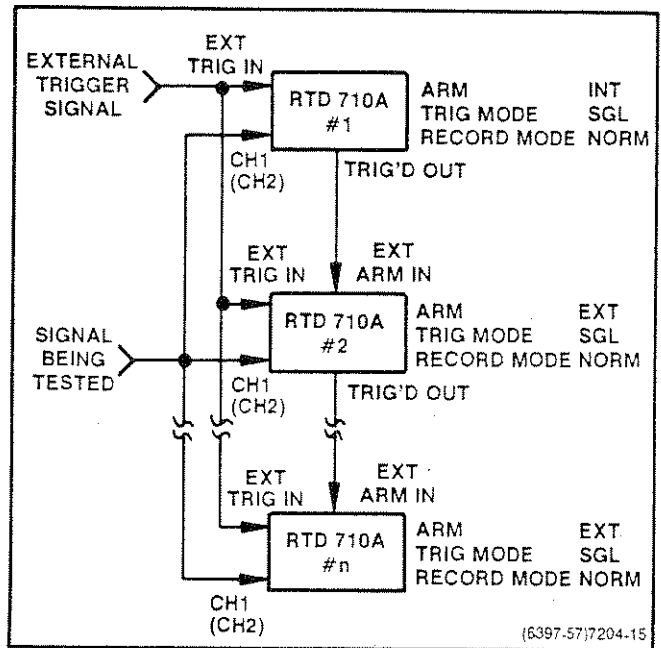
Fig. 3-45. Serially connected RTD 710As.
