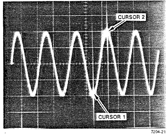
Fig. 3-52. Amplitude measurement with CURSOR 1 and 2.
