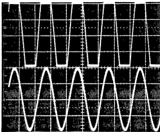
Fig. 3-13. Overrange display.
