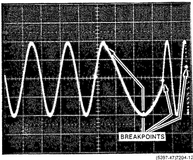
Fig. 3-34. Breakpoint waveform with pre-trigger.
