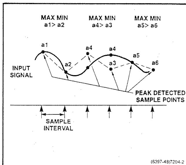
Fig. 3-36. Envelope peak detection.
