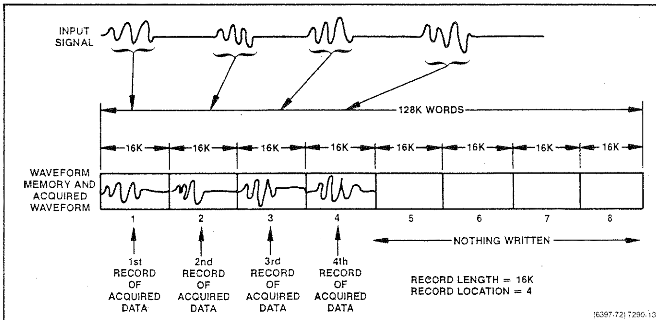
Fig. 3-35. Auto-advance representation.
