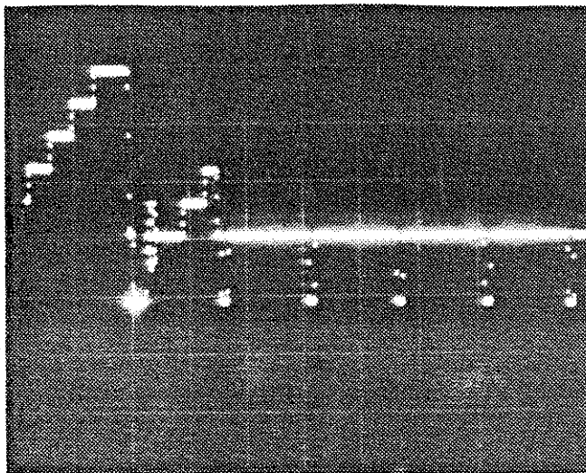
Fig. 6-3 Horizontal sync pulse display.
