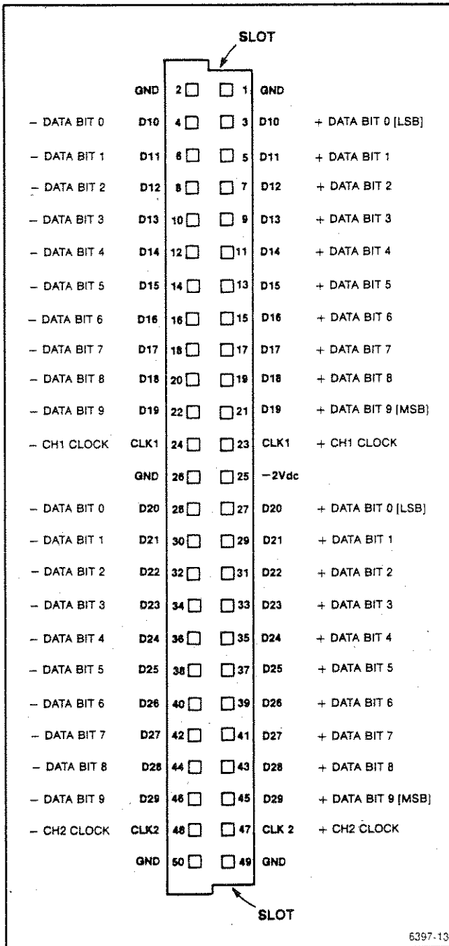
Fig. 4-3 Direct A/D output port connector.
