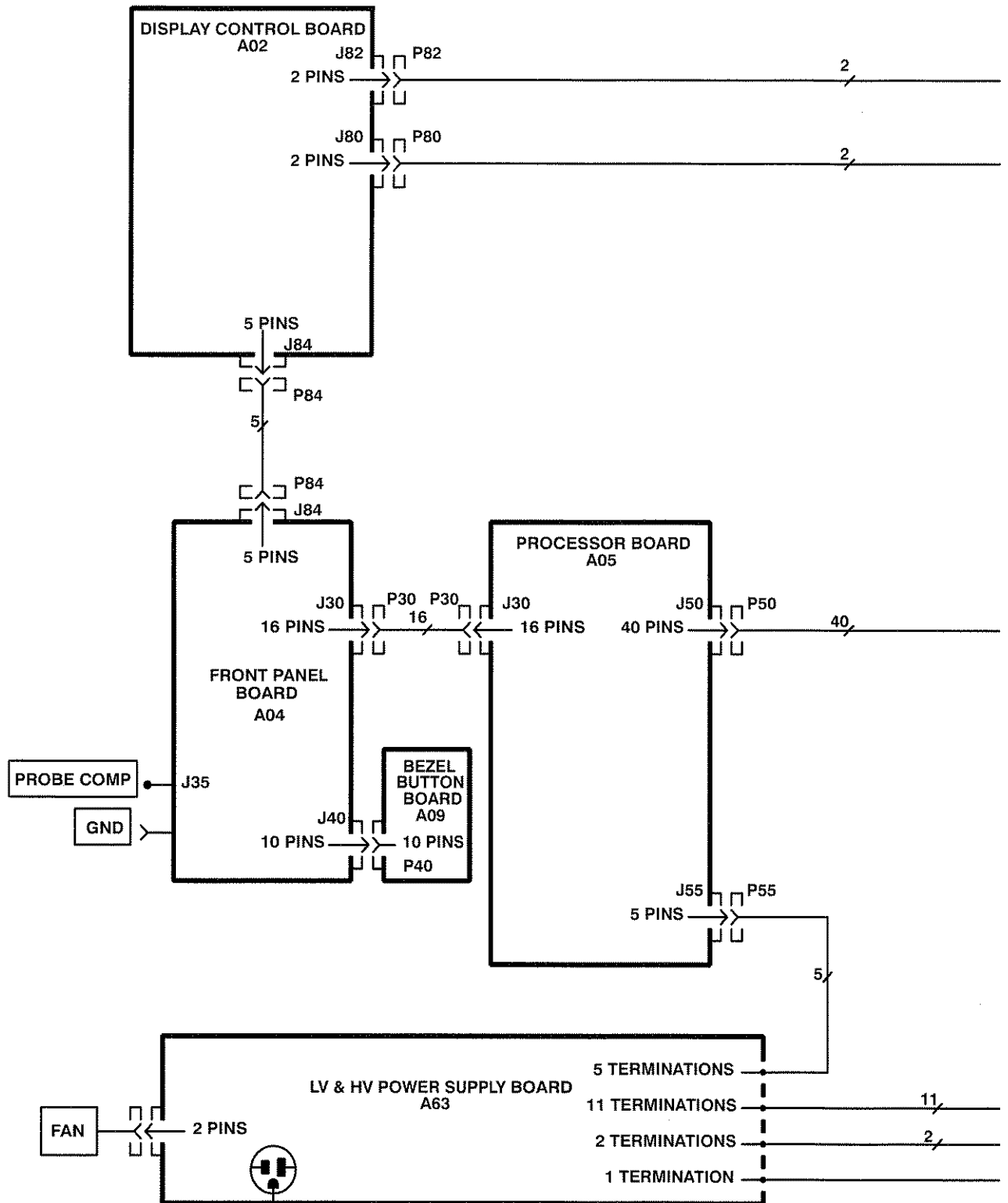
Figure 5-2: Block Diagram (B020100 and Above)
