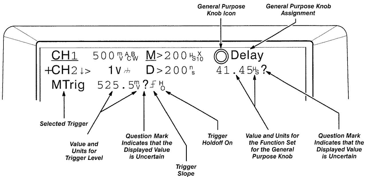
Figure 3-4: Readout Indicators
