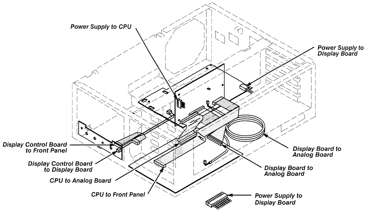
Figure 8-4: Cables and Cable Routing
