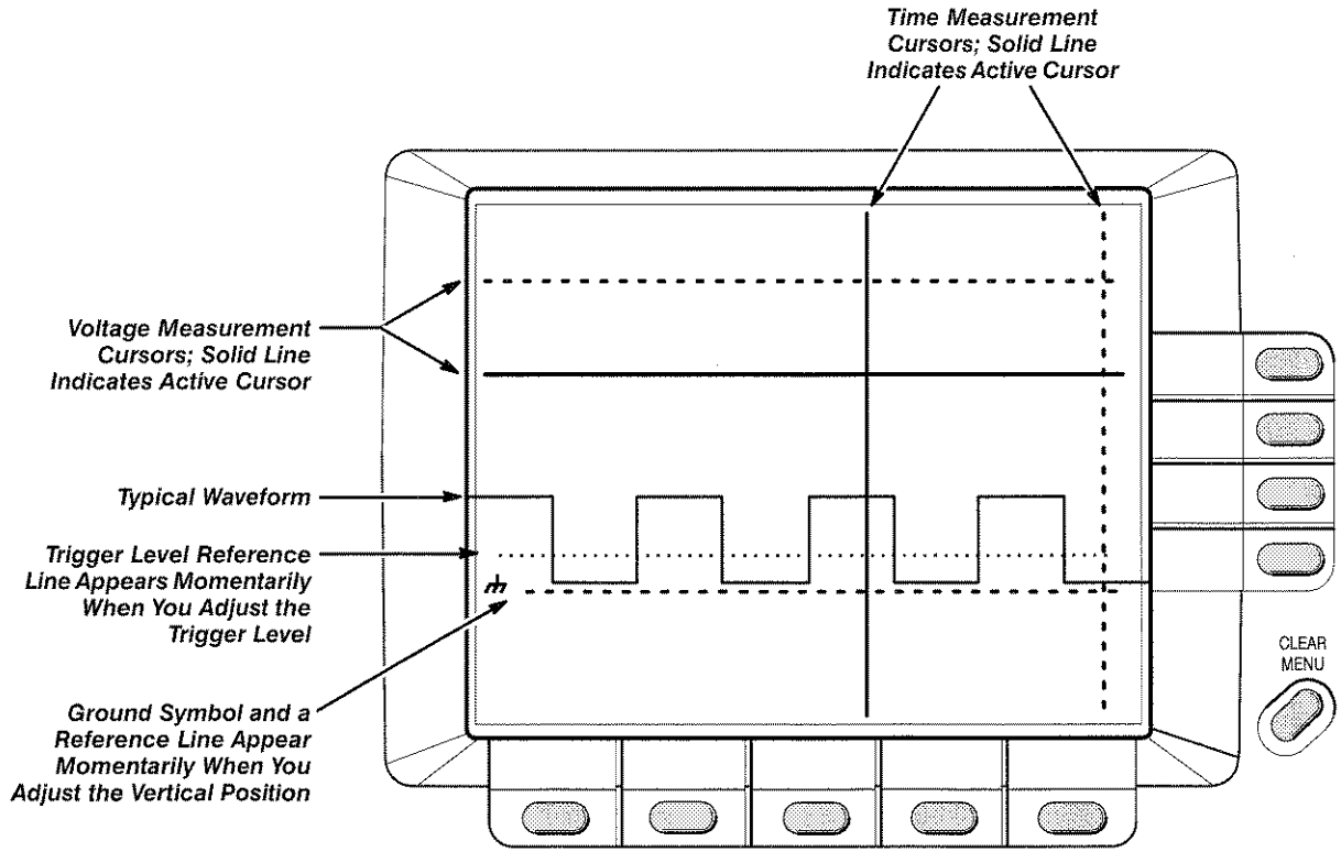
Figure 3-5: Waveform References
