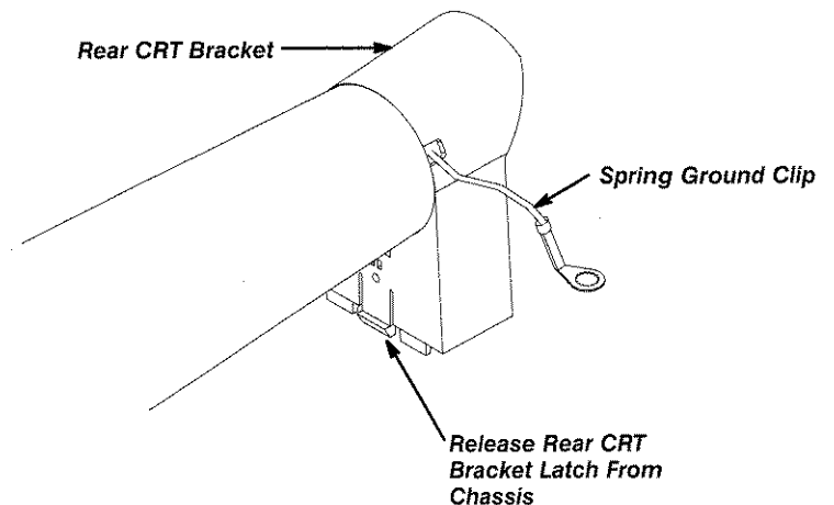
Figure 8-15: CRT Rear Bracket and Ground Clip
