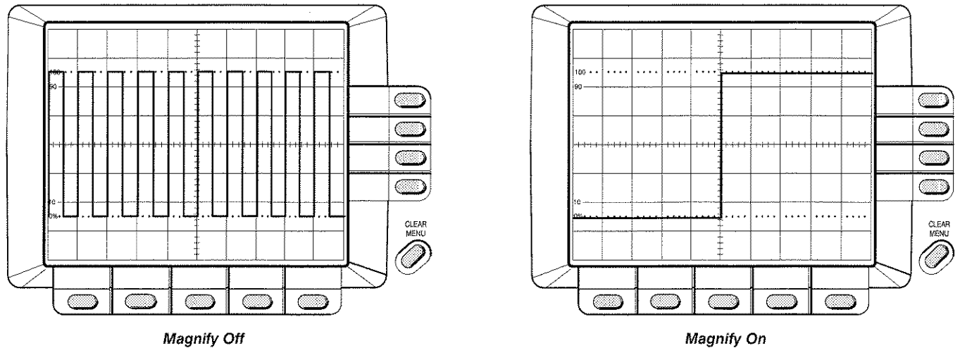
Figure 3-6: Horizontal Magnification
