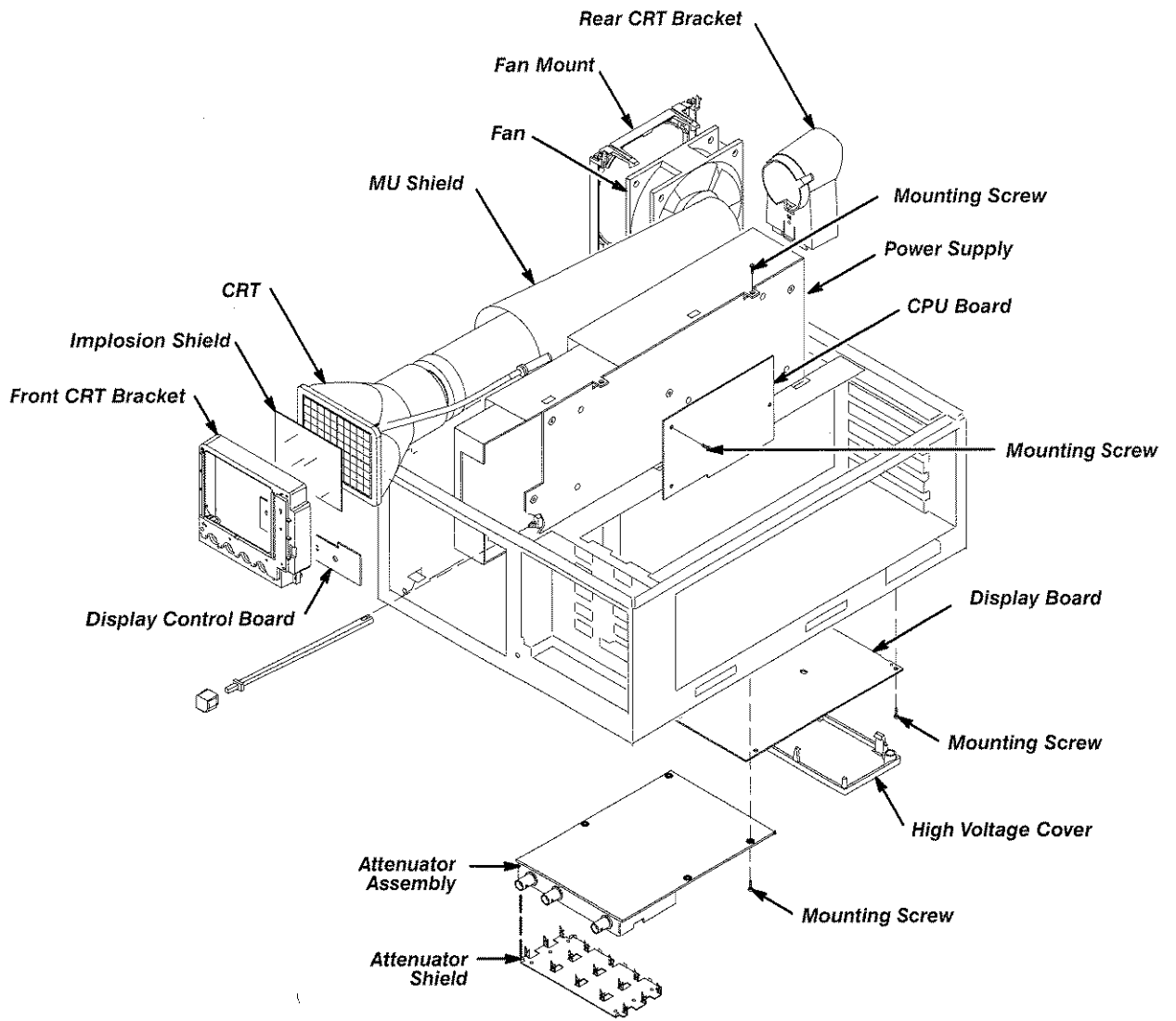
Figure 8-3: Internal Modules
