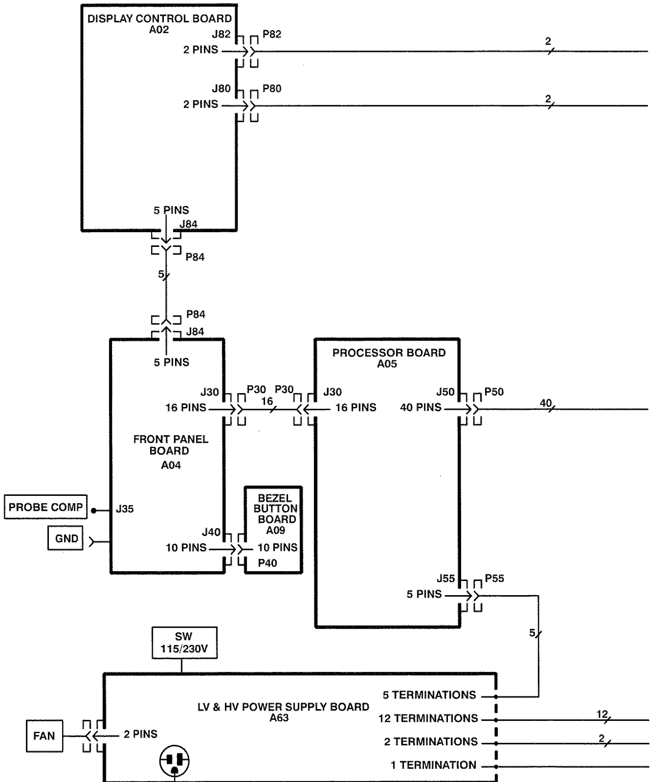
Figure 5-1: Block Diagram (B020099 and Below)
