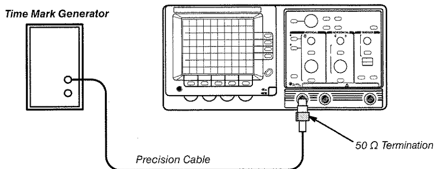
Figure 7-2: CRT Adjustments Calibration Setup
