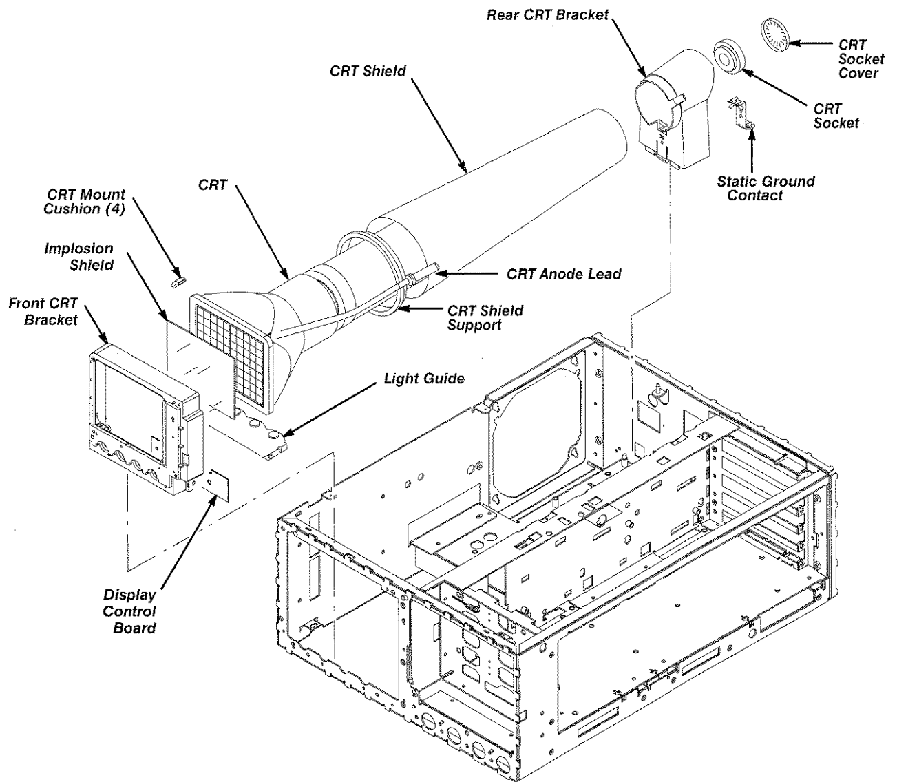
Figure 8-16: CRT Removal
