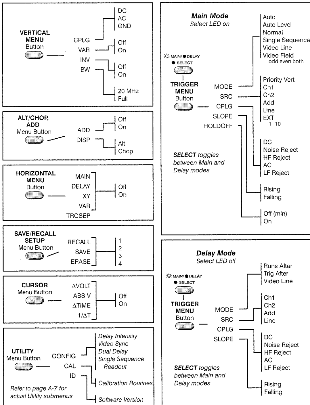
Figure 3-2: Menu Map
