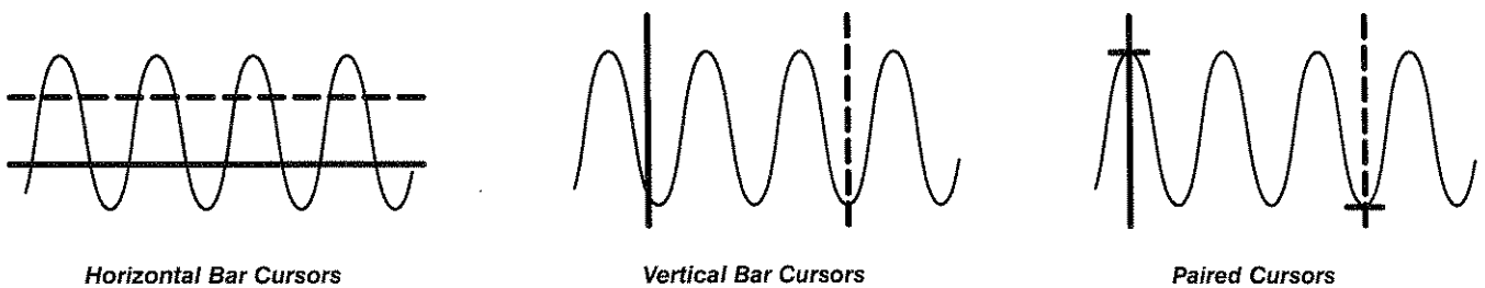
Figure 3-4: Cursor Types
