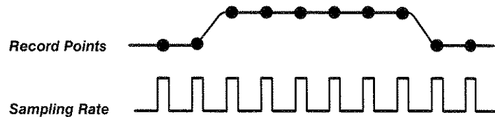
Figure 2-7: Real-Time Sampling
