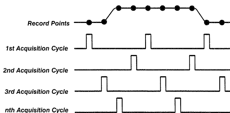
Figure 2-8: Equivalent-Time Sampling
