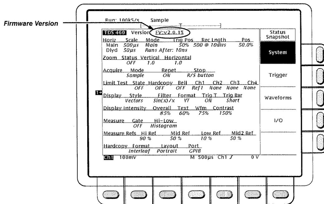
Figure 3-52: Status Menu—System
