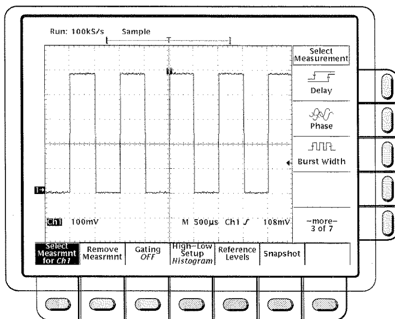
Figure 3-27: Measure Menu
