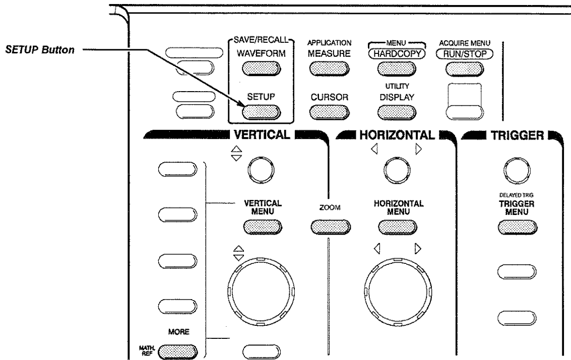
Figure 1-2: Menu Button Locations (Gray Buttons)
