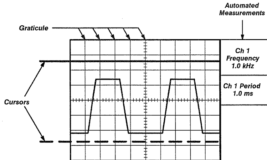
Figure 2-19: Graticule, Cursor and Automated Measurements
