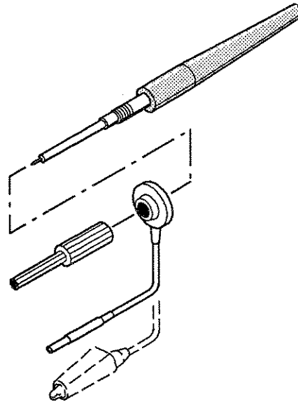
Figure 3-42: Long Ground Leads
