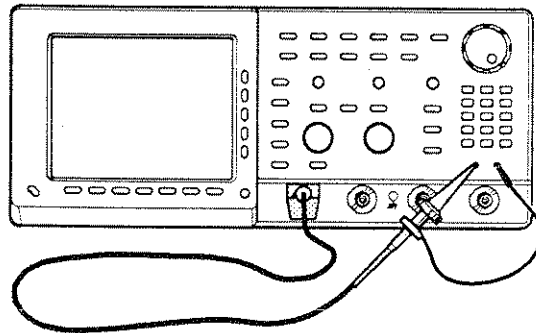
Figure A-21: Initial Test Hookup (TDS 520)
