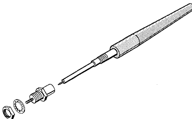
Figure 3-47: Probe-Tip-to-Chassis Adapter
