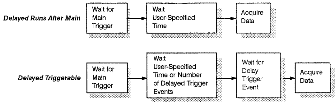
Figure 3-5: Delayed Triggering
