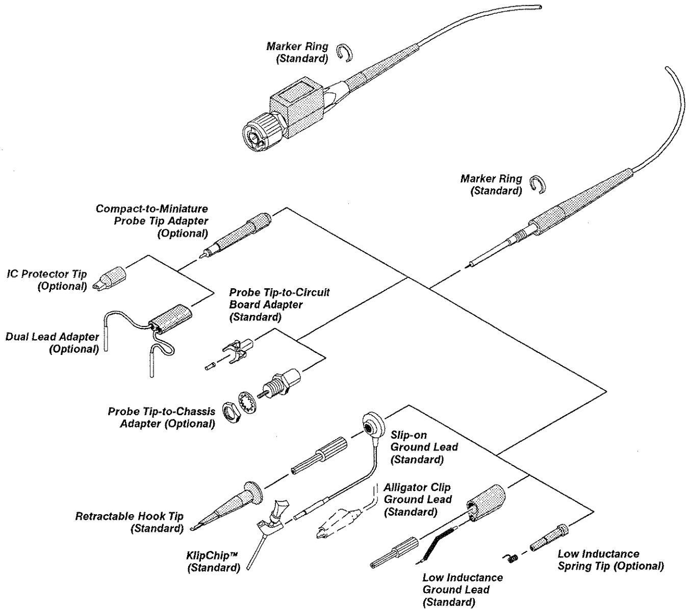
Figure 3-39: Probe Accessories
