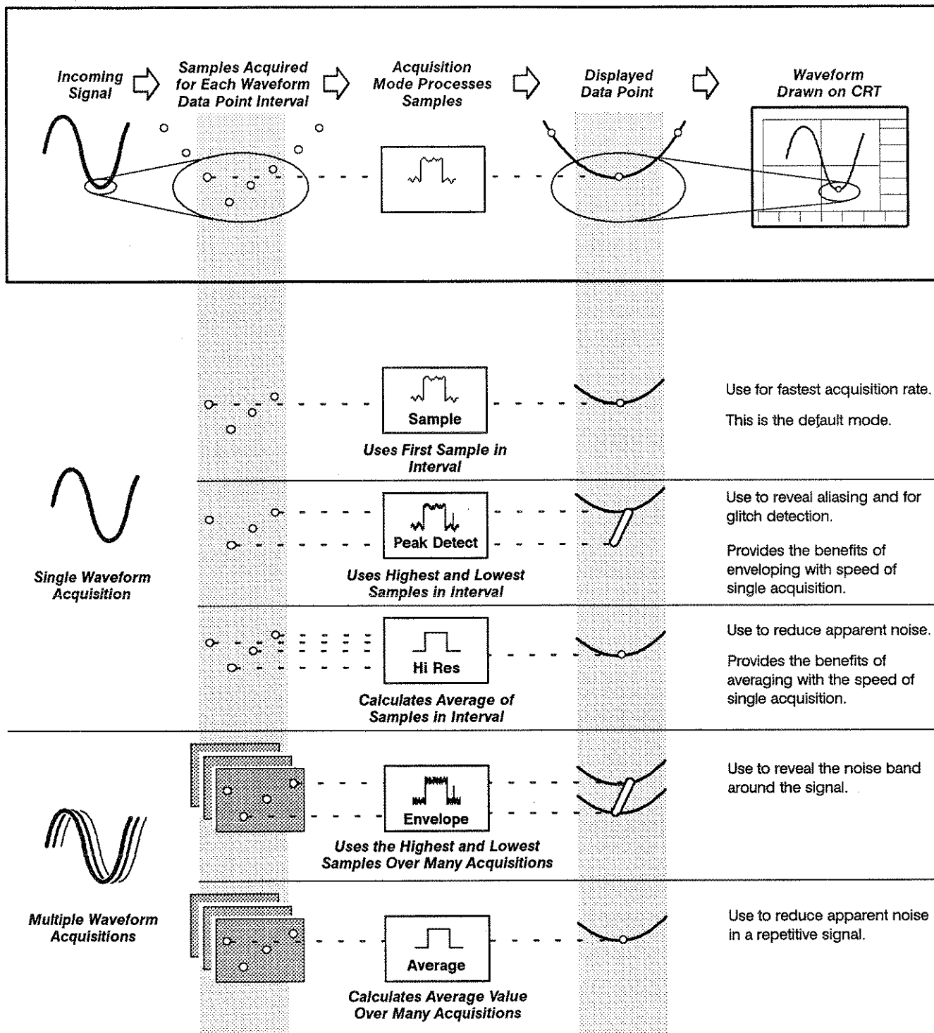
Figure 2-18: How the Acquisition Modes Work
