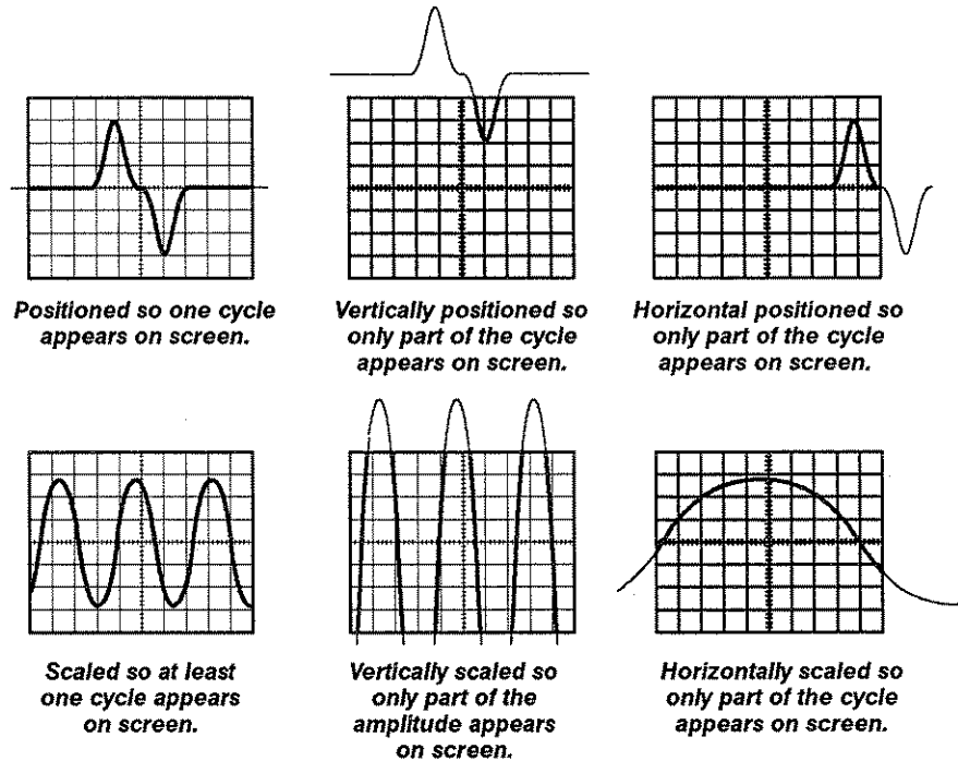
Figure 2-12: Proper and Improper Scaling and Positioning
