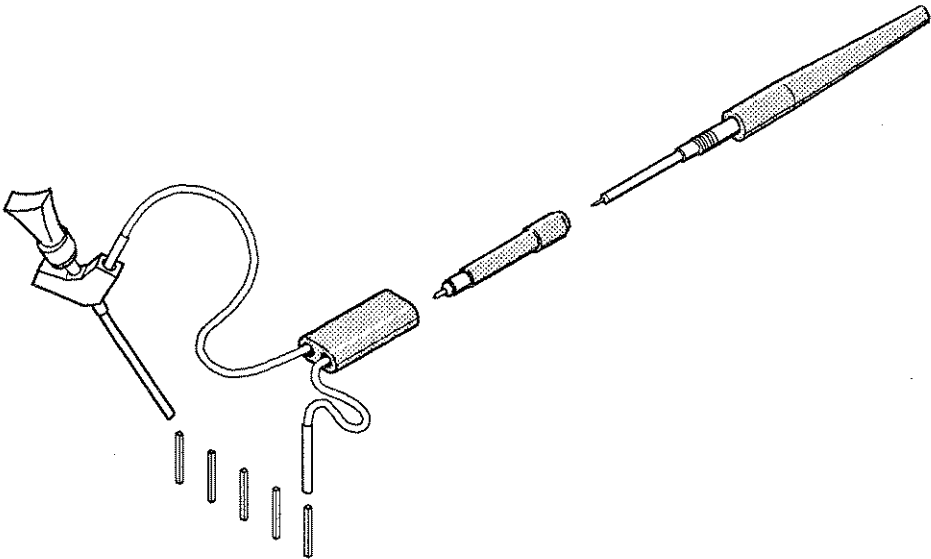
Figure 3-50: Dual-Lead Adapter
