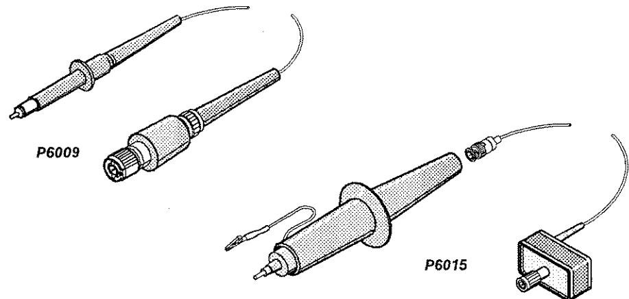
Figure 3-52: The P6009 and P6015 High Voltage Probes
