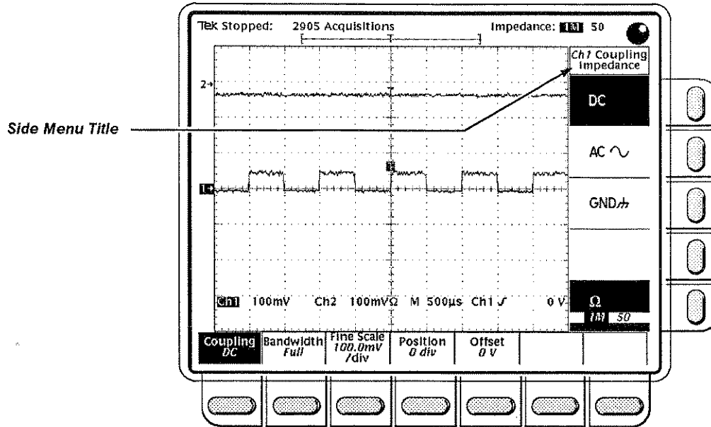
Figure 1-11: The Menu After Changing Channels
