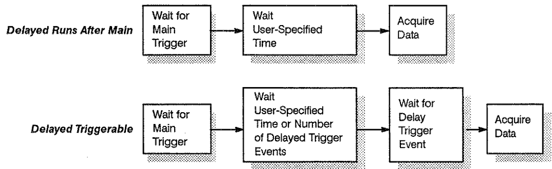
Figure 2-9: Delayed Triggering
