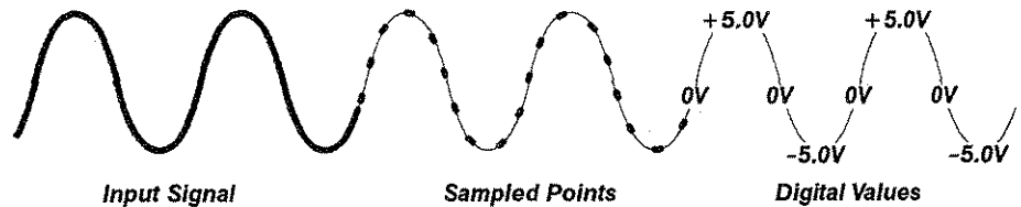
Figure 2-14: Acquisition: Input Analog Signal, Sample, and Digitize
