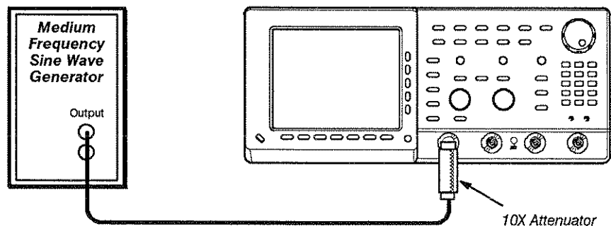
Figure A-14: Initial Test Hookup
