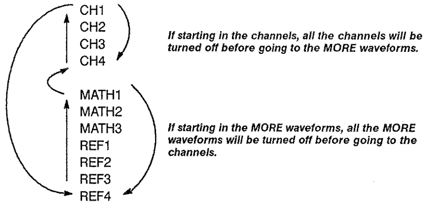
Figure 3-62: Waveform Selection Priority (TDS 540)
