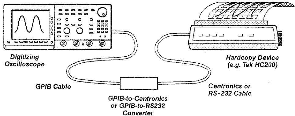
Figure 3-19: Connecting the TDS and Hardcopy Device Via a Converter
