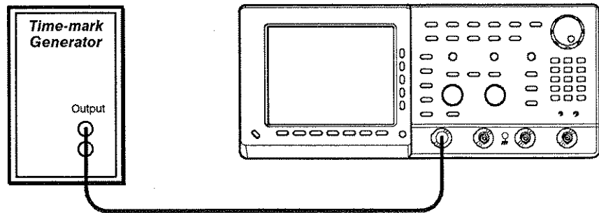
Figure A-12: Initial Test Hookup
