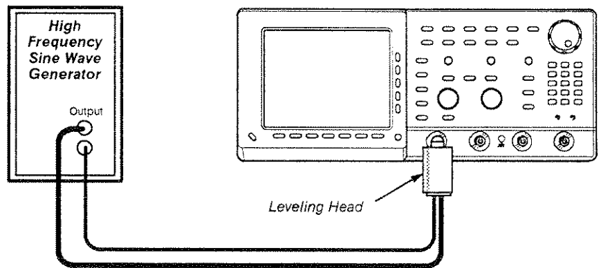
Figure A-8: Initial Test Hookup
