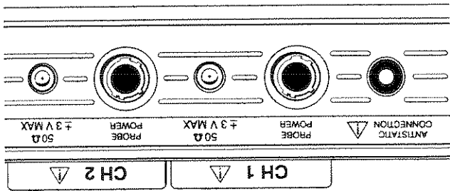
Figure 3-40: The Probe Interface Connectors
