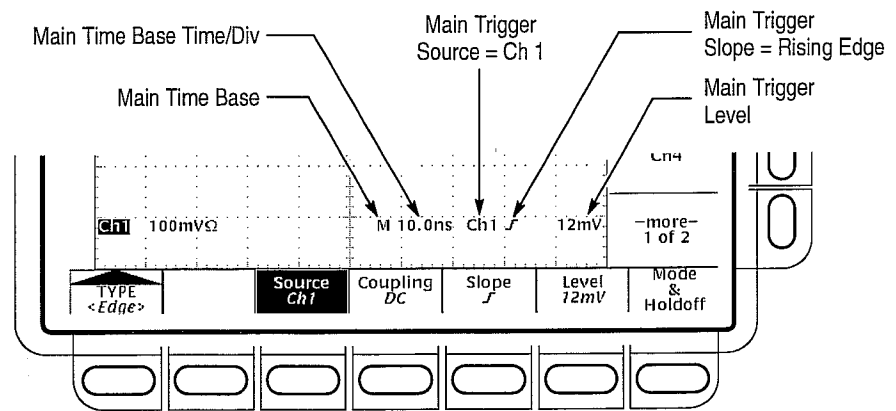
Figure 3–40: Example Trigger Readouts — Edge Trigger Selected
