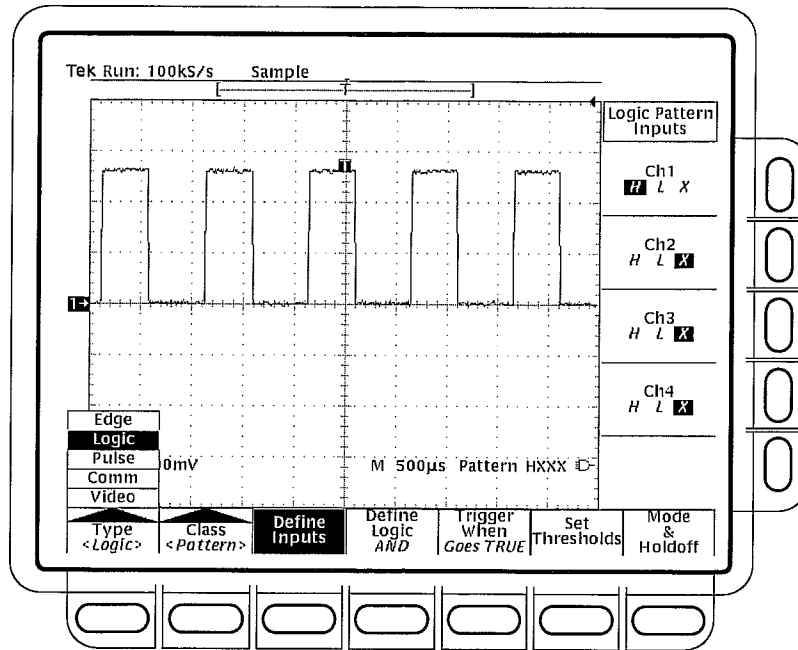
Figure 3–46: Logic Trigger Menu
