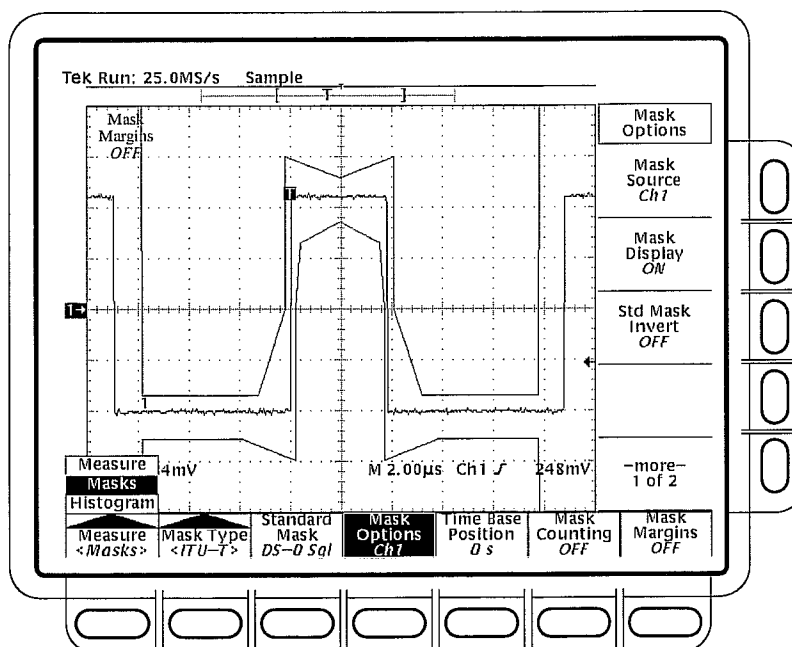
Figure 3–70: Mask menu
