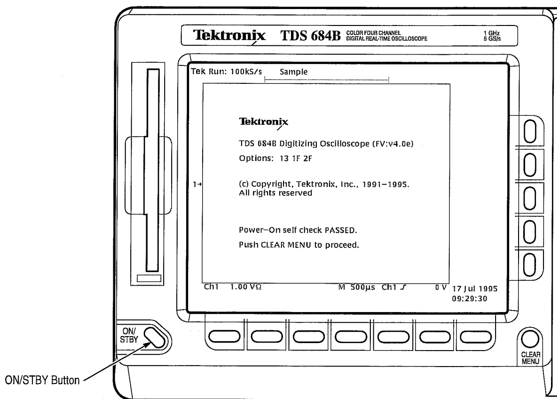
Figure 1-2: ON/STBY Button
