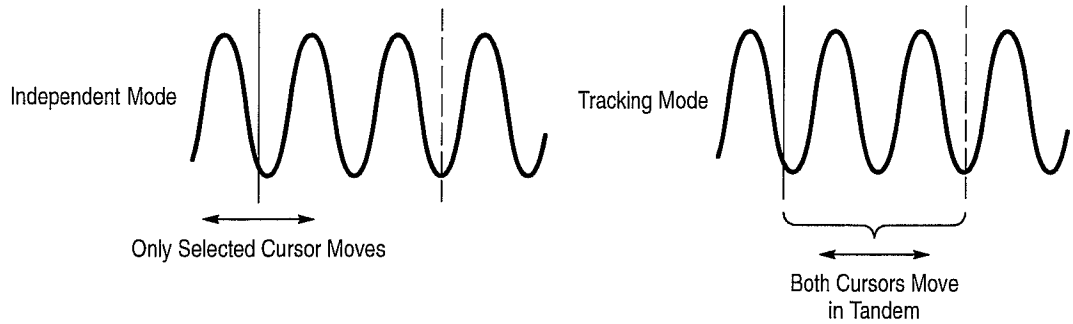
Figure 3-66: Cursor Modes
