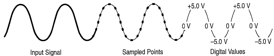
Figure 3–11: Acquisition: Input Analog Signal, Sample, and Digitize
