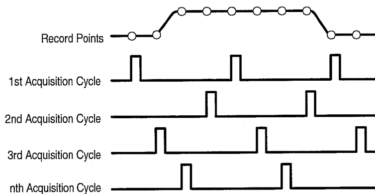
Figure 3–14: Equivalent-Time Sampling
