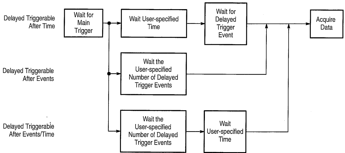
Figure 3–55: Delayed Triggerable
