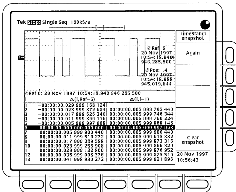
Figure 3-34: Horizontal Menu — FastFrame Snapshot
