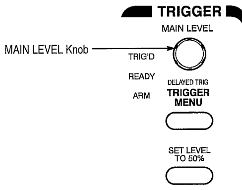
Figure 2–7: TRIGGER Controls
