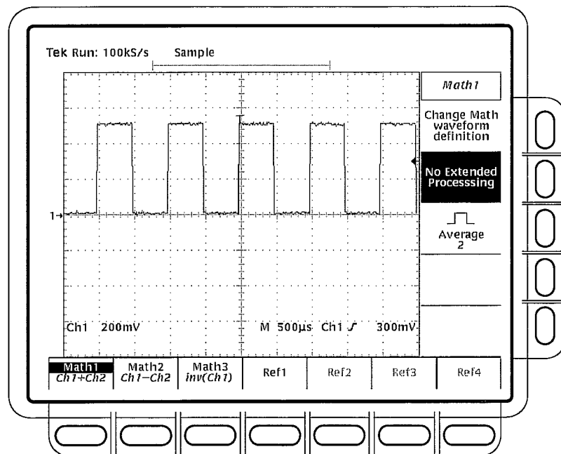
Figure 3-77: More Menu
