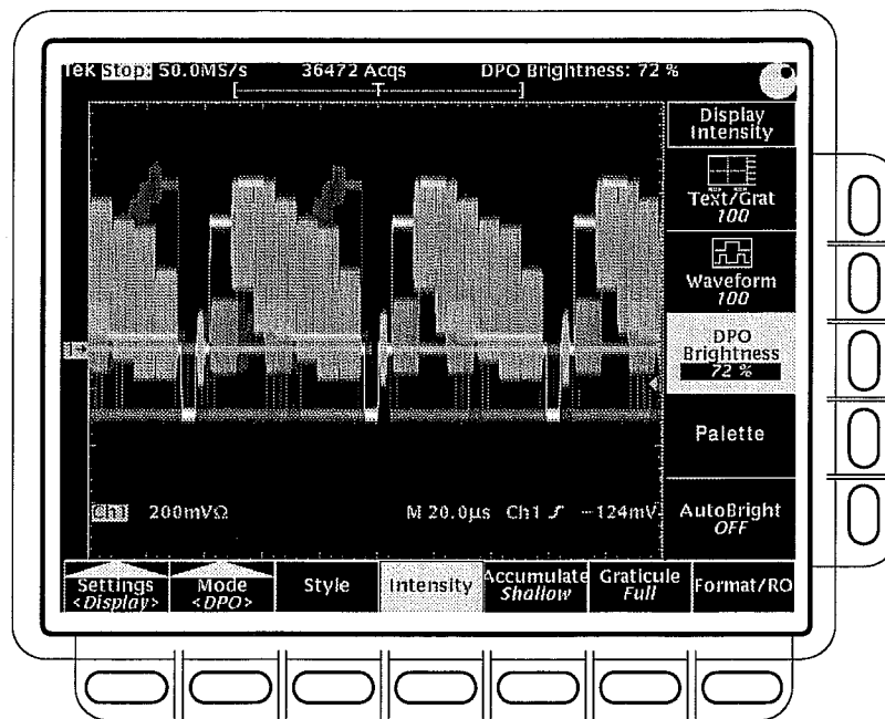
Figure 3–29: DPO Display
