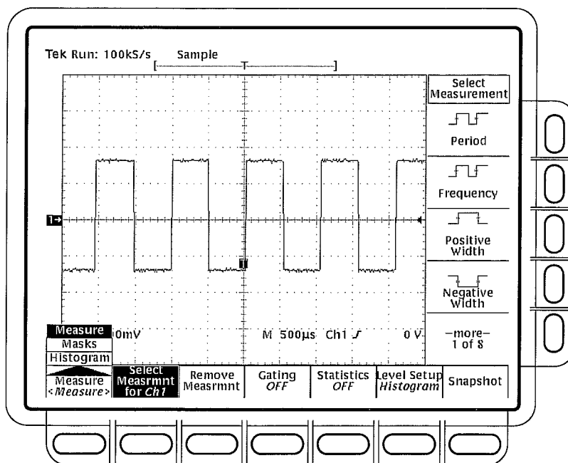
Figure 3–60: Measure Menu
