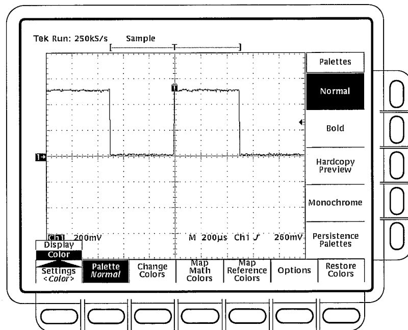
Figure 3–21: Display Menu — Setting
