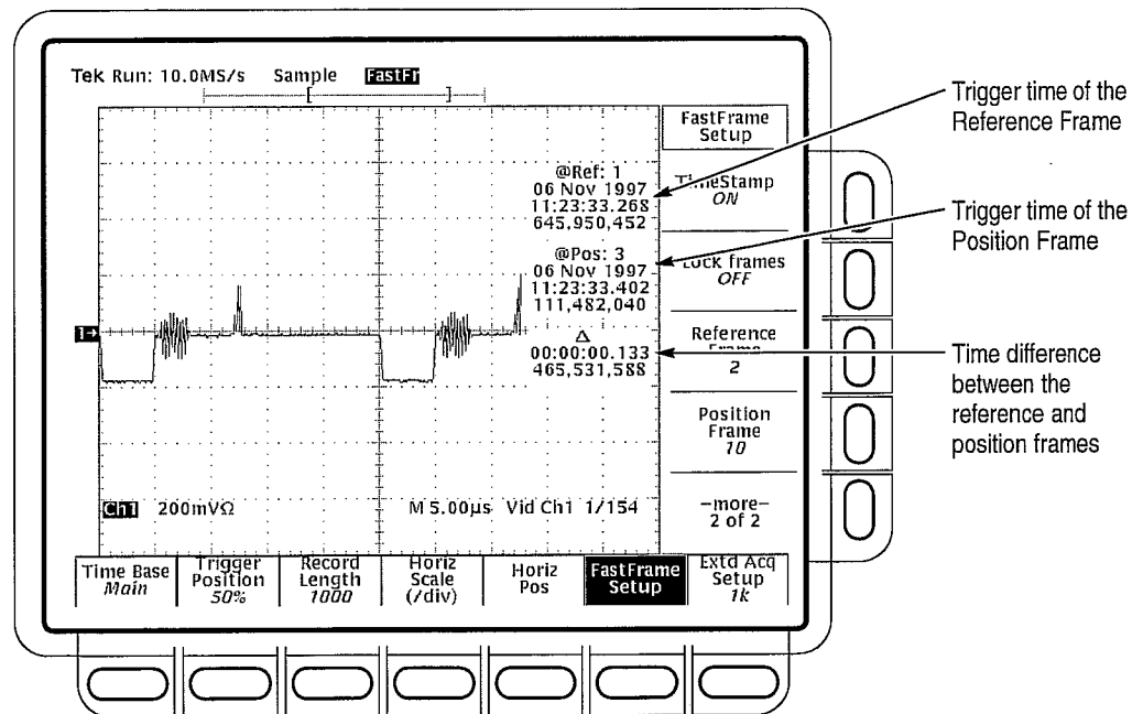
Figure 3–35: FastFrame TimeStamp
