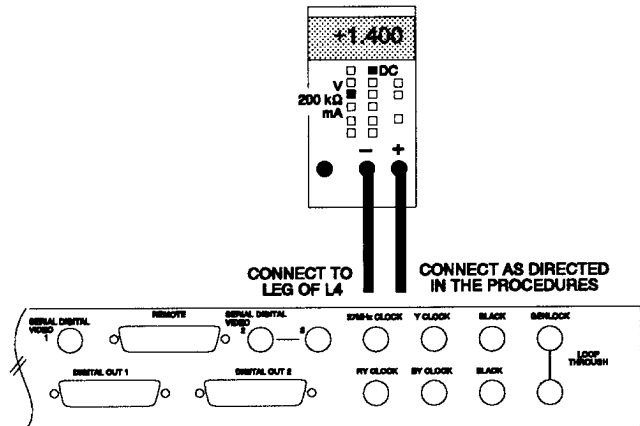
Fig. A-11. Setup to adjust the Serial Digital Video Output Amplitude.
