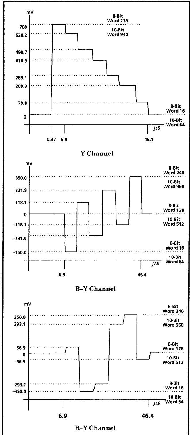
Fig. 3-9. 100% Color Bars.
