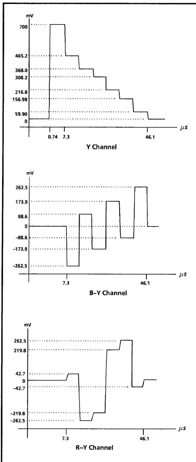
Fig. 3-17. 75% Bars (50 Hz).
