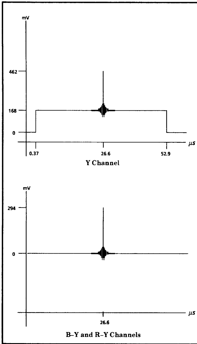
Fig. 3-46. SIN X/\chi .
