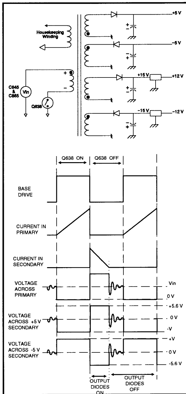
Fig. 6-20. Basic operation of T440.
