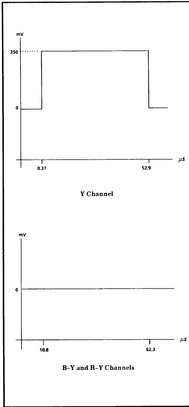
Fig. 3-40. Flat Field.
