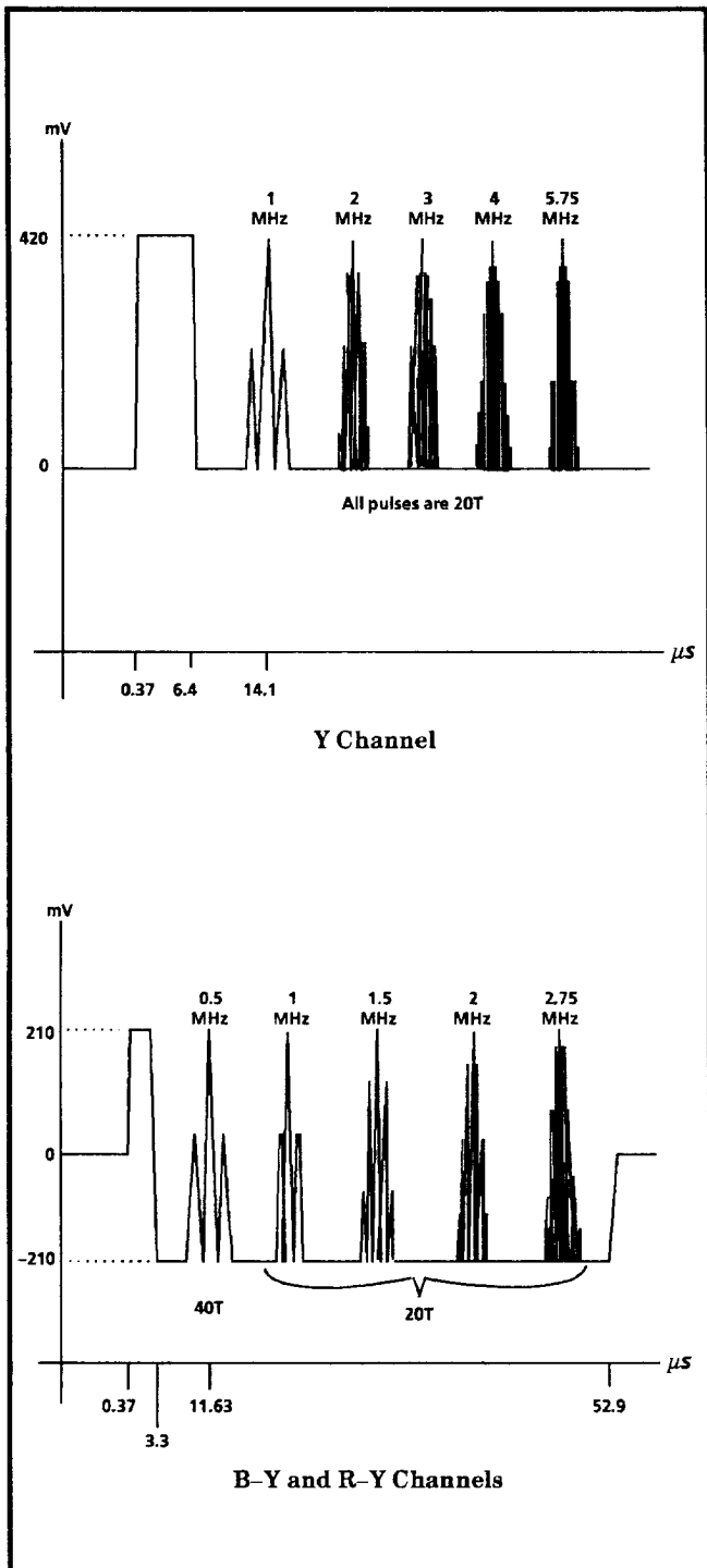
Fig. 3-31. Multipulse.
