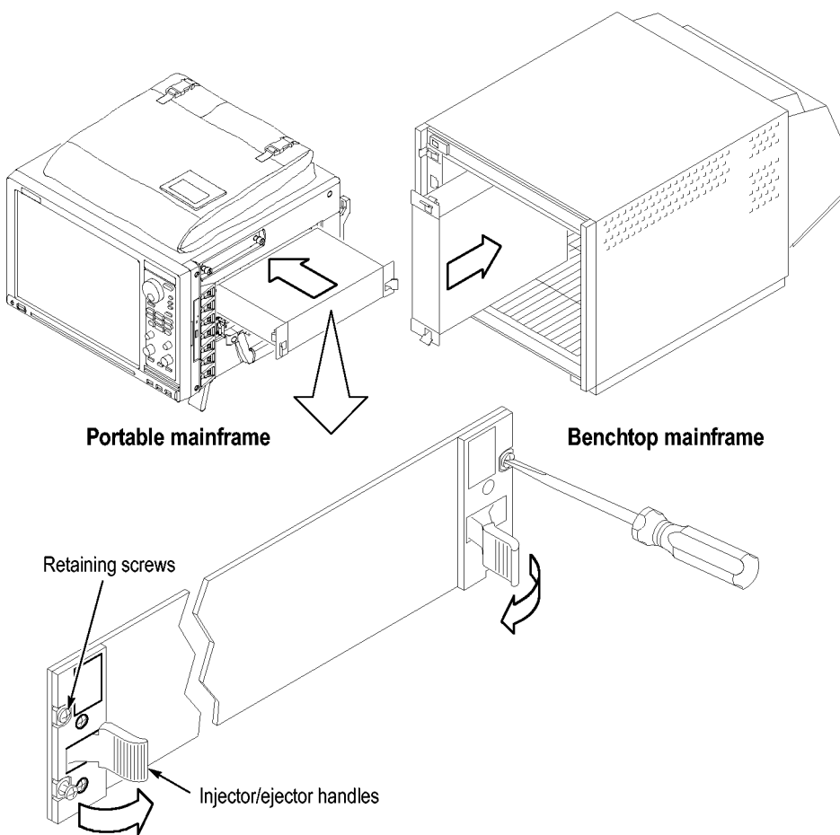
Figure 4: Installing modules
