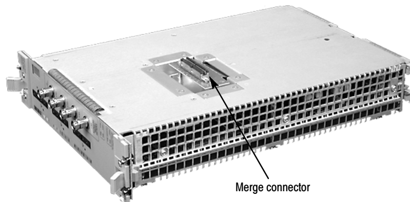
Figure 2- 4: Merge connector on a TLA7Axx (shown in the extended position)
