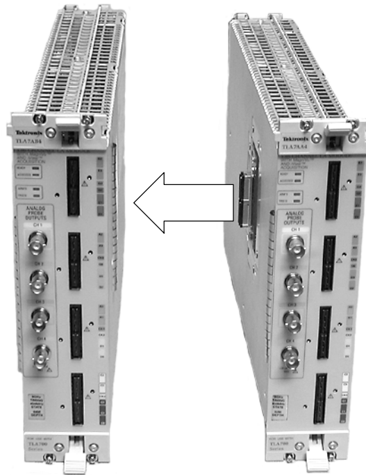
Figure 2-8: Connecting the logic analyzer modules together
