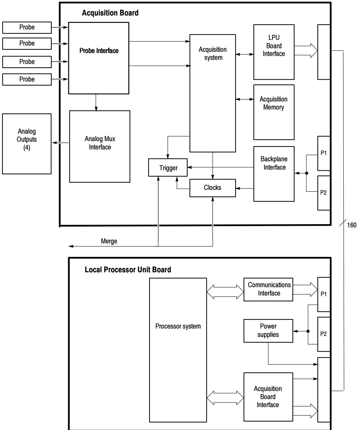
Figure 9- 1: TLA7AAX logic analyzer block diagram
