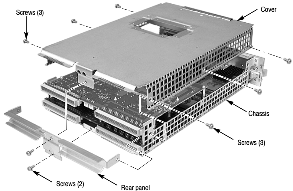
Figure 6-7: Cover removal
