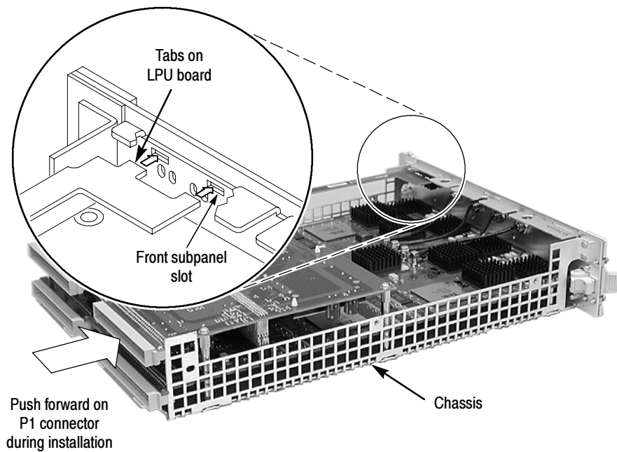
Figure 6- 11: Inserting LPU board tabs into front subpanel
