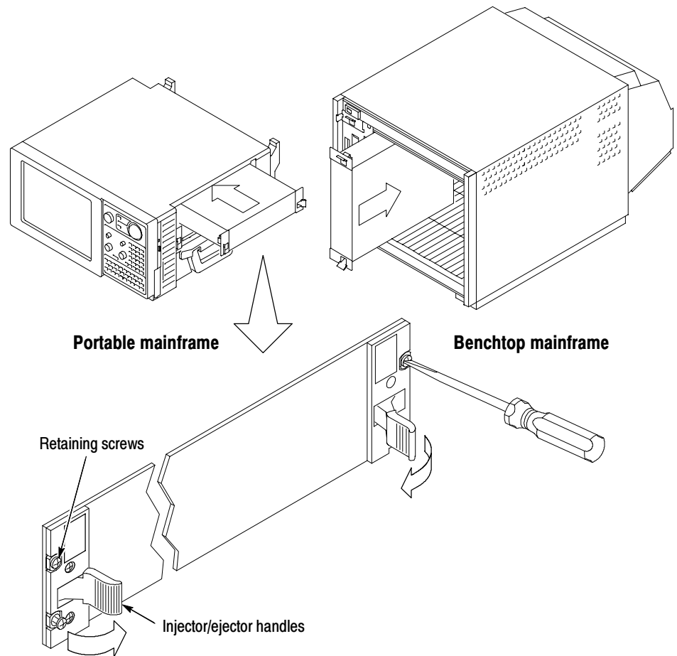
Figure 2-2: Installing modules in the mainframe
