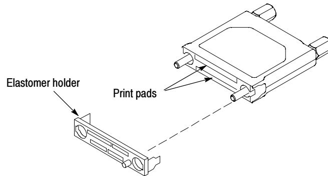
Figure 6-1: Cleaning the probe heads
