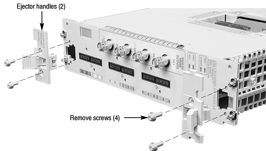
Figure 6-5: Injector/ejector handle replacement
