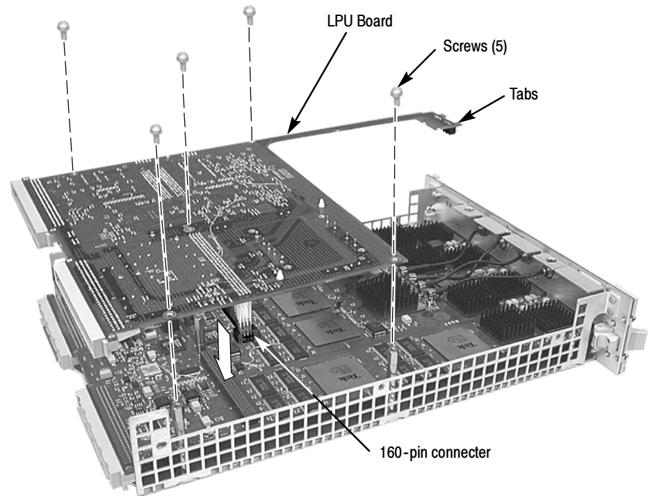
Figure 6-10: LPU board removal
