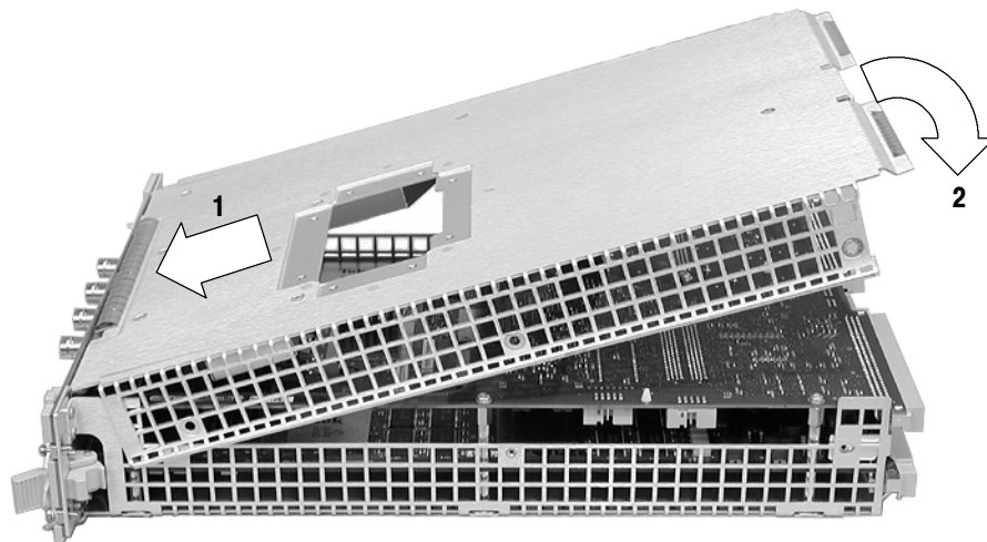
Figure 6-8: Installing the cover onto the chassis
