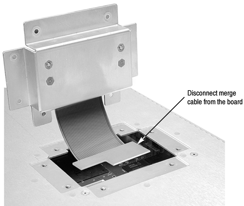
Figure 6-6: Removing the merge cable bracket from the cover
