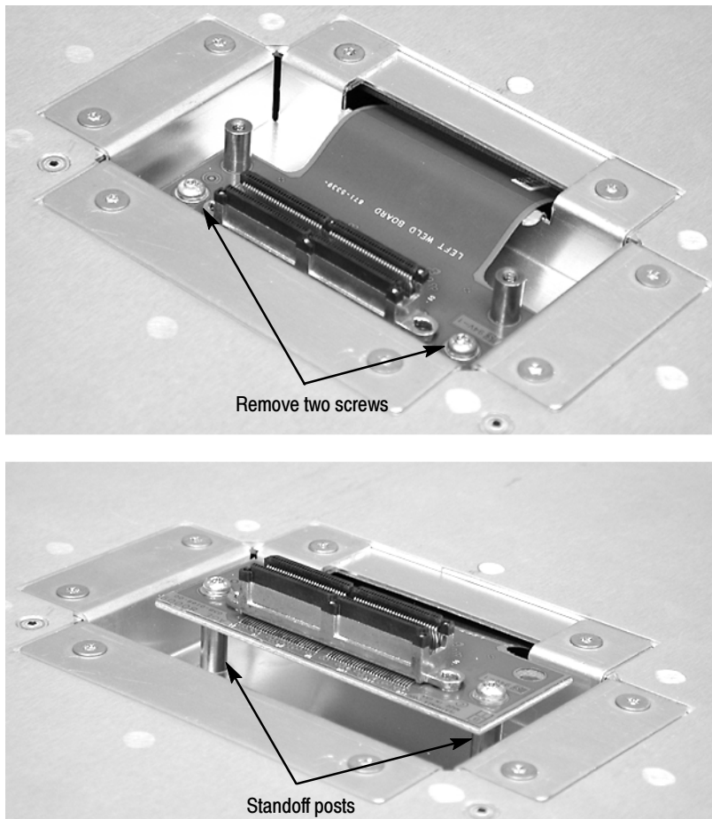
Figure 2-7: Removing the merge connector assembly from the module
