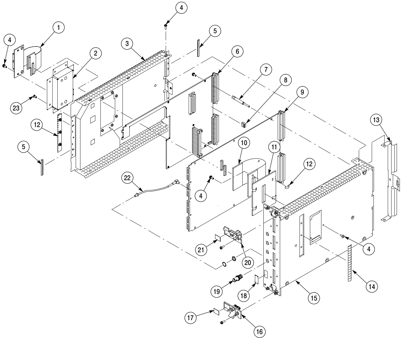
Figure 10- 1: TLA7AAX, TLA7ABX, and TLA7NAX Logic Analyzer Module exploded view
