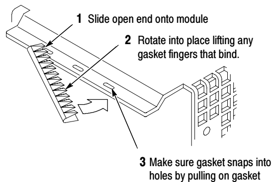
Figure 6- 16: Rear EMI gasket replacement
