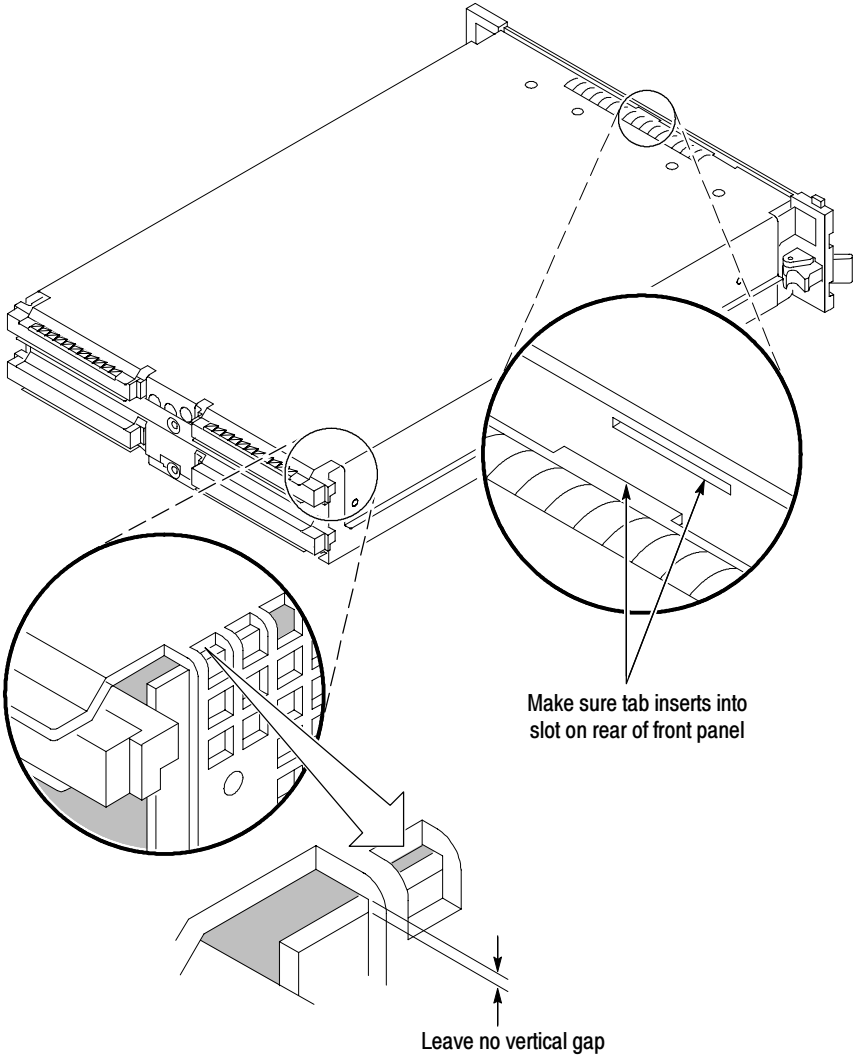
Figure 6-9: Seating the cover on the chassis
