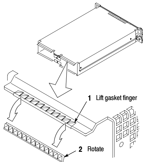
Figure 6-15: Rear EMI gasket removal
