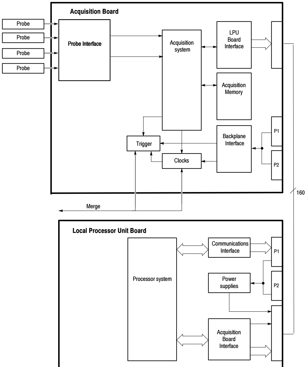
Figure 9-2: TLA7NAX logic analyzer block diagram
