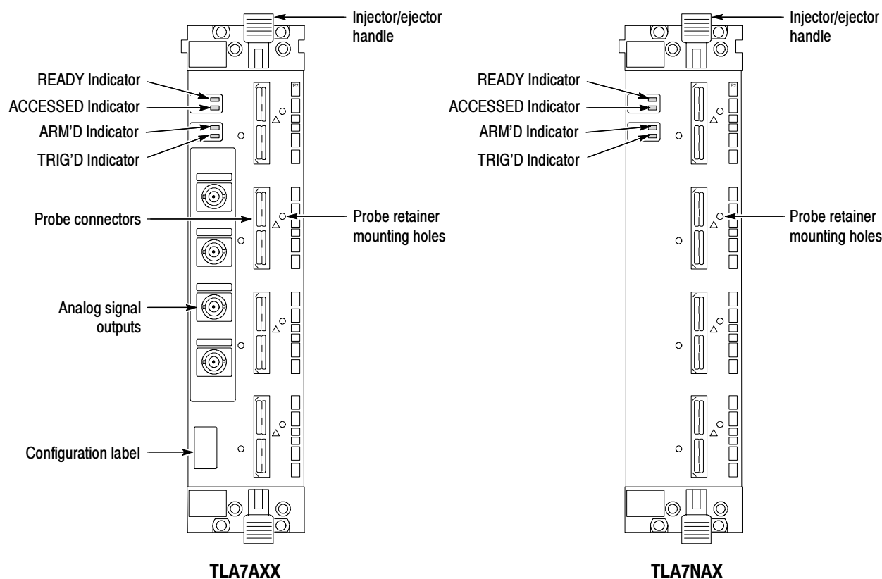
Figure 2-3: Front panel of the TLA7Axx and TLA7NAX logic analyzer module
