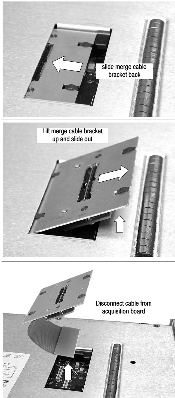
Figure 6- 13: Removing the merge cable assembly
