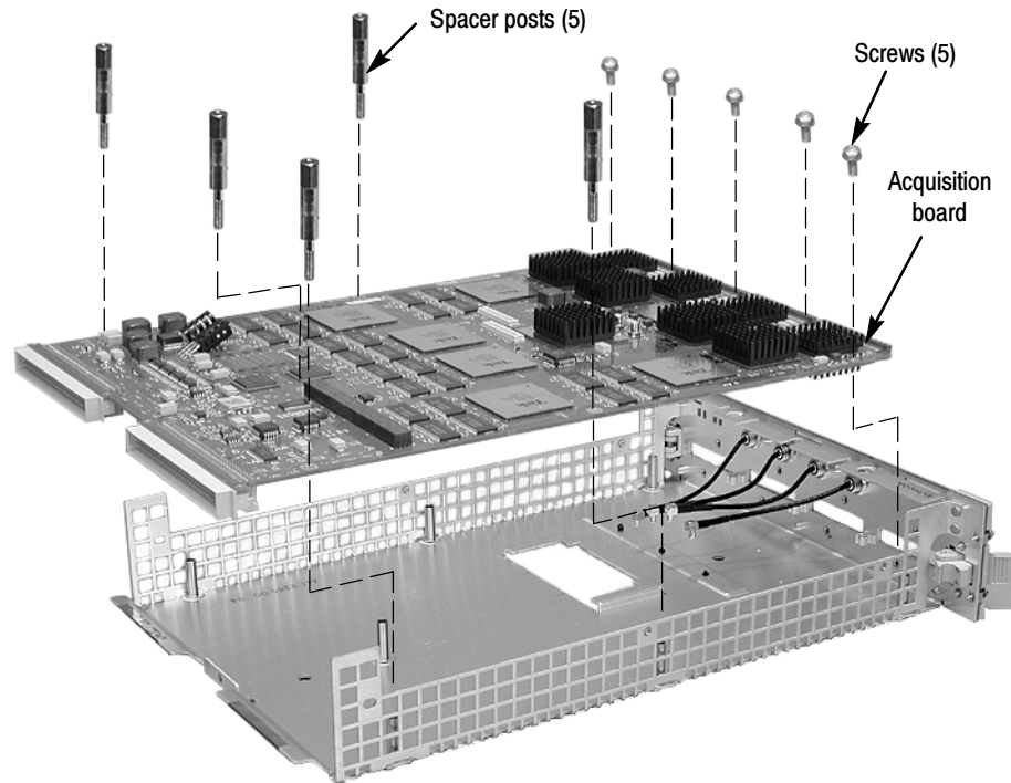
Figure 6-14: Removing the acquisition board from the chassis
