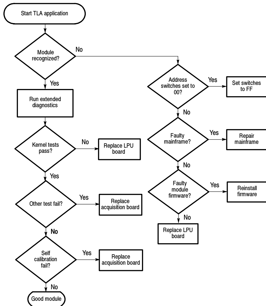
Figure 6- 17: Primary troubleshooting chart
