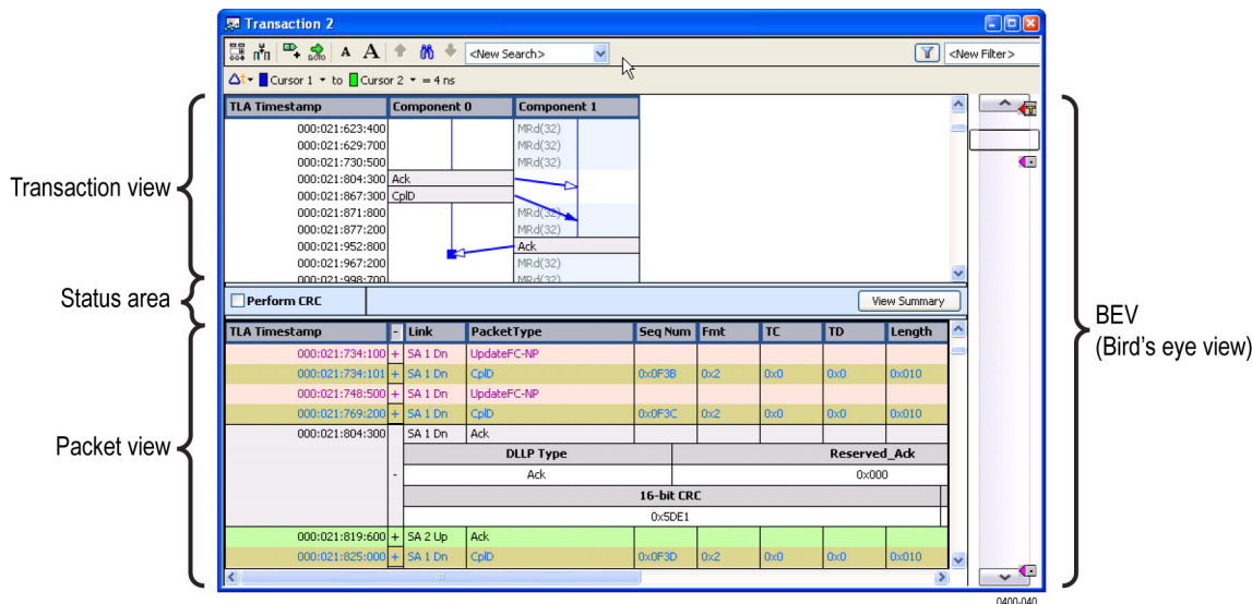
Figure 32: Transaction window
