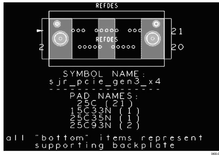
Figure 56: P67SA08 x4 midbus probe CAD symbol
