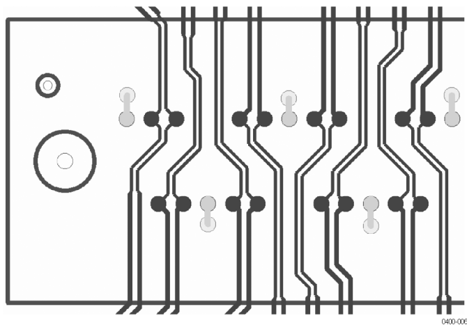
Figure 55: Recommended trace routing on the primary surface layer
