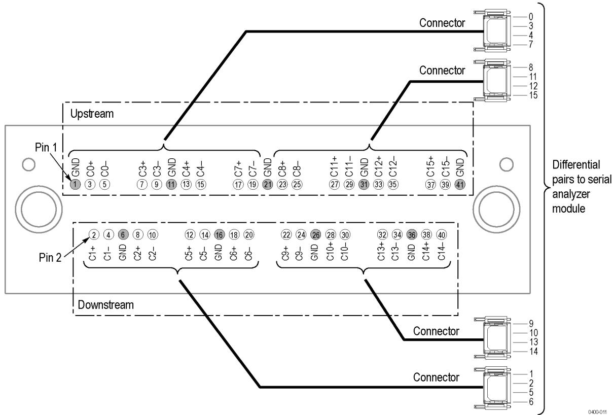
Figure 76: x8 midbus footprint connections in an upstream and downstream configuration
