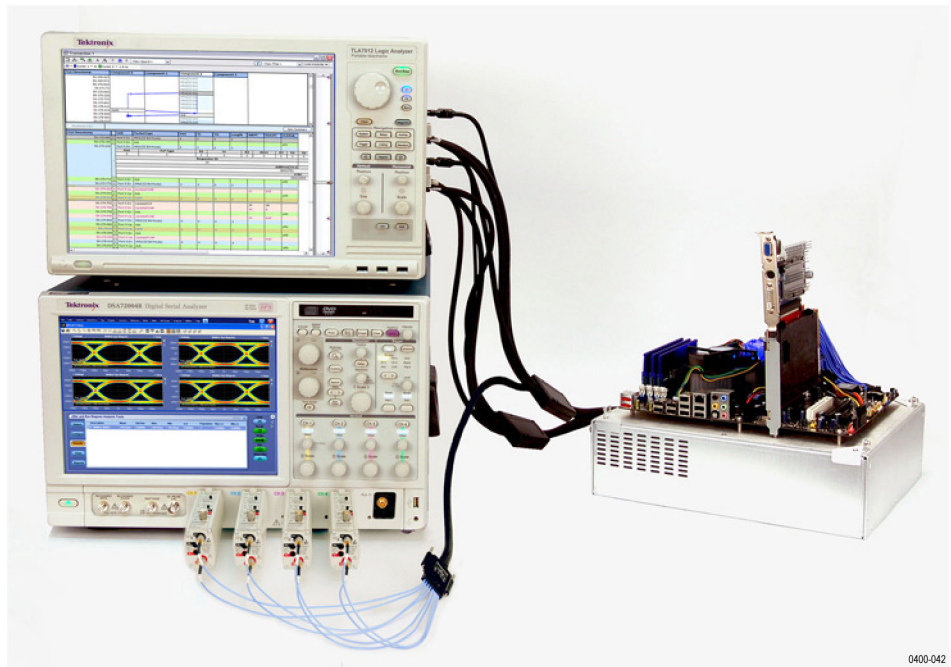
Figure 83: P67UHDSMA probe connected to the inputs of a Tektronix oscilloscope (example 1)
