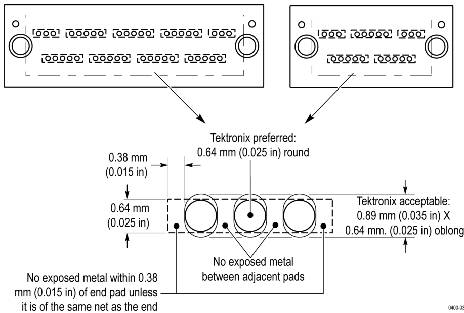
Figure 51: Footprint pad details for x8 and x4 midbus probes
