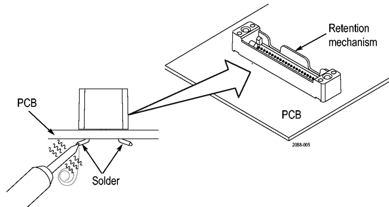
Figure 89: Soldering the anchoring posts to the circuit board (PCB)
