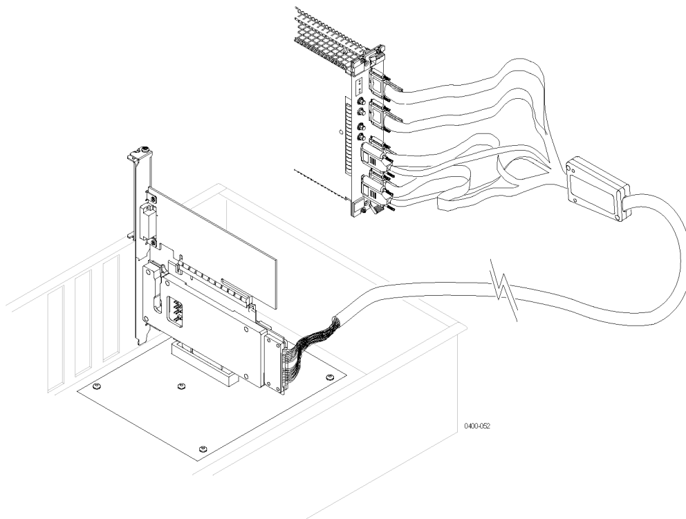
Figure 12: Connecting a slot interposer probe
