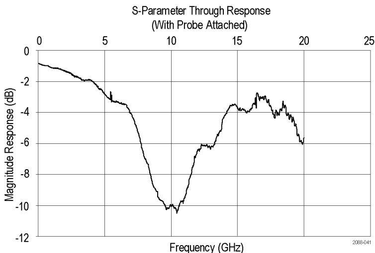
Figure 69: S-parameter data of retention mechanism plus P67SA16G2 x8 Midbus probe
