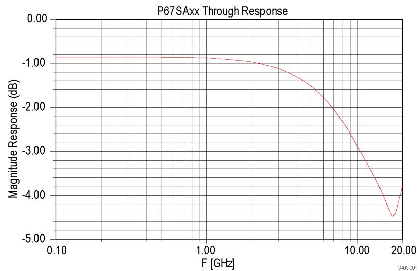
Figure 67: Probe impact of the P67SAxx midbus probe
