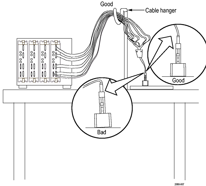
Figure 11: Arranging the midbus probe cables
