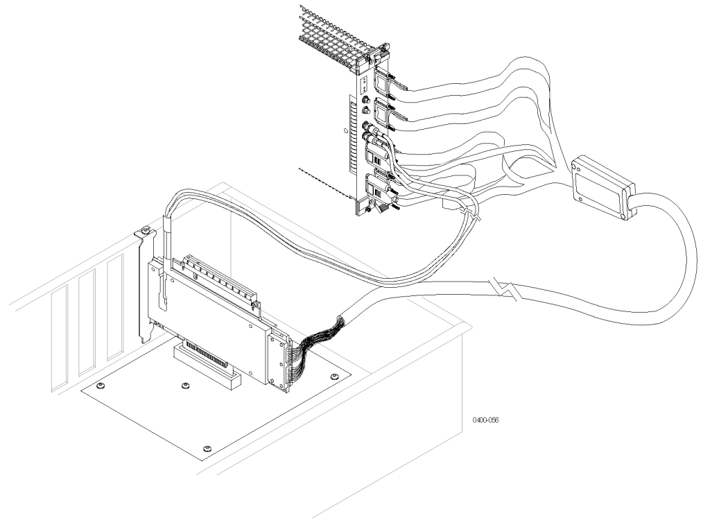
Figure 72: Slot interposer probe with a reference clock cable connected
