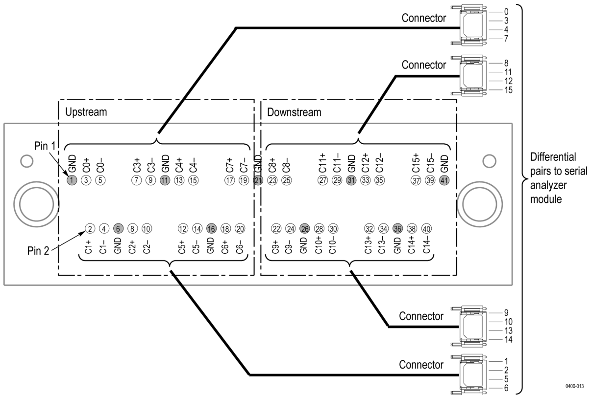
Figure 77: x8 midbus footprint connections for an upstream and downstream configuration
