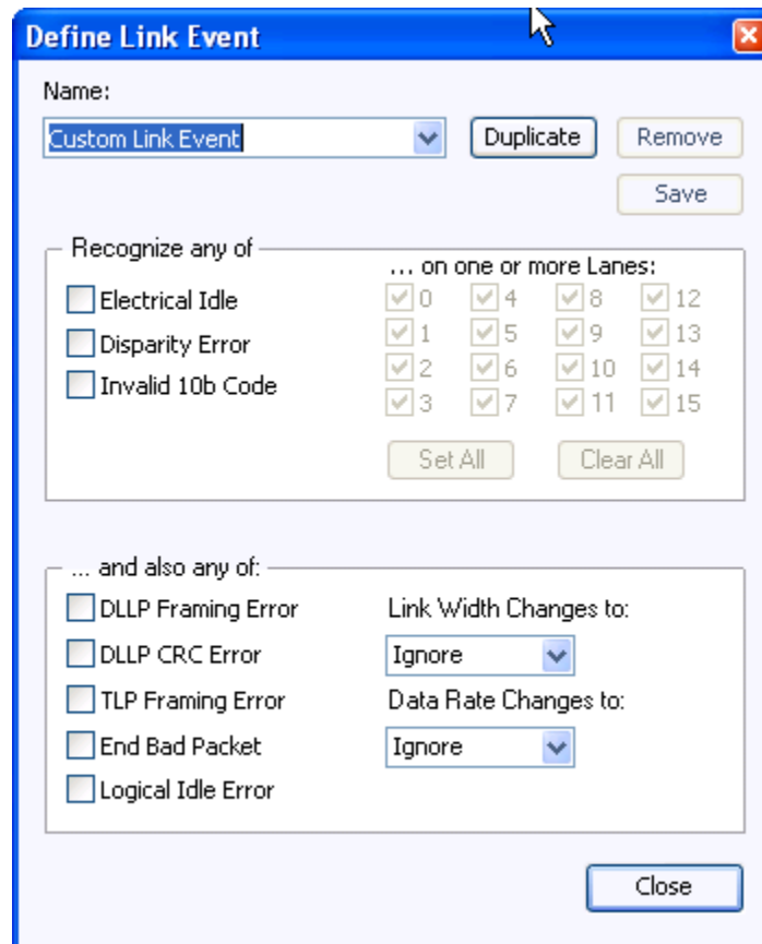
Figure 26: Defining a Link event
