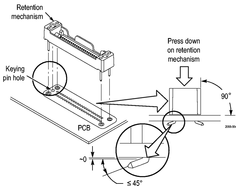
Figure 88: Installing the retention mechanism
