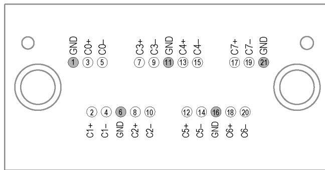
Figure 74: P67SA08 x4 midbus probe footprint pin assignments
