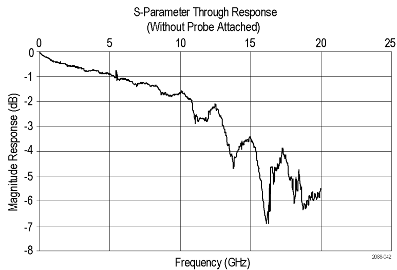
Figure 68: S-parameter data of retention mechanism only
