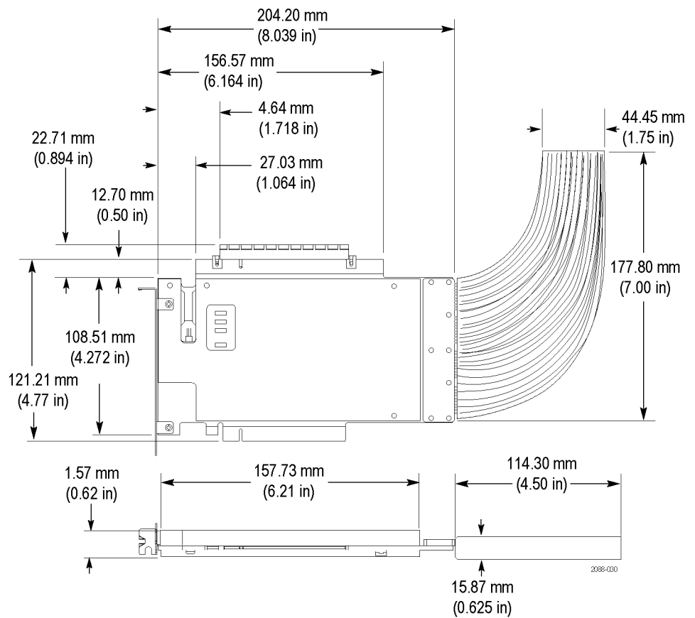
Figure 43: P67SA16S Slot Interposer Probe dimensions
