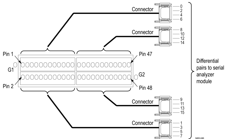
Figure 82: P67SA16G2 x8 midbus footprint connection module connector
