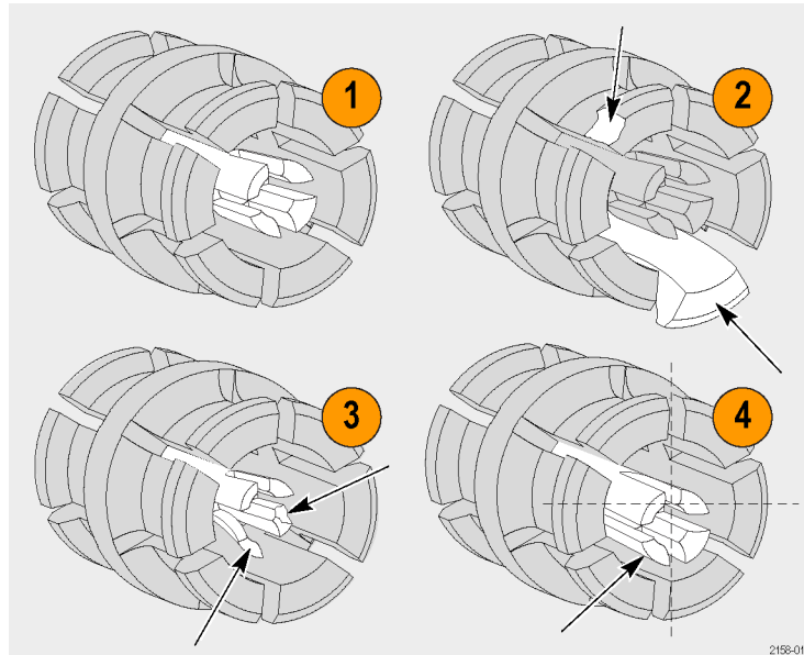
Figure 97: Inspect the bullet contacts
