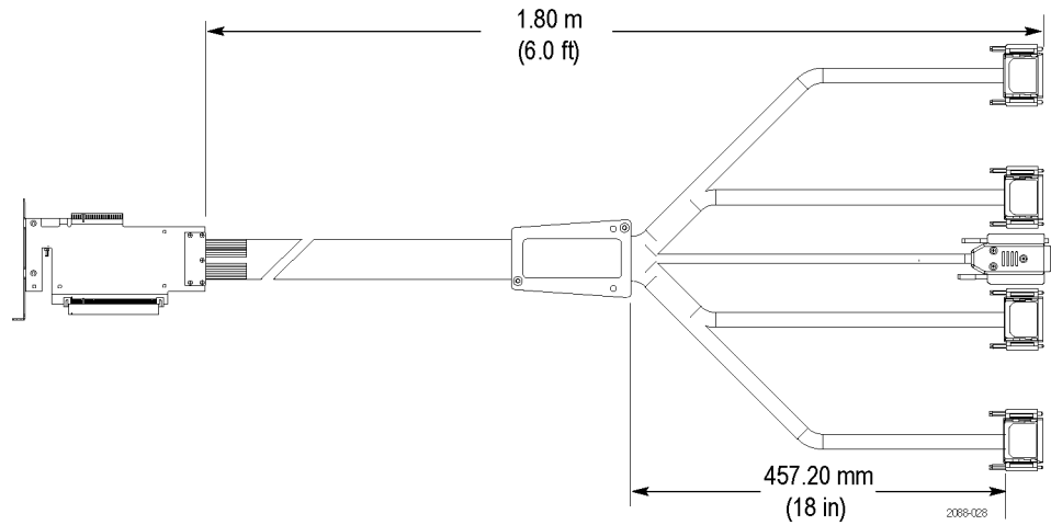
Figure 42: P67SA16S, P67SA08S, P67SA04S and P67SA01S Slot Interposer probe cable lengths
