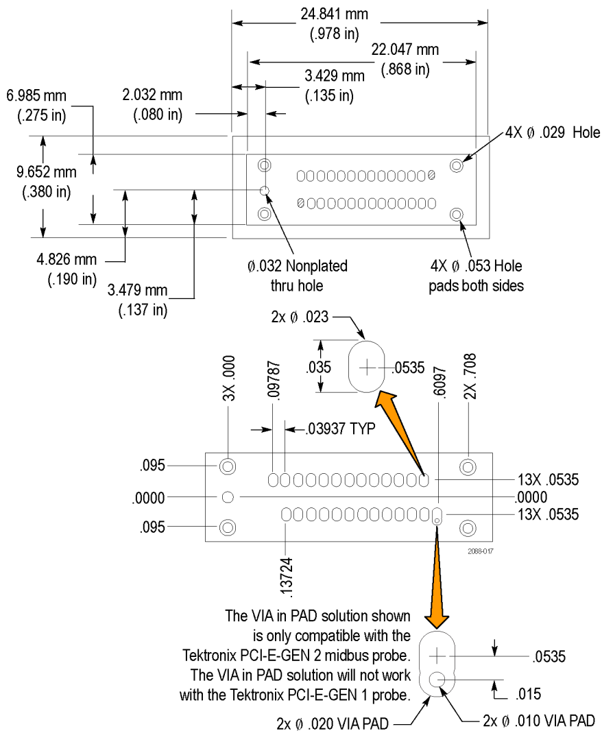
Figure 54: P67SA16G2 x8 midbus footprint dimensions and keep-out area
