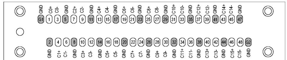
Figure 81: P67SA16G2 midbus probe footprint pin assignments
