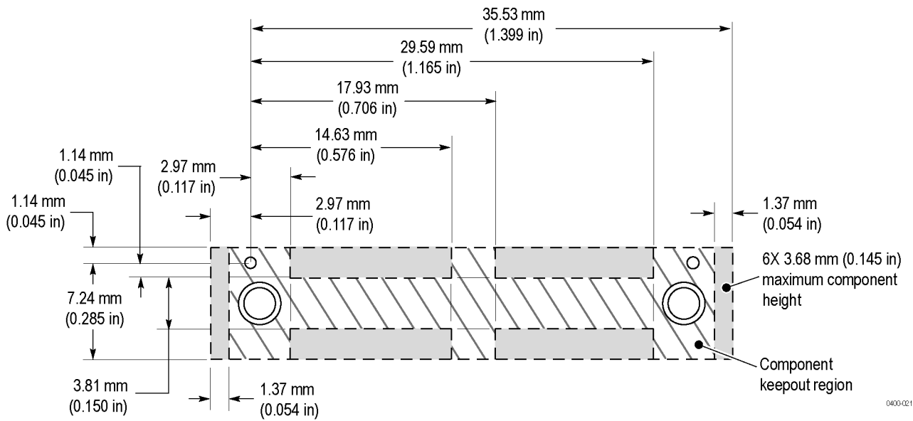
Figure 50: x8 midbus footprint dimension and keep-out area (back side of circuit board)
