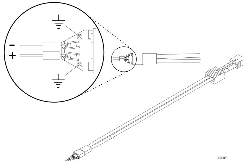
Figure 59: TriMode Resistor Solder Tip
