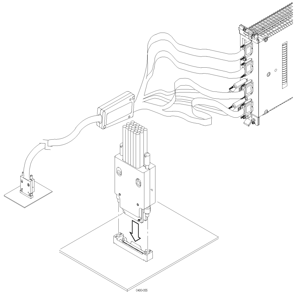
Figure 10: Connecting a probe to the retention mechanism
