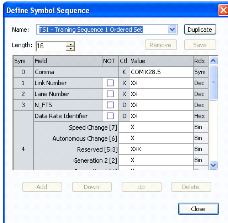
Figure 28: Defining a symbol sequence
