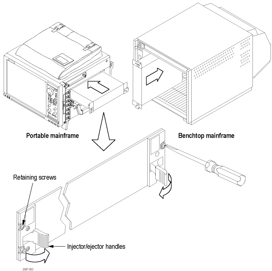
Figure 7: Installing a module
