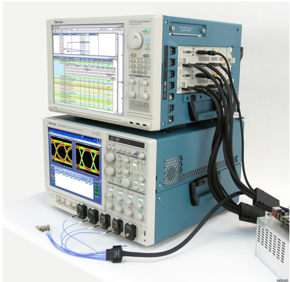
Figure 84: P67UHDSMA probe connected to the inputs of a Tektronix oscilloscope (example 2)
