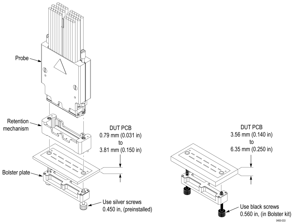
Figure 86: Connecting the P67SA16 midbus probe to the retention mechanism on the circuit board
