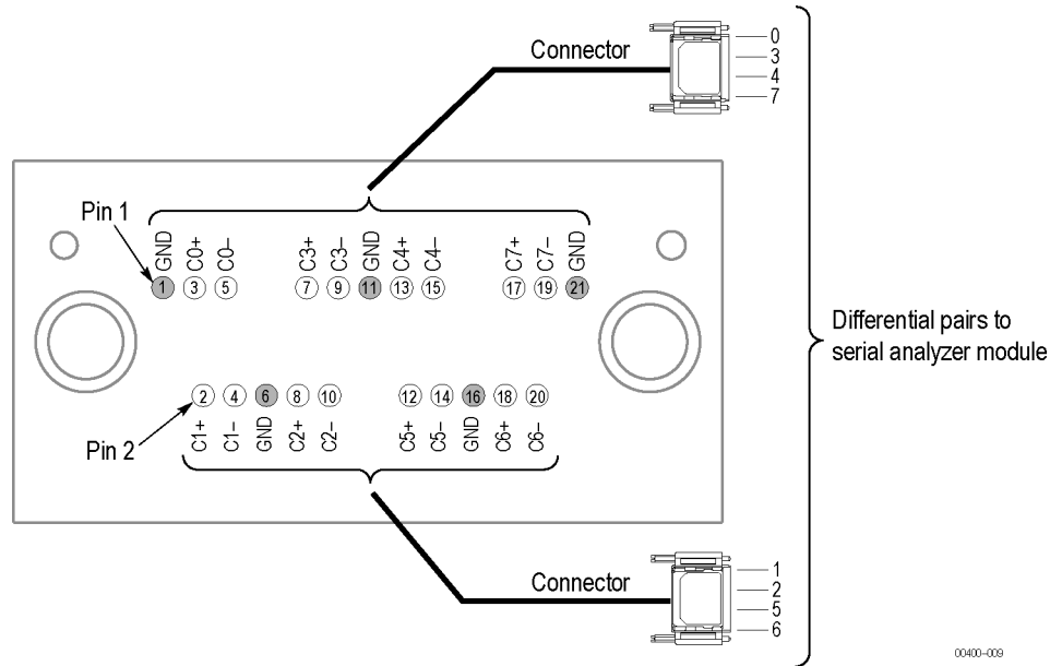
Figure 78: x4 midbus footprint connections for an upstream or downstream configuration
