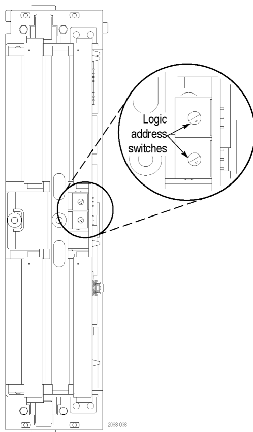
Figure 6: TL7SA16 rear panel
