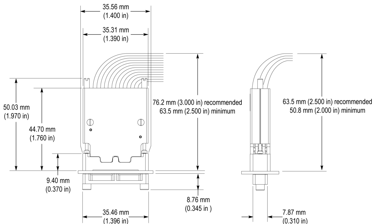
Figure 41: P67SA16 midbus probe head dimensions
