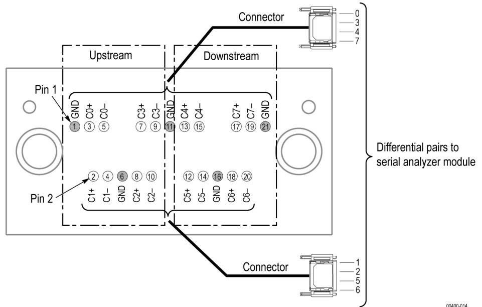
Figure 80: x4 midbus footprint connections for an upstream and downstream configuration.
