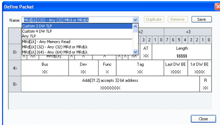
Figure 22: Defining a TLP
