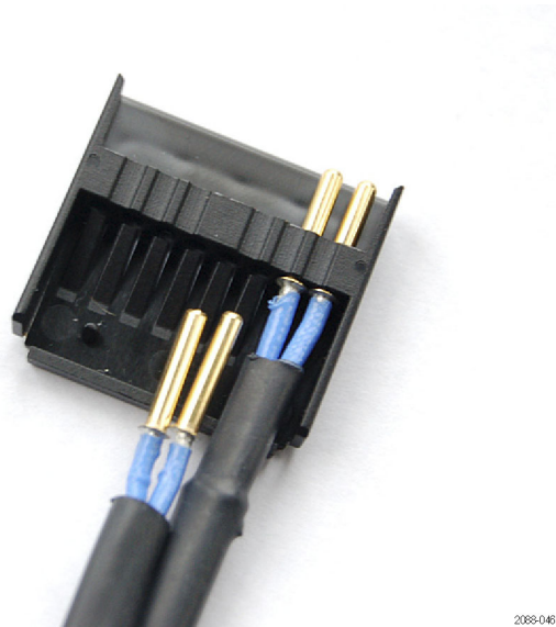
Figure 94: Inserting additional probe wires
