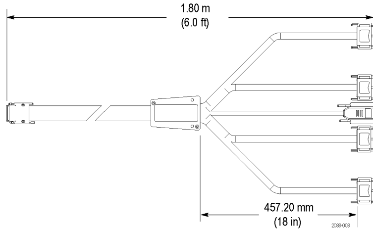
Figure 39: P67SA08 and P67SA16 cable length dimensions
