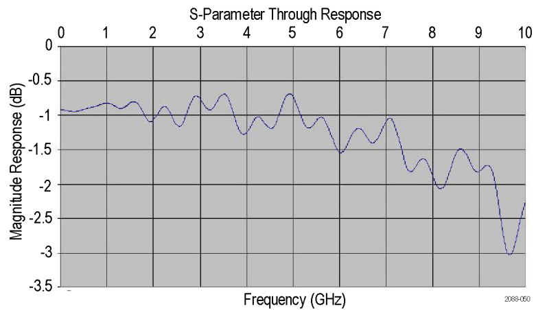
Figure 71: S-parameter data of P67SA01SD Solder-Down probe
