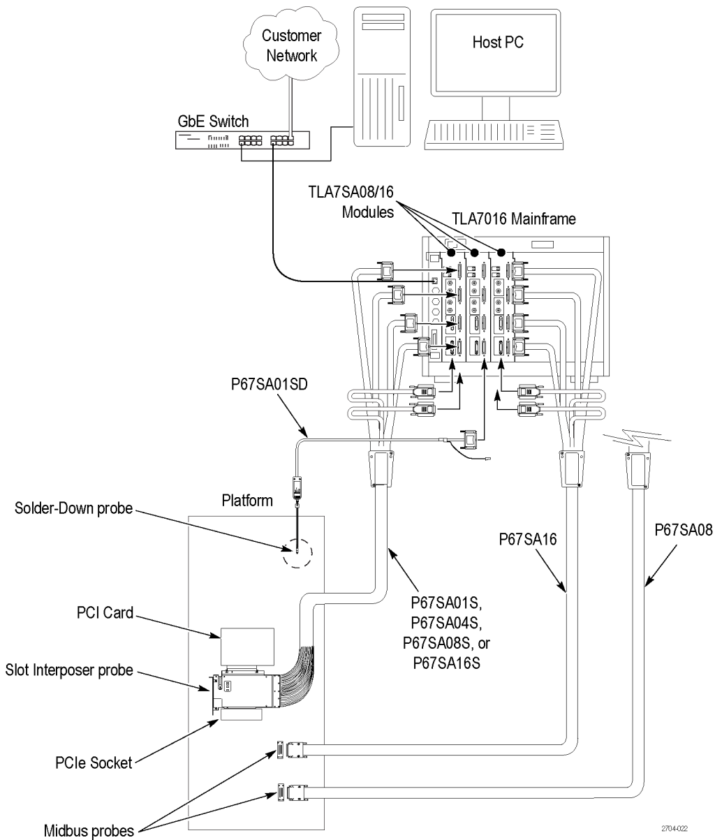
Figure 8: Installation overview
