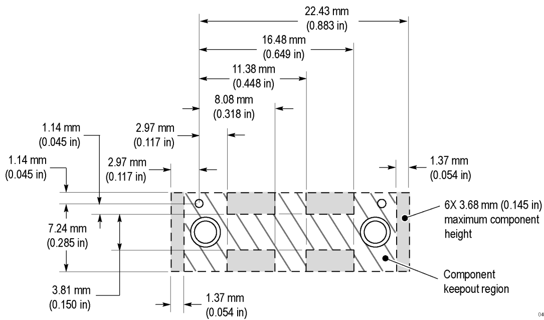
Figure 53: x4 midbus footprint dimension and keep-out area (back side of circuit board)
