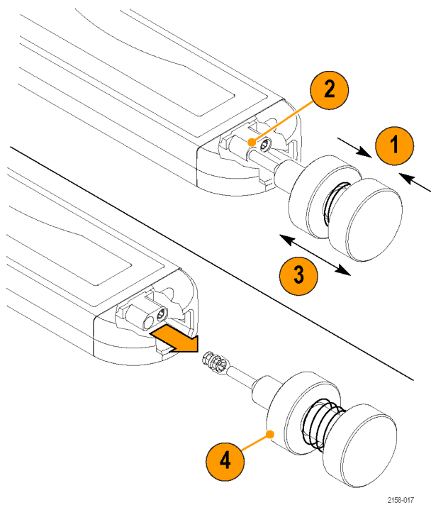
Figure 96: Removing the bullet contacts
