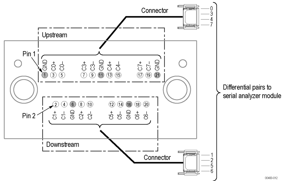
Figure 79: x4 midbus footprint connections for an upstream and downstream configuration
