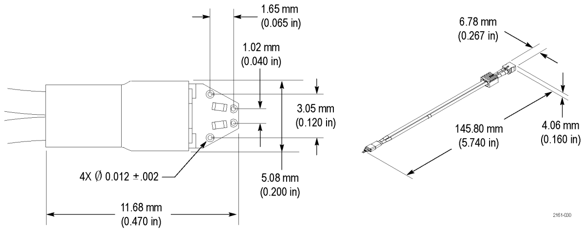
Figure 46: P75TLRST Solder Tip dimensions
