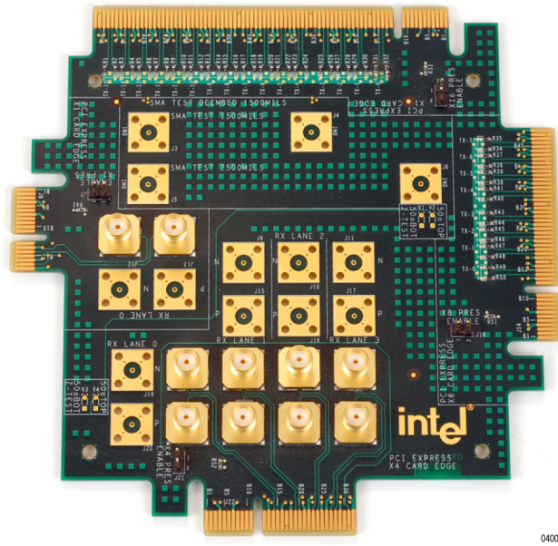
Figure 45: PCI Express Compliance Load Board (CLB1)
