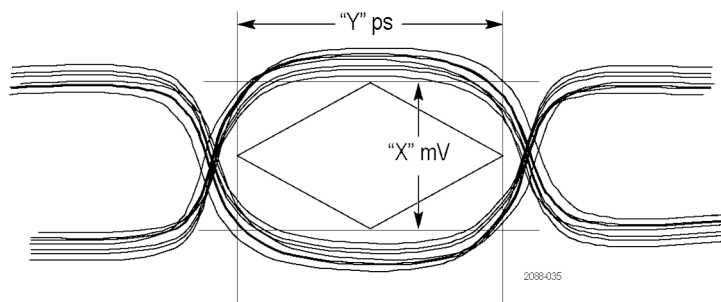
Figure 66: Signal eye measurements (time versus voltage)
