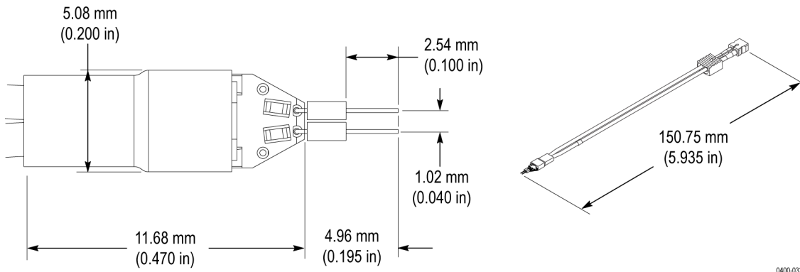
Figure 47: TriMode Resistor Solder Tip dimensions
