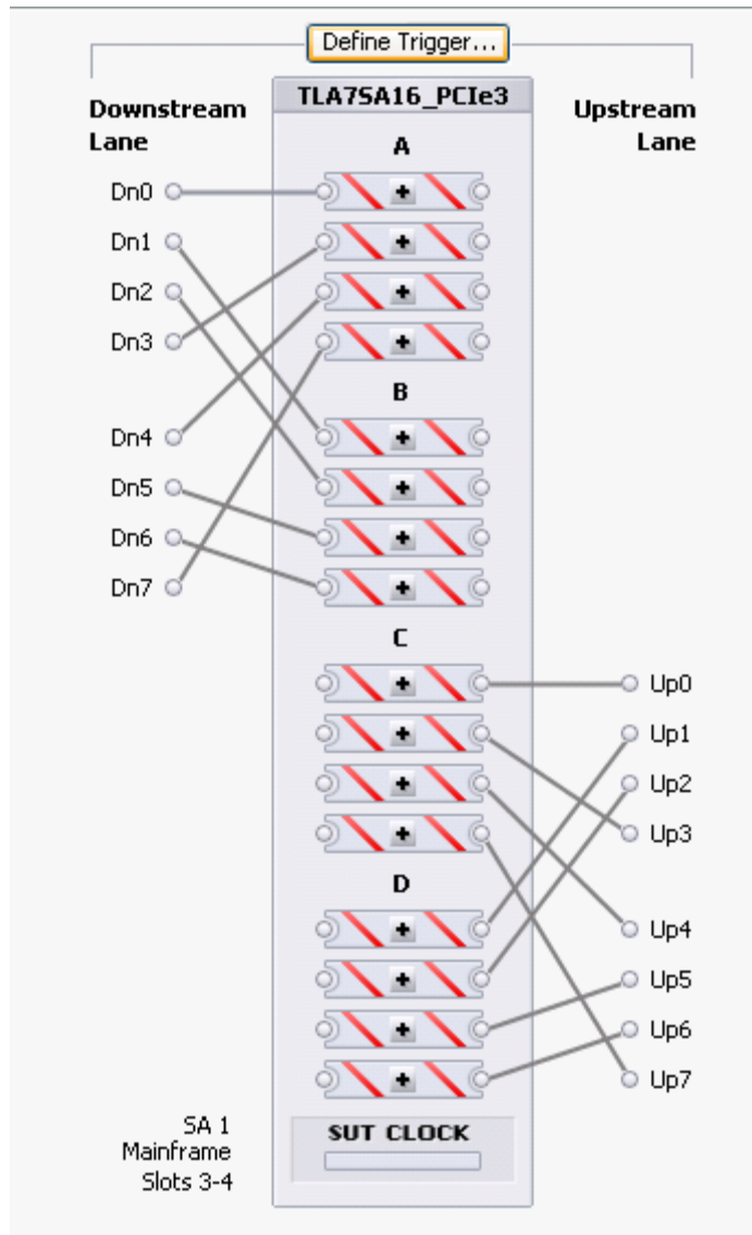
Figure 19: Channel-lane connectors
