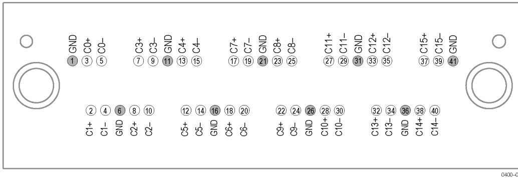
Figure 73: P67SA16 x8 midbus probe footprint pin assignments
