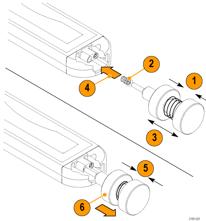
Figure 98: Installing the bullet contacts
