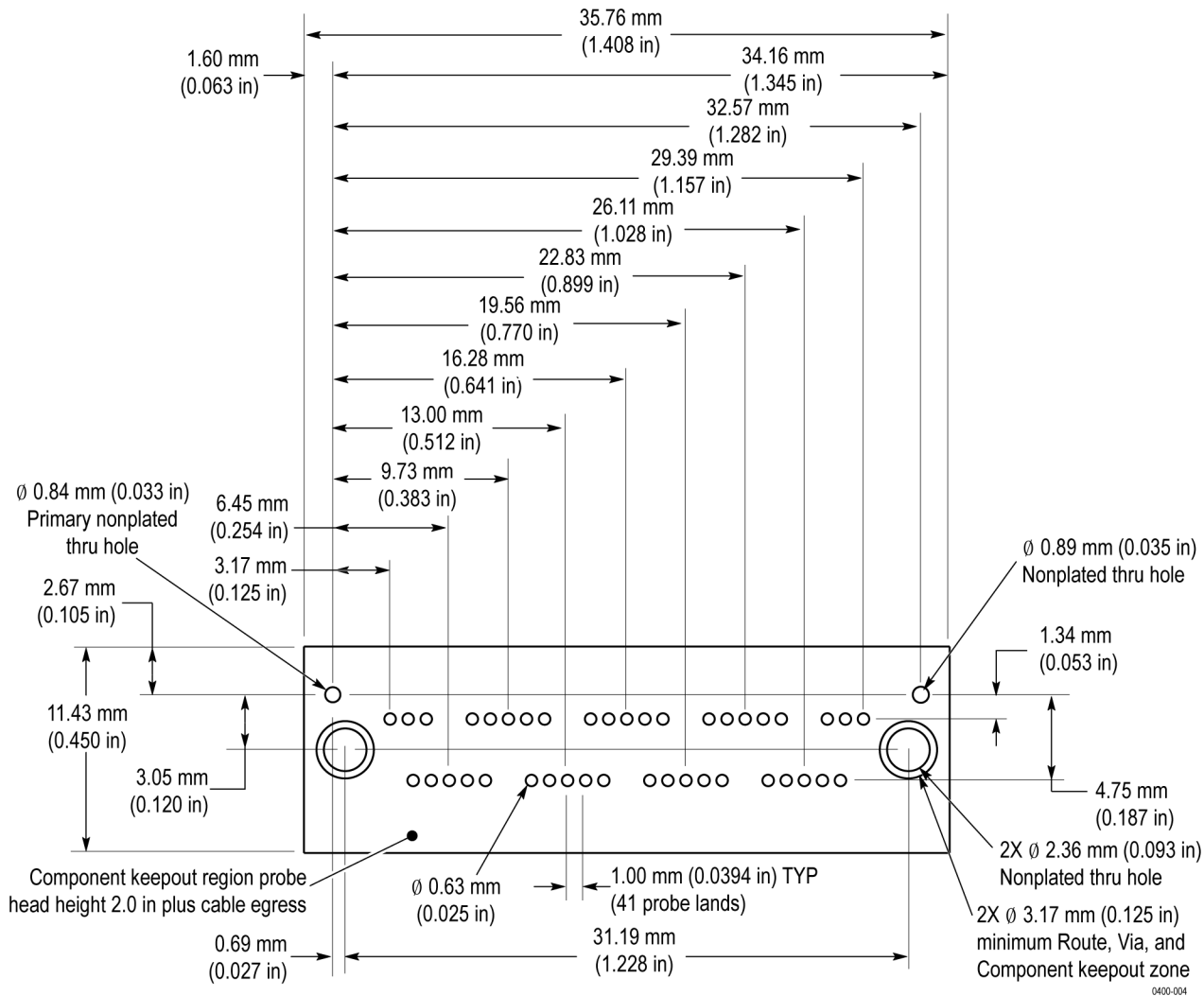
Figure 49: x8 midbus footprint dimensions and keep-out area (front side of circuit board)
