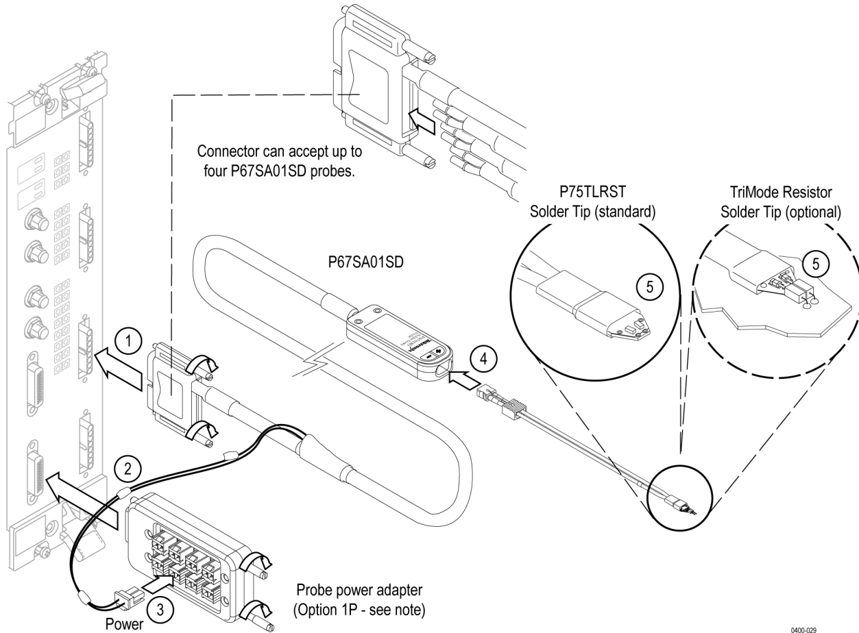
Figure 48: Connecting the P67SA01SD Solder-Down probe
