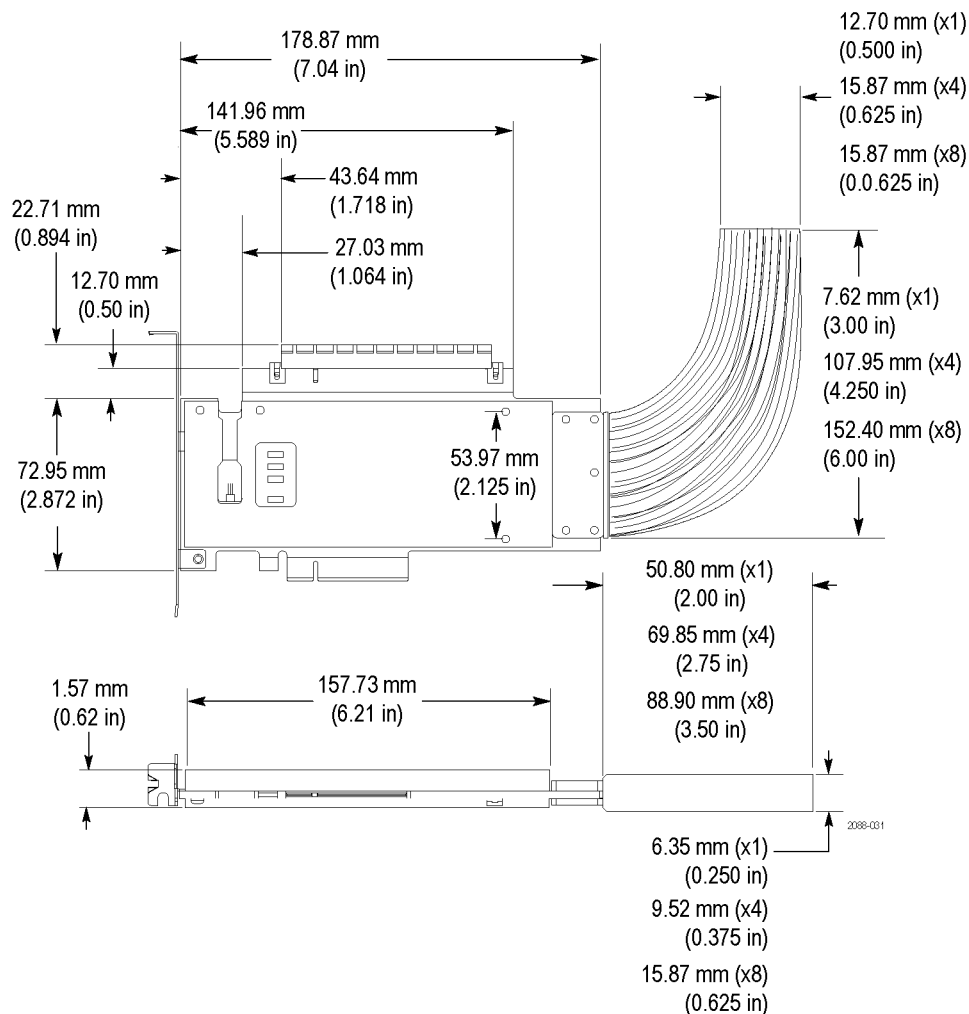
Figure 44: P67SA01S, P67SA04S, and P67SA08S Slot Interposer probe dimensions
