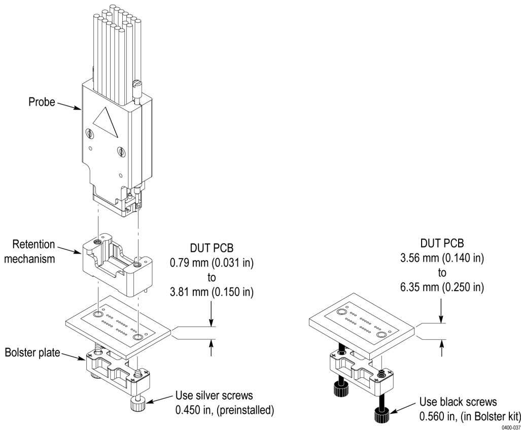
Figure 87: Connecting the P67SA08 midbus probe to the retention mechanism on the circuit board
