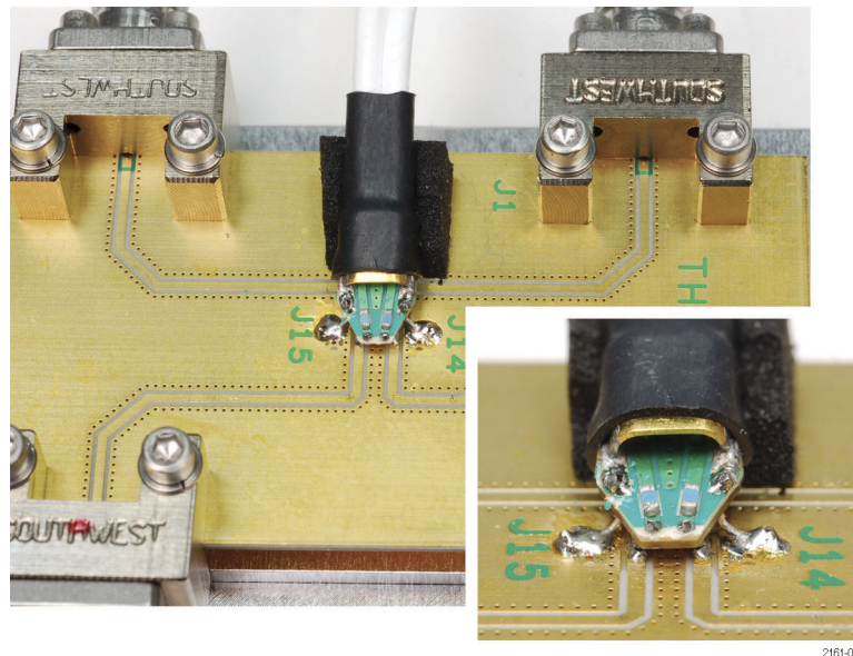
Figure 60: Typical wire length from probe tip to circuit
