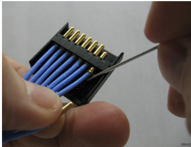
Figure 93: Removing individual wires
