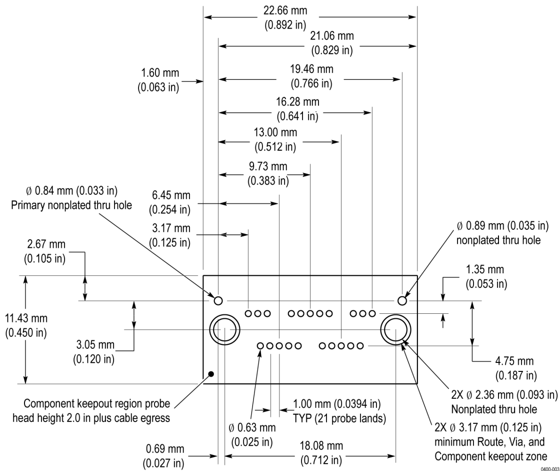
Figure 52: x4 midbus footprint dimensions and keep-out area (front side of circuit board)
