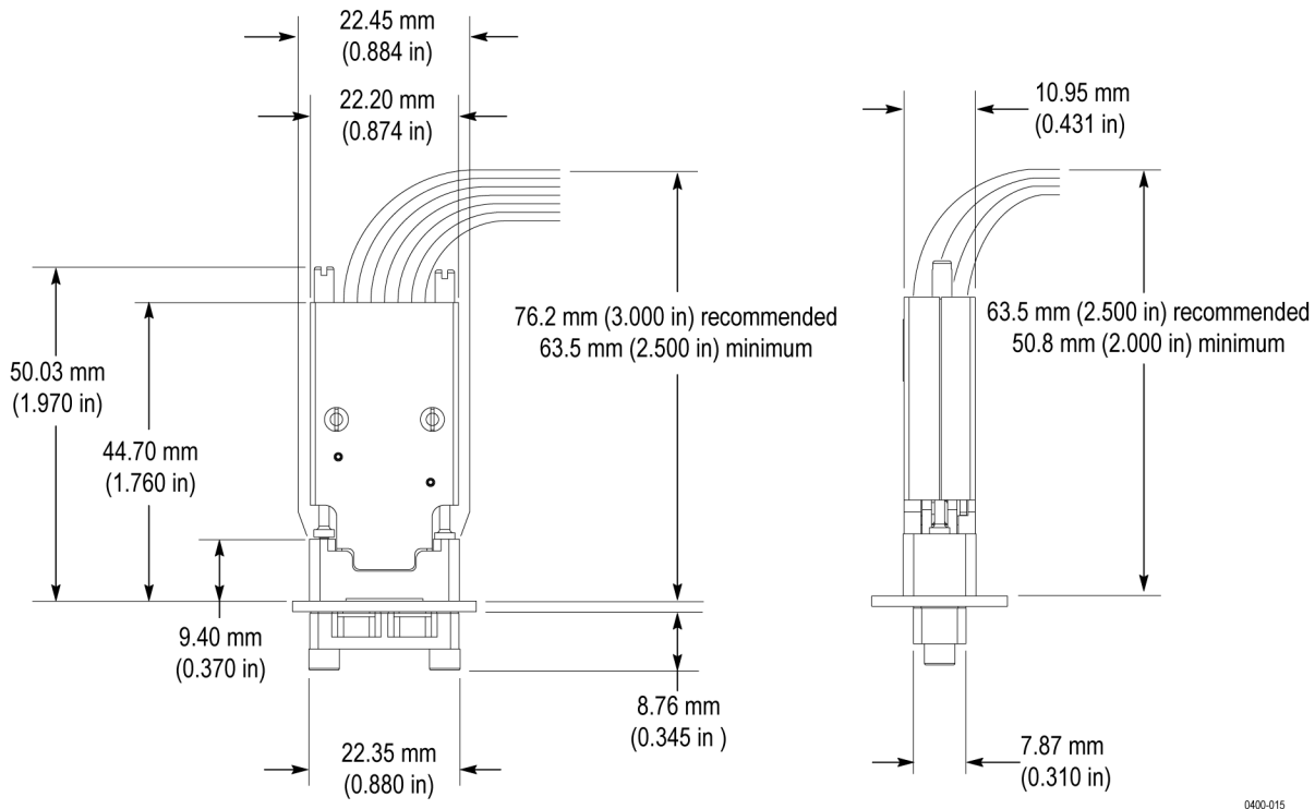
Figure 40: P67SA08 midbus probe head dimensions
