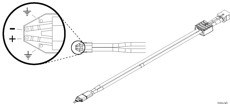
Figure 58: P75TLRST TriMode Long Reach Solder Tip
