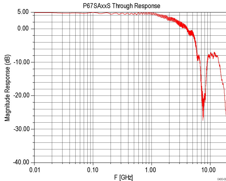
Figure 70: Probe impact of the P67SAxxS slot probe
