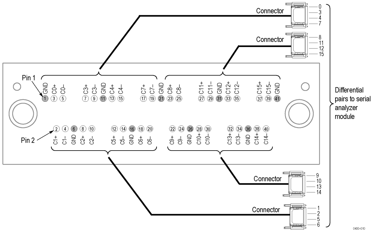
Figure 75: x8 midbus footprint connections for an upstream or downstream configuration
