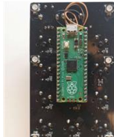
Raspberry Pi Pico RGB CherryMX-Macro-Keyboard
