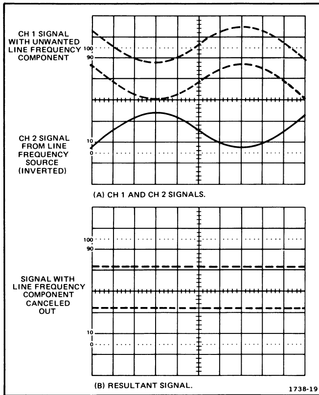
Fig. 17. Common-mode rejection.
