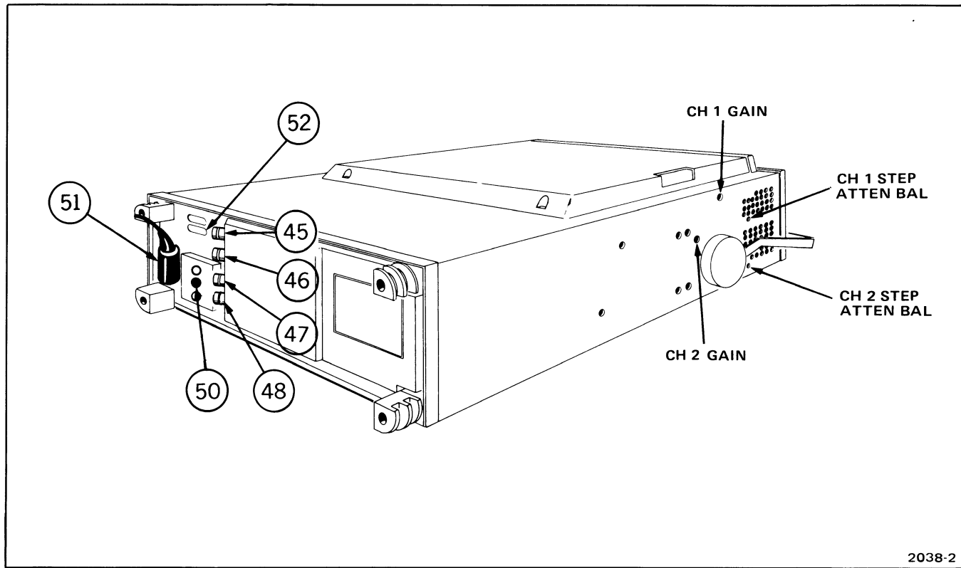
Fig. 7. Rear panel and left side panel controls, connectors, and indicators.
