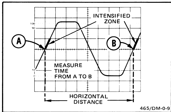
Fig. 26. Time duration.
