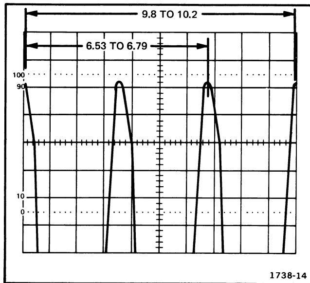
Fig. 12. Basic 465 timing check.
