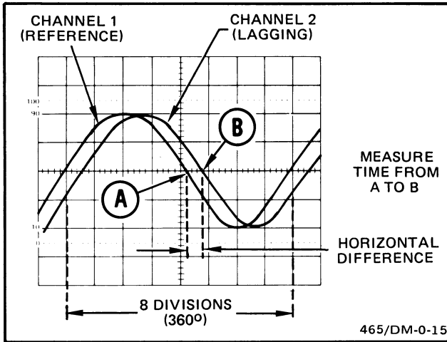
Fig. 21. Phase difference.
