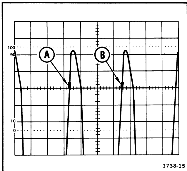
Fig. 13. DM44 timing check.
