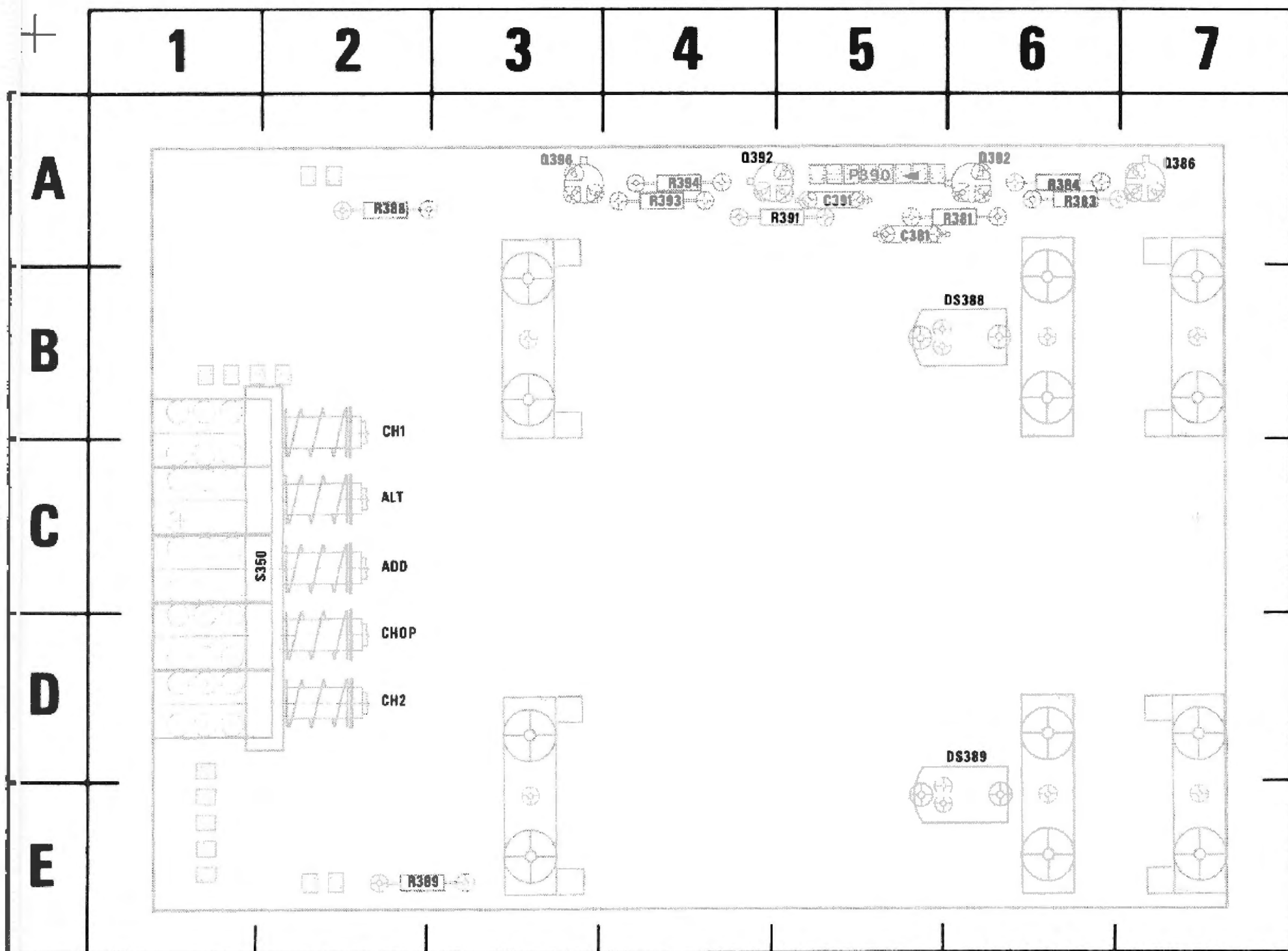
Fig. 8-5. A4—Vertical Mode Switch circuit board.
