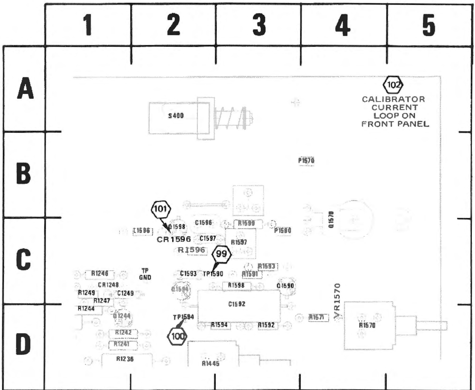
Fig. 8-17. Partial A9—Interface circuit board. (Calibrator Components)
