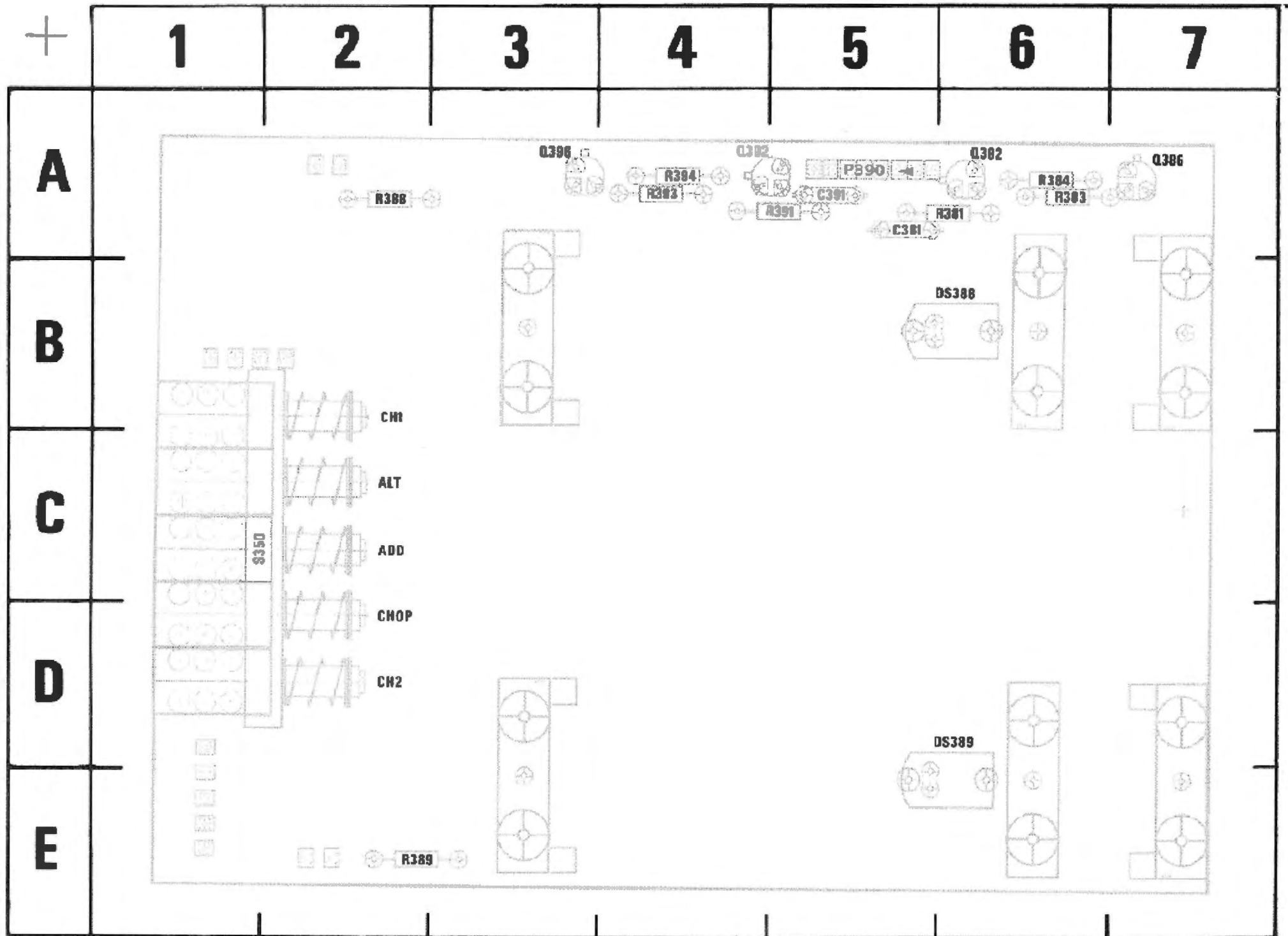
Fig. 8-3. A4-Vertical Mode Switch circuit board.
