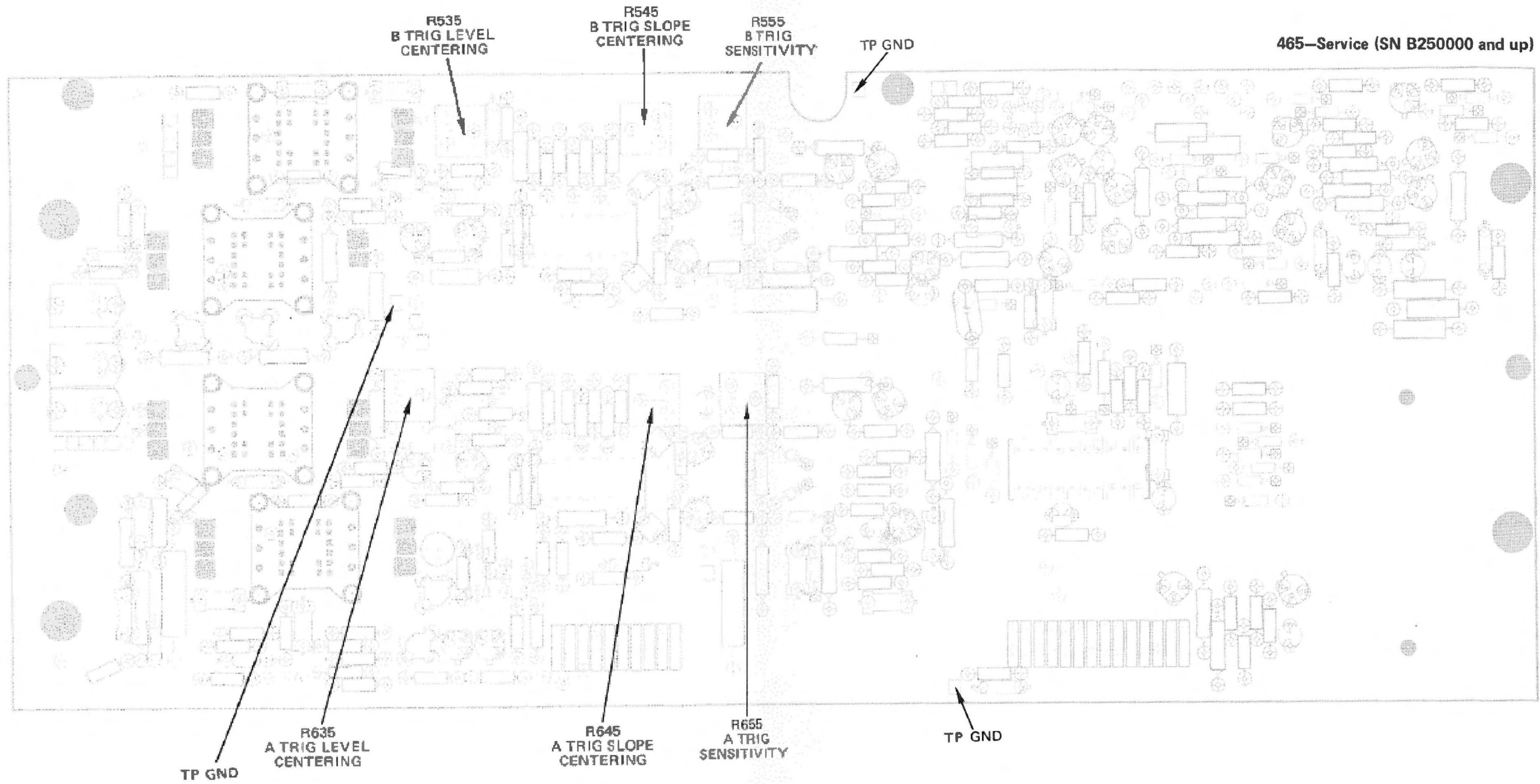
Fig. 8-23. Trigger Generator and Sweep Logic circuit board adjustment locations.
