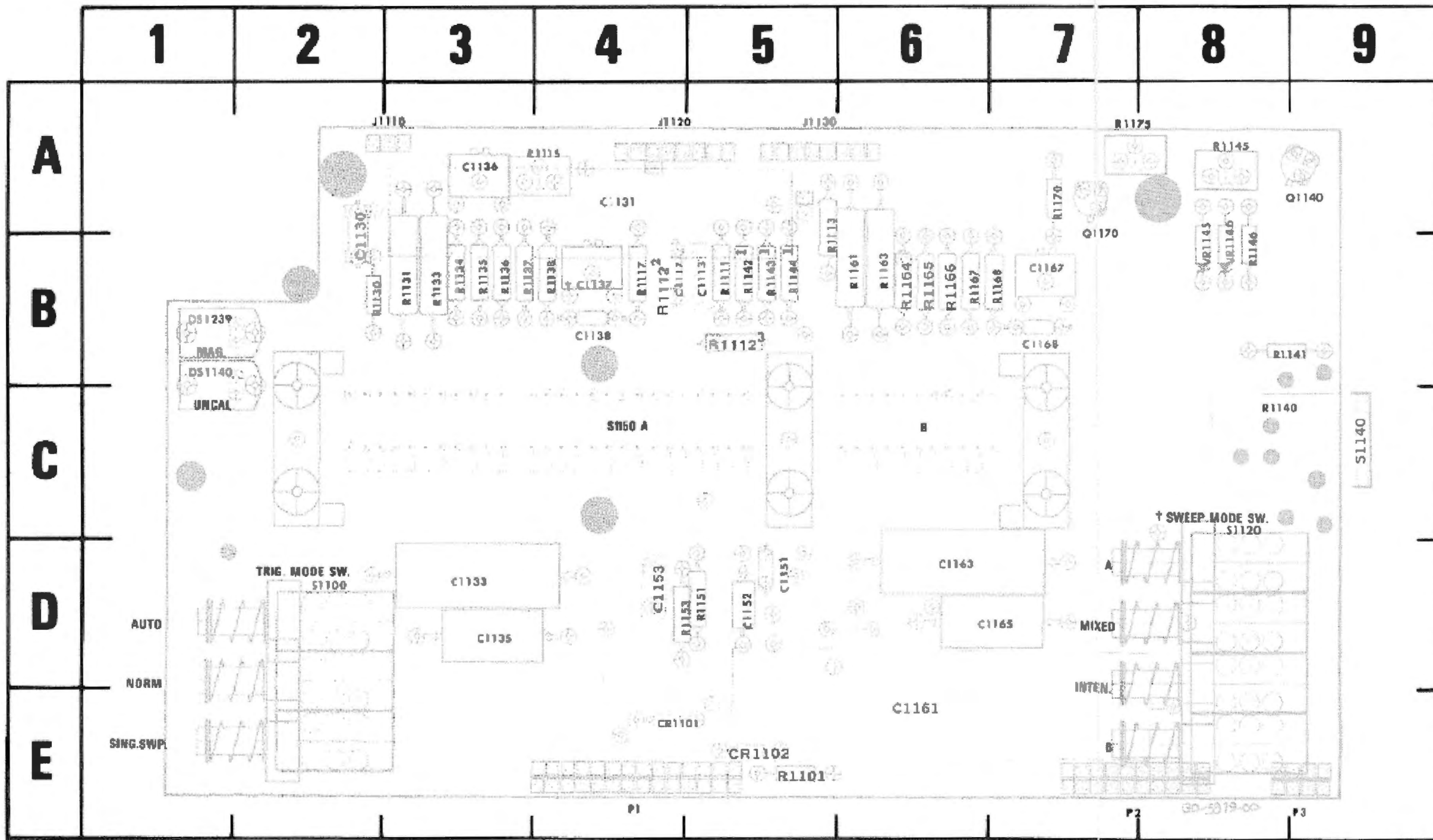
Fig. 8-11. A7—Timing circuit board.
