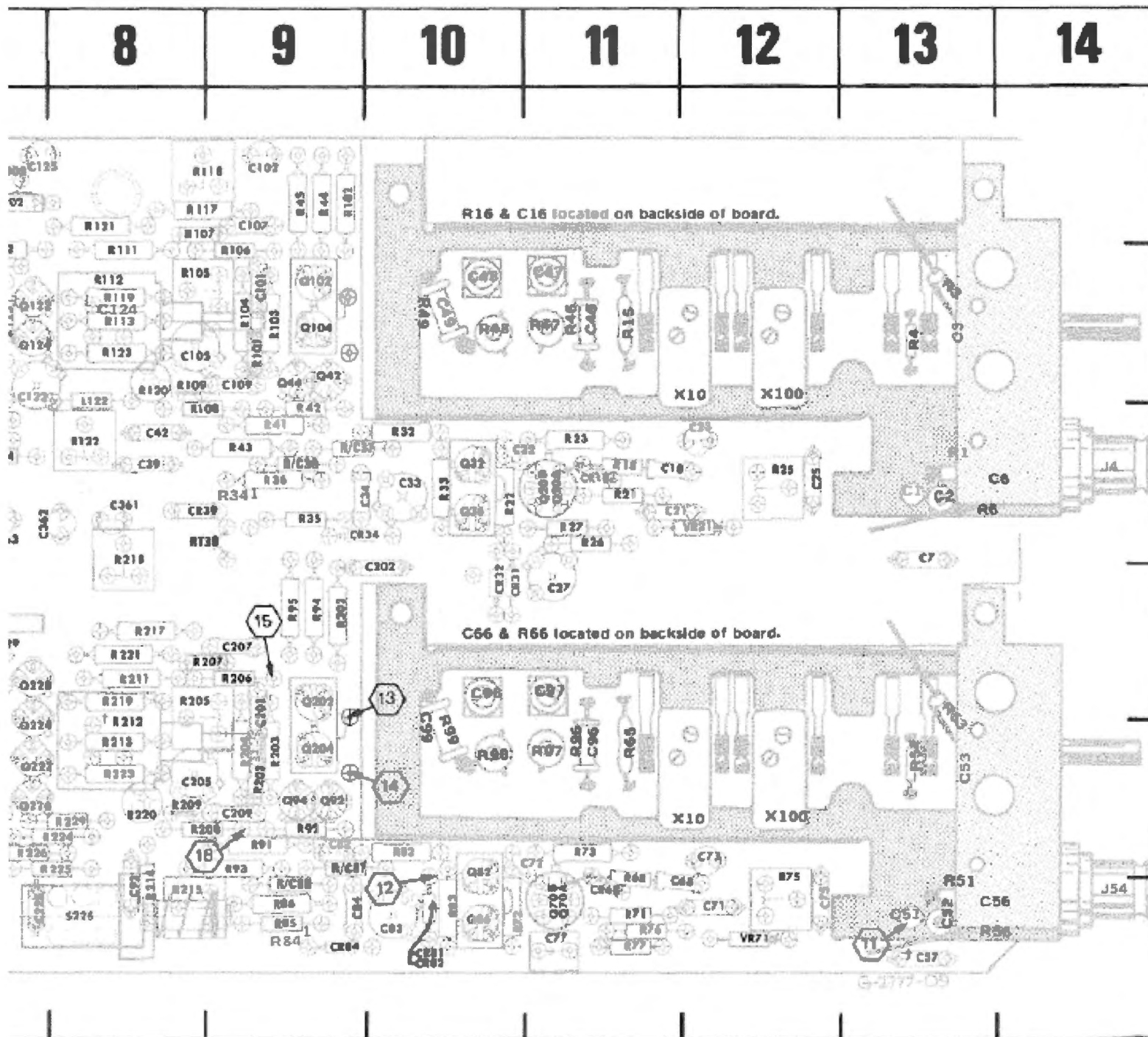
A3—Vertical Preamp circuit boards.
