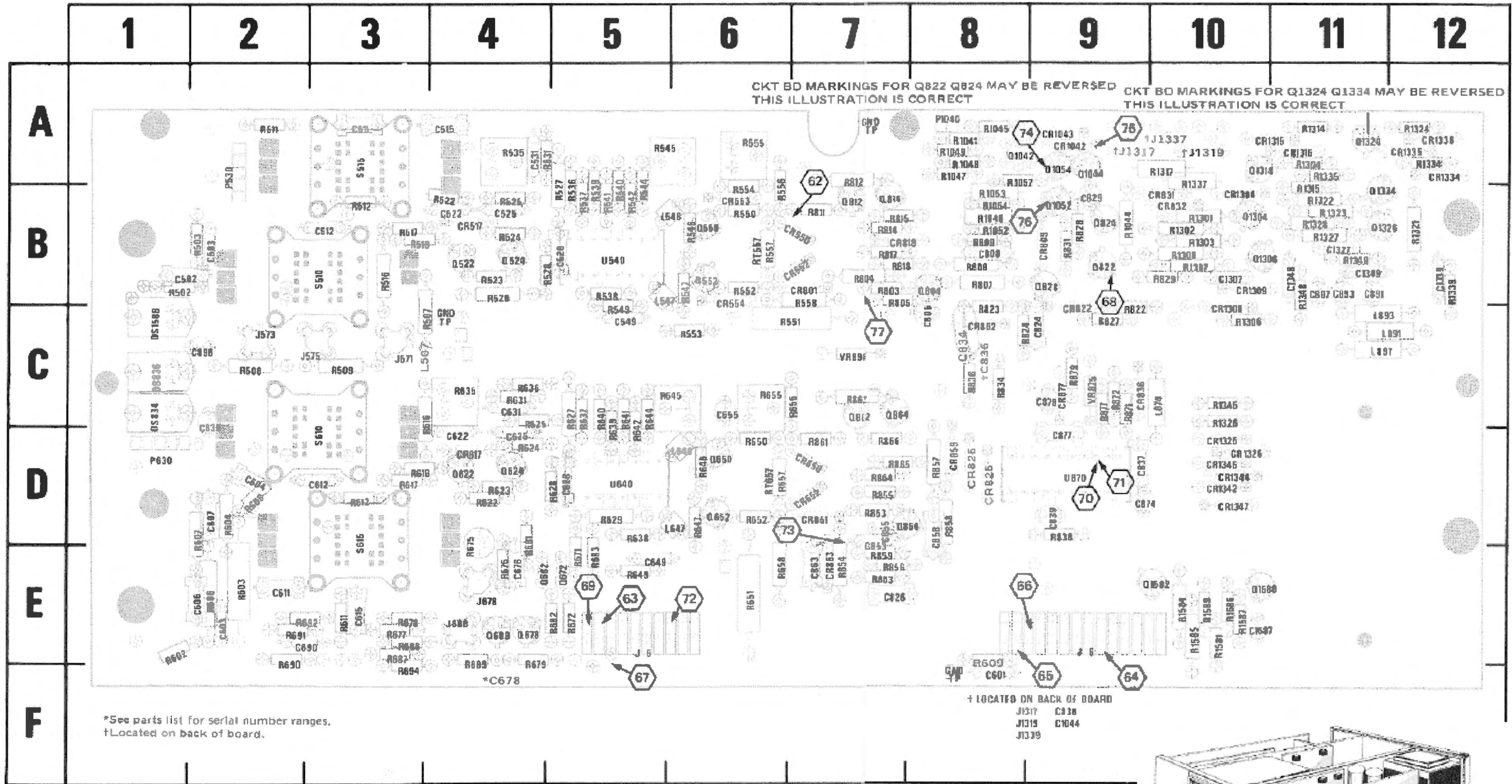
Fig. 8-12. A8—Trigger Generator and Sweep Logic circuit board.
