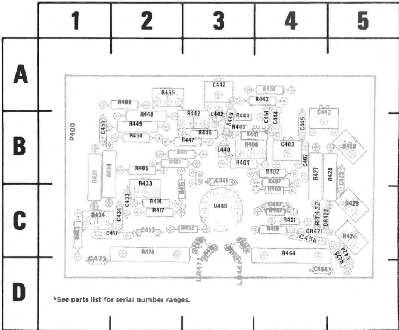
Fig. 8-8. A5b—Vertical Output Amplifier circuit board (IC version).
