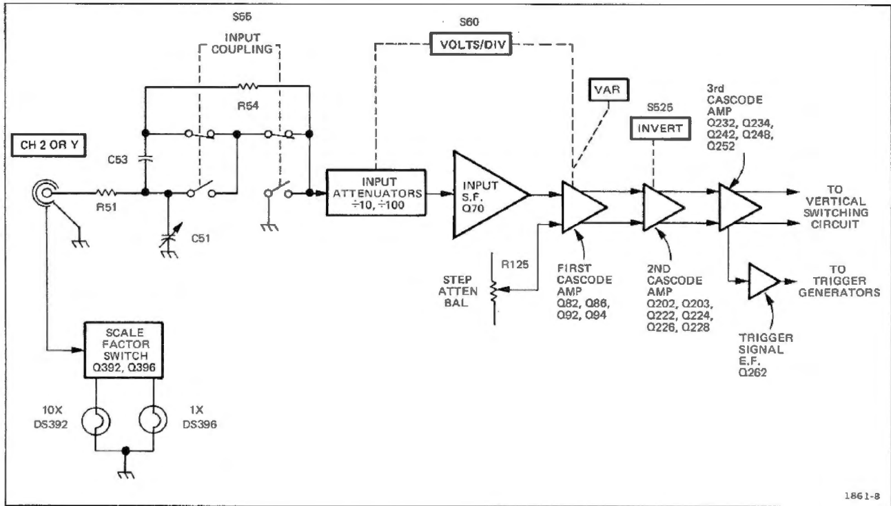
Fig. 3-3. Detailed block diagram of the Channel 2 Preamp.
