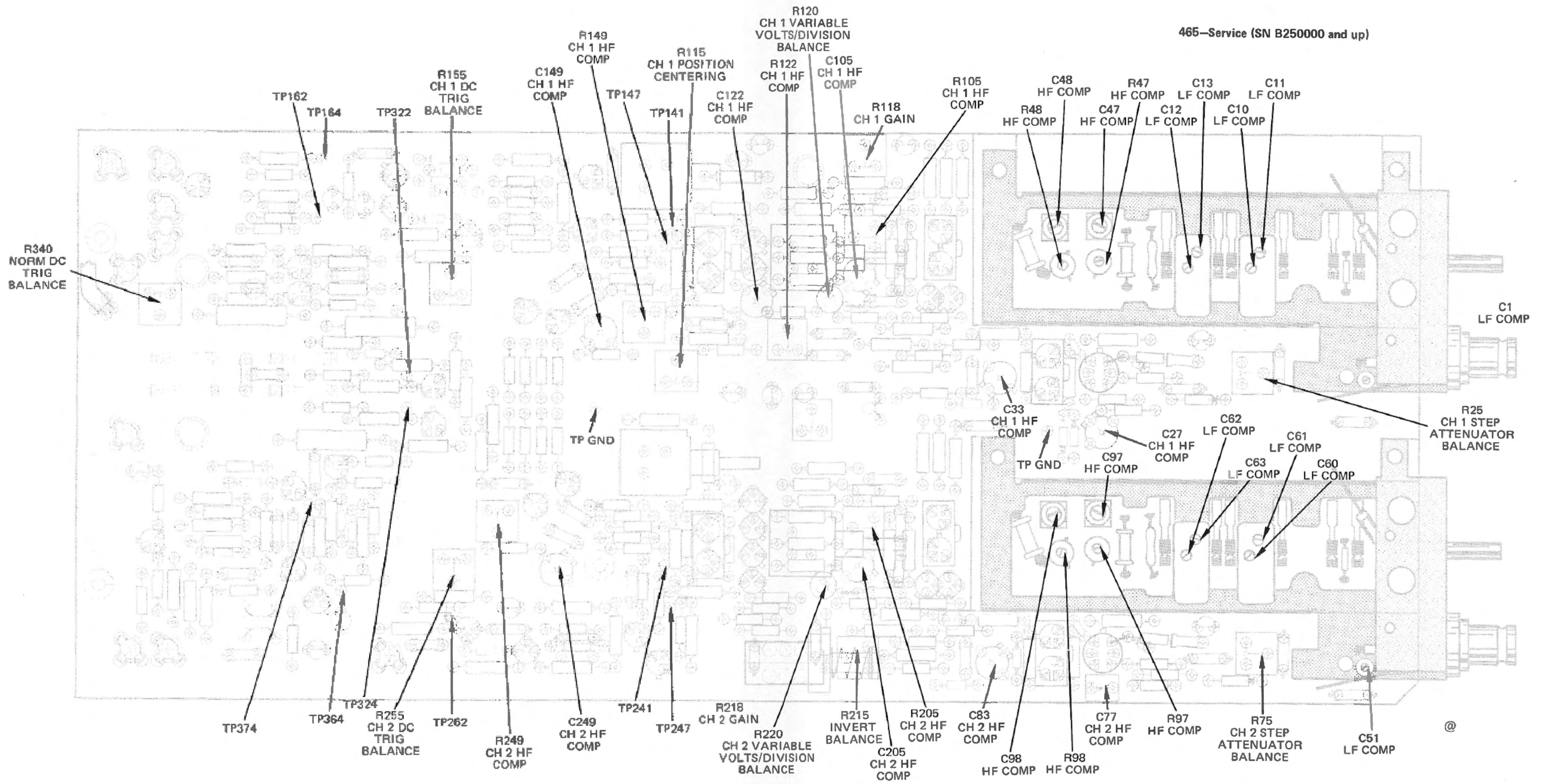
Fig. 8-20. Vertical Preamplifier and Attenuator circuit board adjustment locations.
