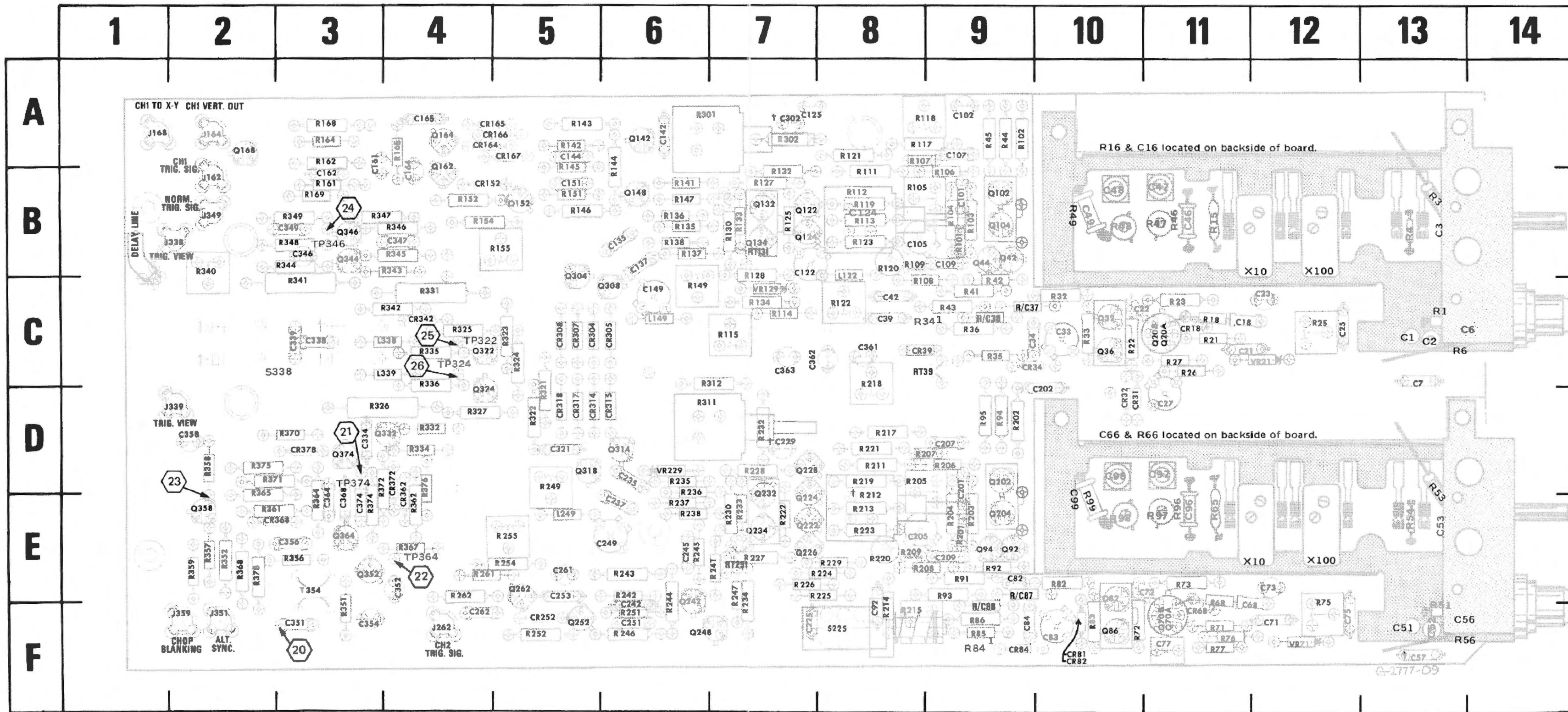
Fig. 8-6. A1 & A2—Attenuators and A3—Vertical Preamp circuit boards.
