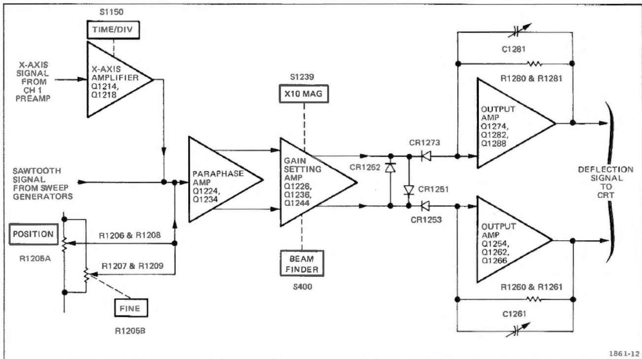
Fig. 3-7. Detailed block diagram of the Horizontal Amplifier.
