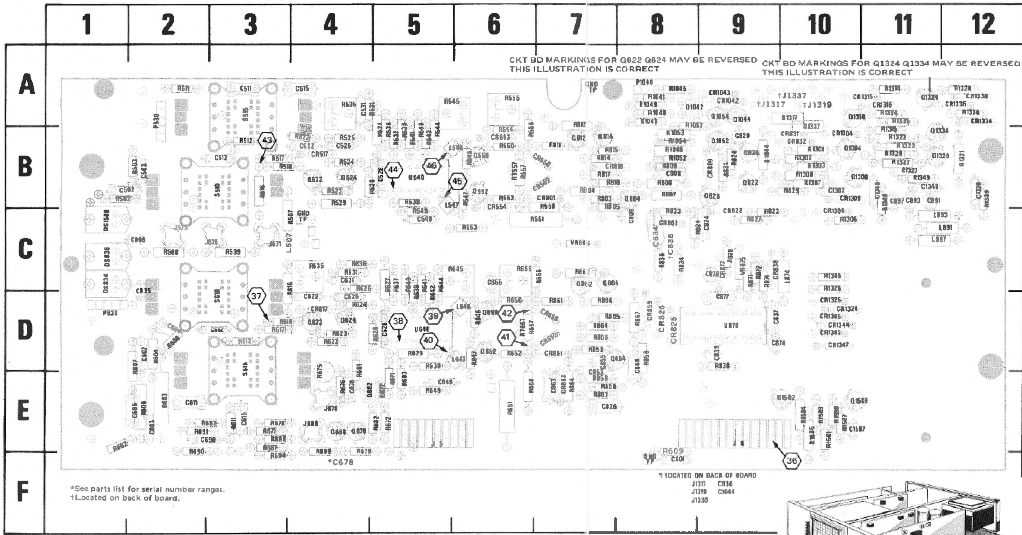
Fig. 8-9. A8—Trigger Generator and Sweep Logic circuit board.
