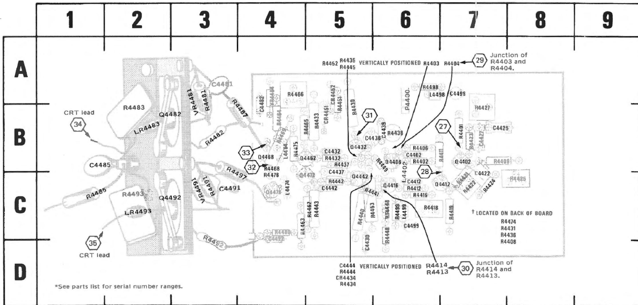
Fig. 8-7. A5a—Vertical Output Amplifier circuit board (discrete version).
