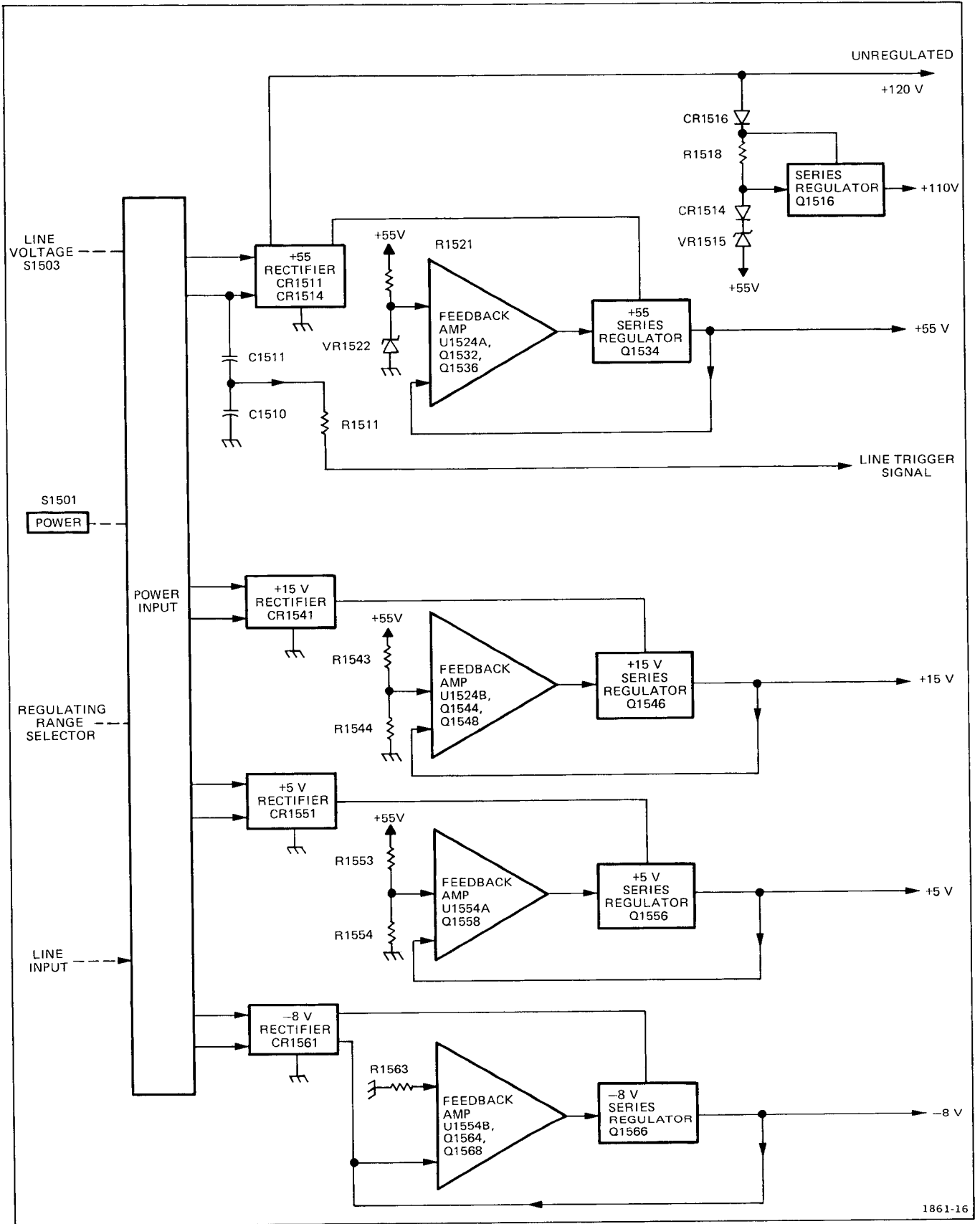
Fig. 3-11. Detailed block diagram of the Low Voltage Power Supply.
