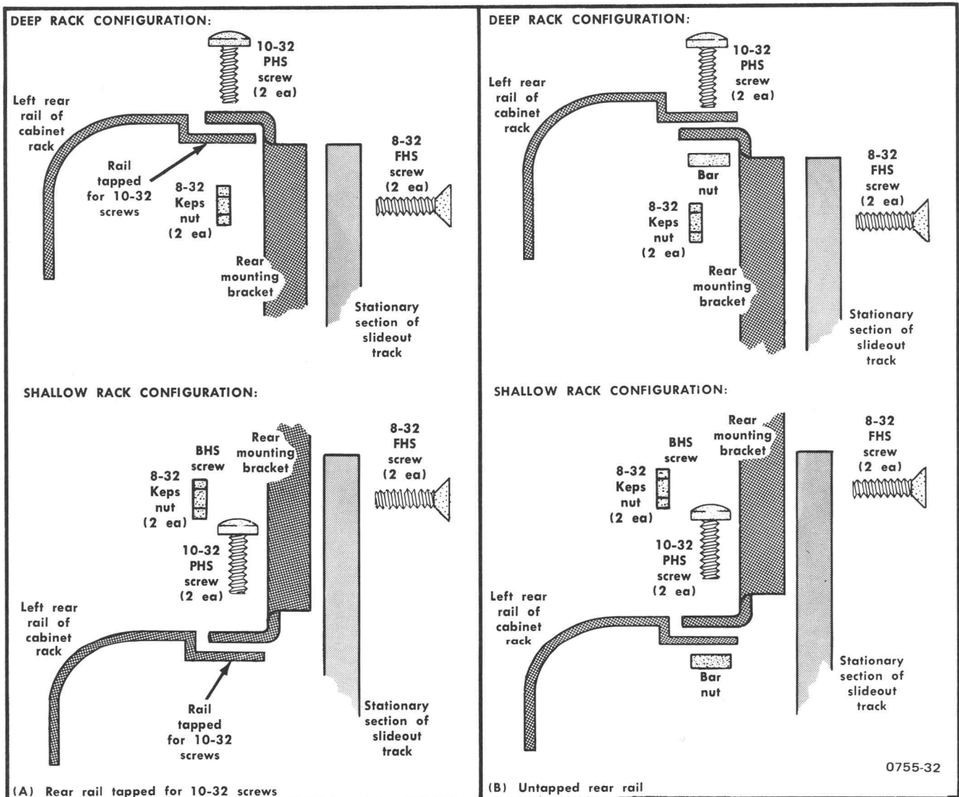
Fig. 4-12. Alternative method of installing the instrument using rear support brackets.
