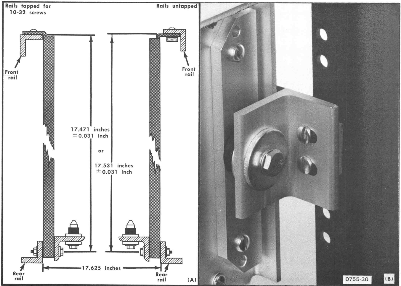
Fig. 4-7. Supporting the rear of the stationary sections: (A) Dimensions necessary; (B) Completed installation.
