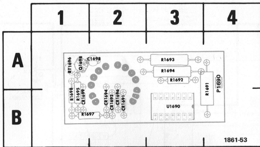
Fig. 8-9. A6—Fan circuit board.
