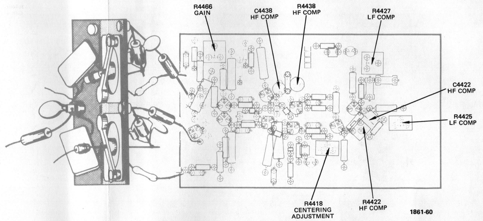
Fig. 8-14. Vertical Output Amplifier circuit board adjustment locations (discrete version).
