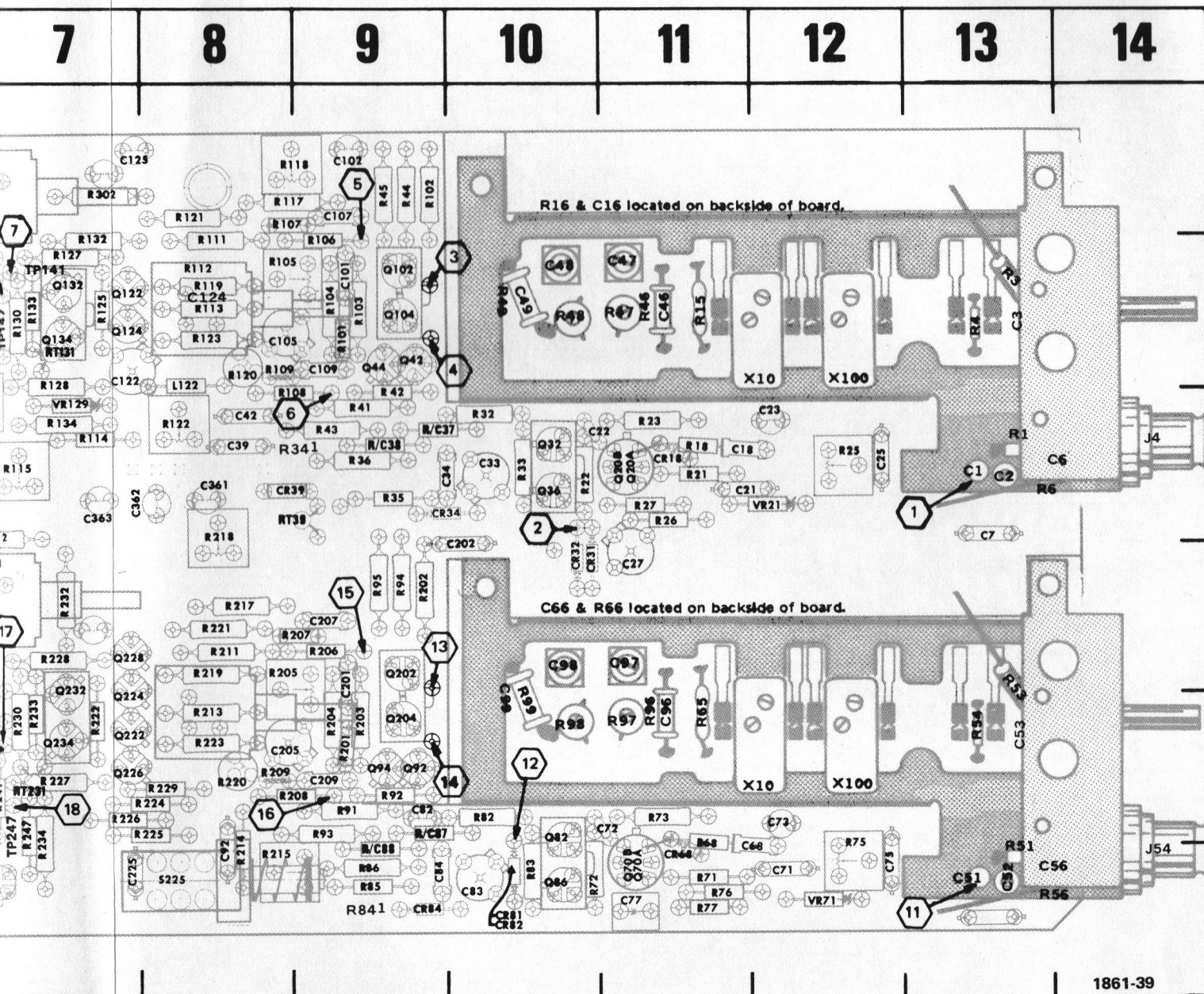
& A2—Attenuators and A3—Vertical Preamp circuit boards.
