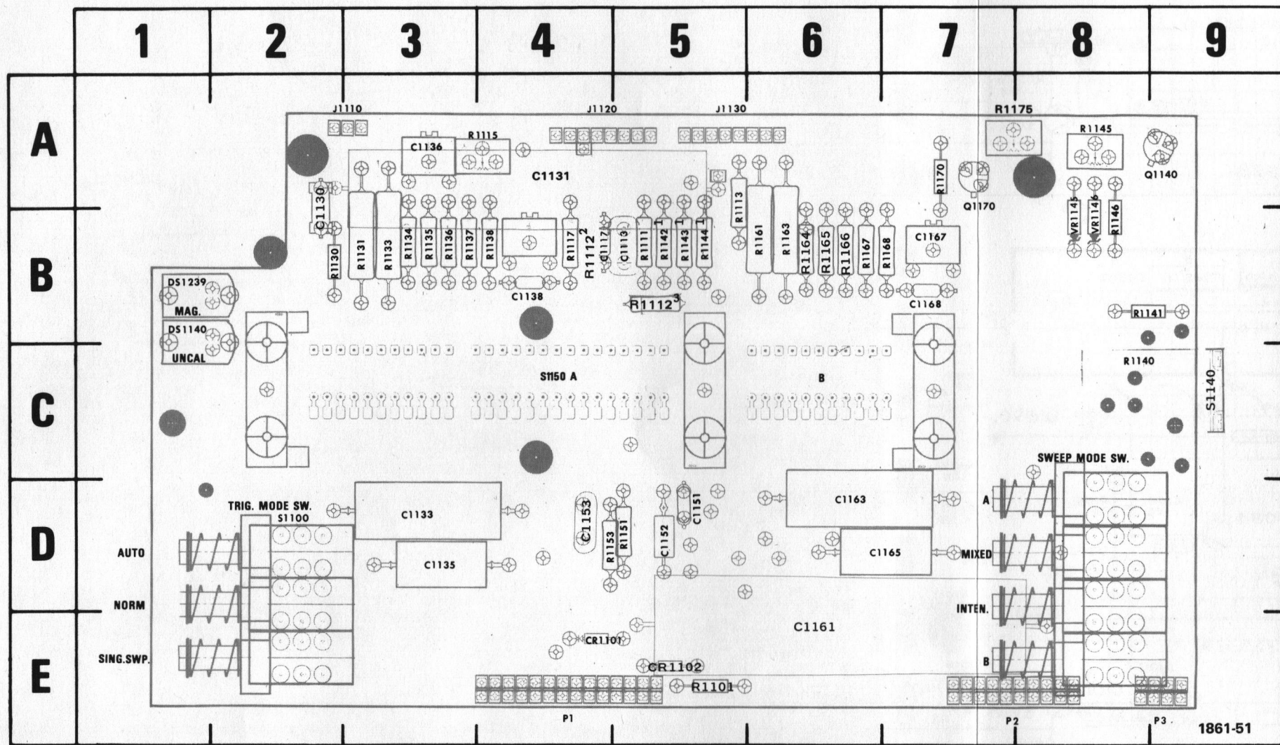
Fig. 8-8. A7—Timing circuit board.
