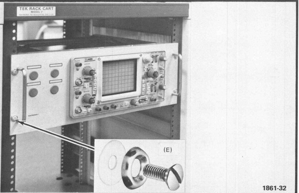
Fig. 4-10. Procedure for inserting or removing the instrument after the slide-out tracks have been installed.
