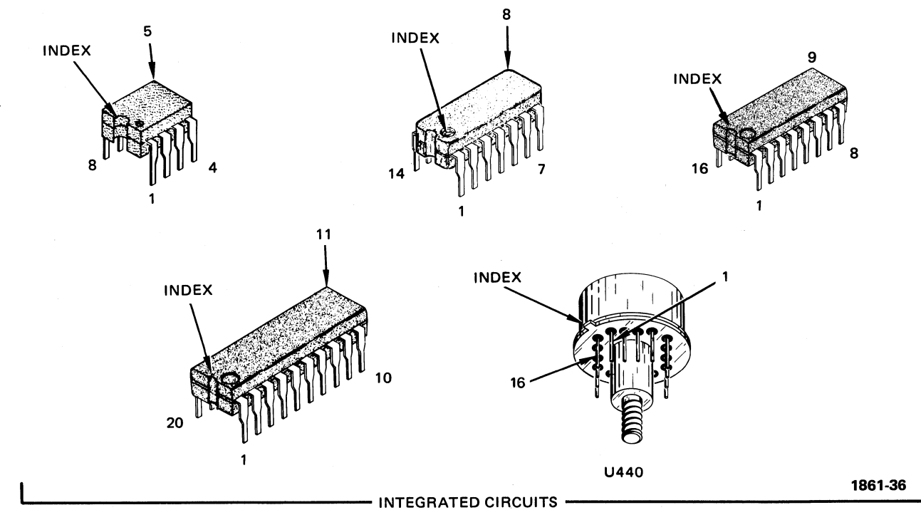
Fig. 8-1. Semiconductor lead configurations.
