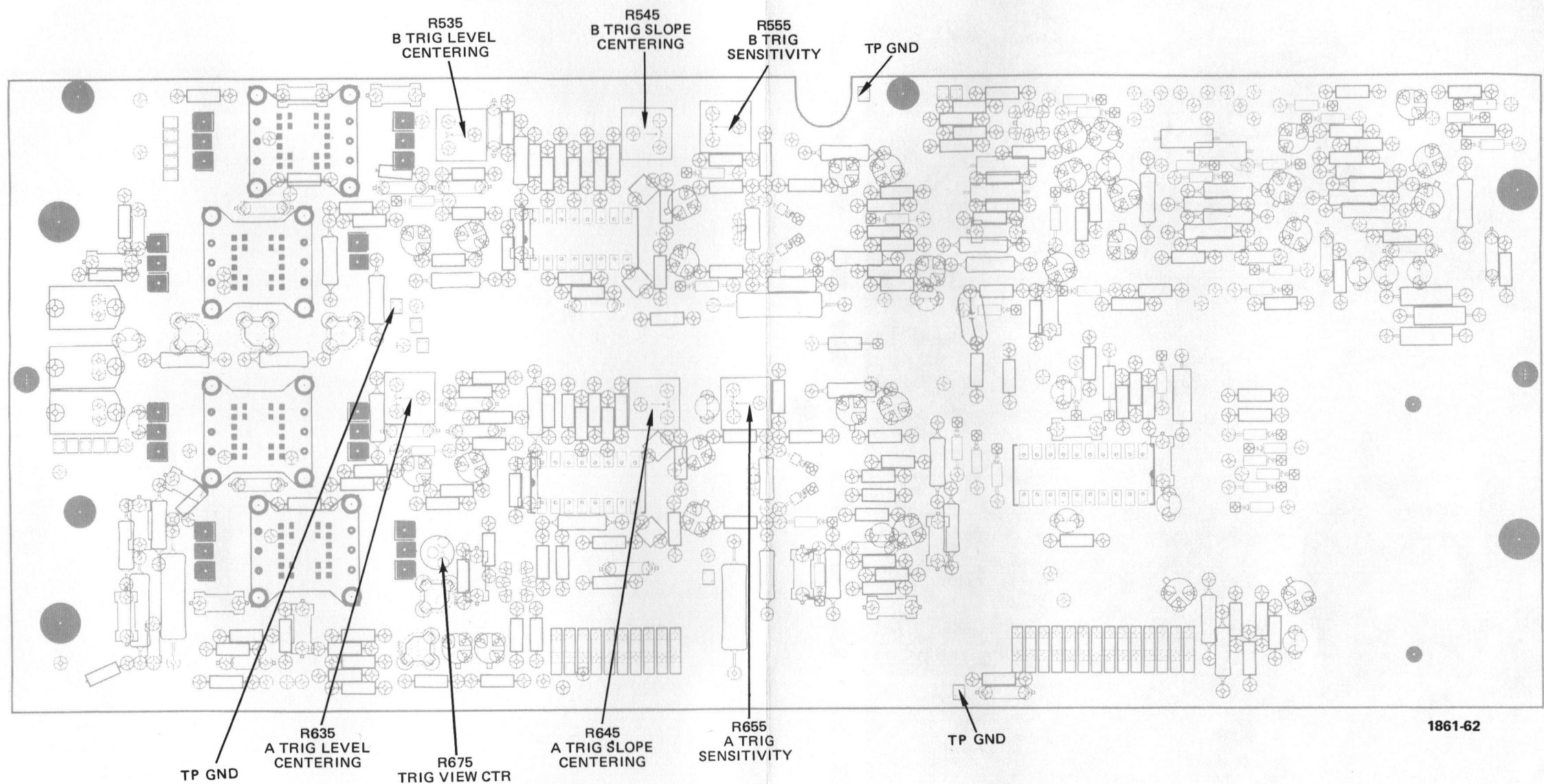
Fig. 8-16. Trigger Generator and Sweep Logic circuit board adjustment locations.
