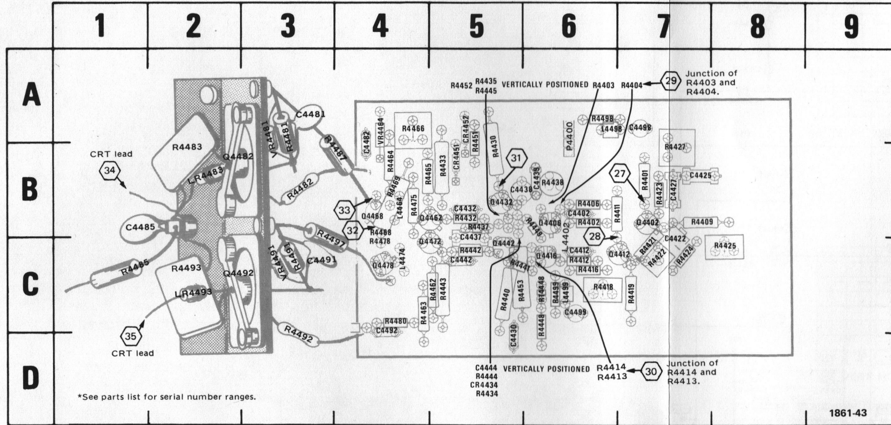
Fig. 8-4. A5a—Vertical Output Amplifier circuit board (discrete version).
