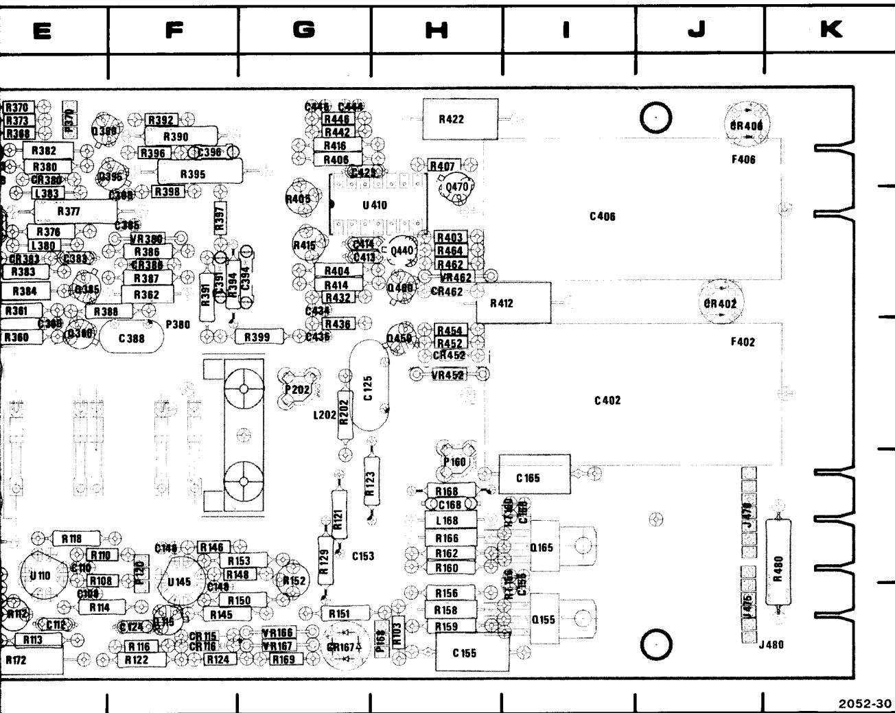
Amplifier circuit board with component locations of components (SN B030829 & below).
