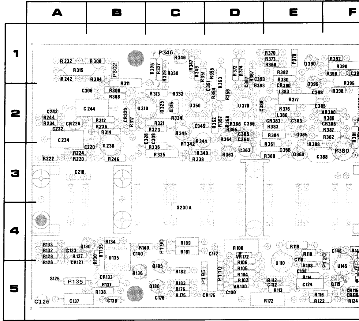
Fig. 7-1. A1—Amplifier circuit board with component loca
