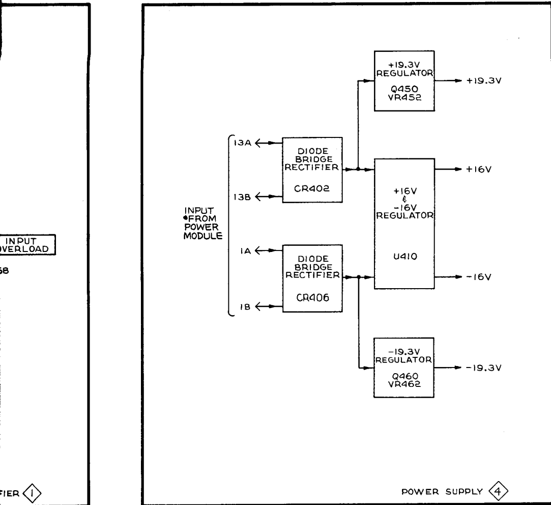
BLOCK DIAGRAM
