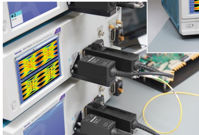
DPO70E Series Optical probes utilizing the ATI channel on the 70 GHz DPO70000SX Series Oscilloscope
