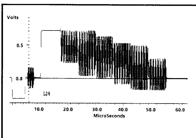
Fig. 4-11. 75% Colour Bars.
