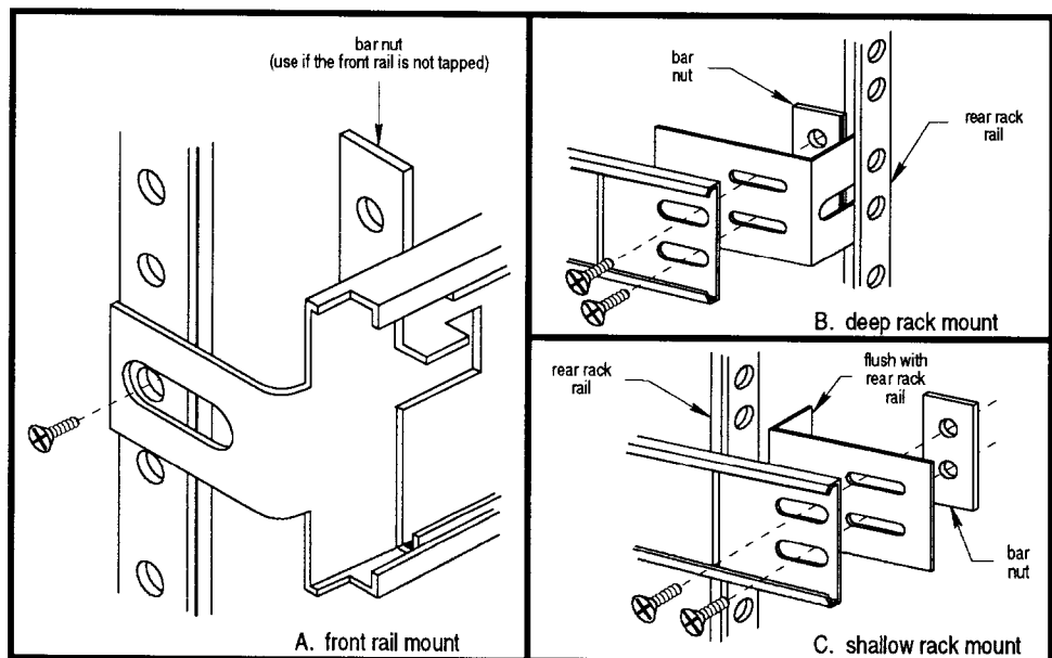
Figure 2-4. Mounting details.
