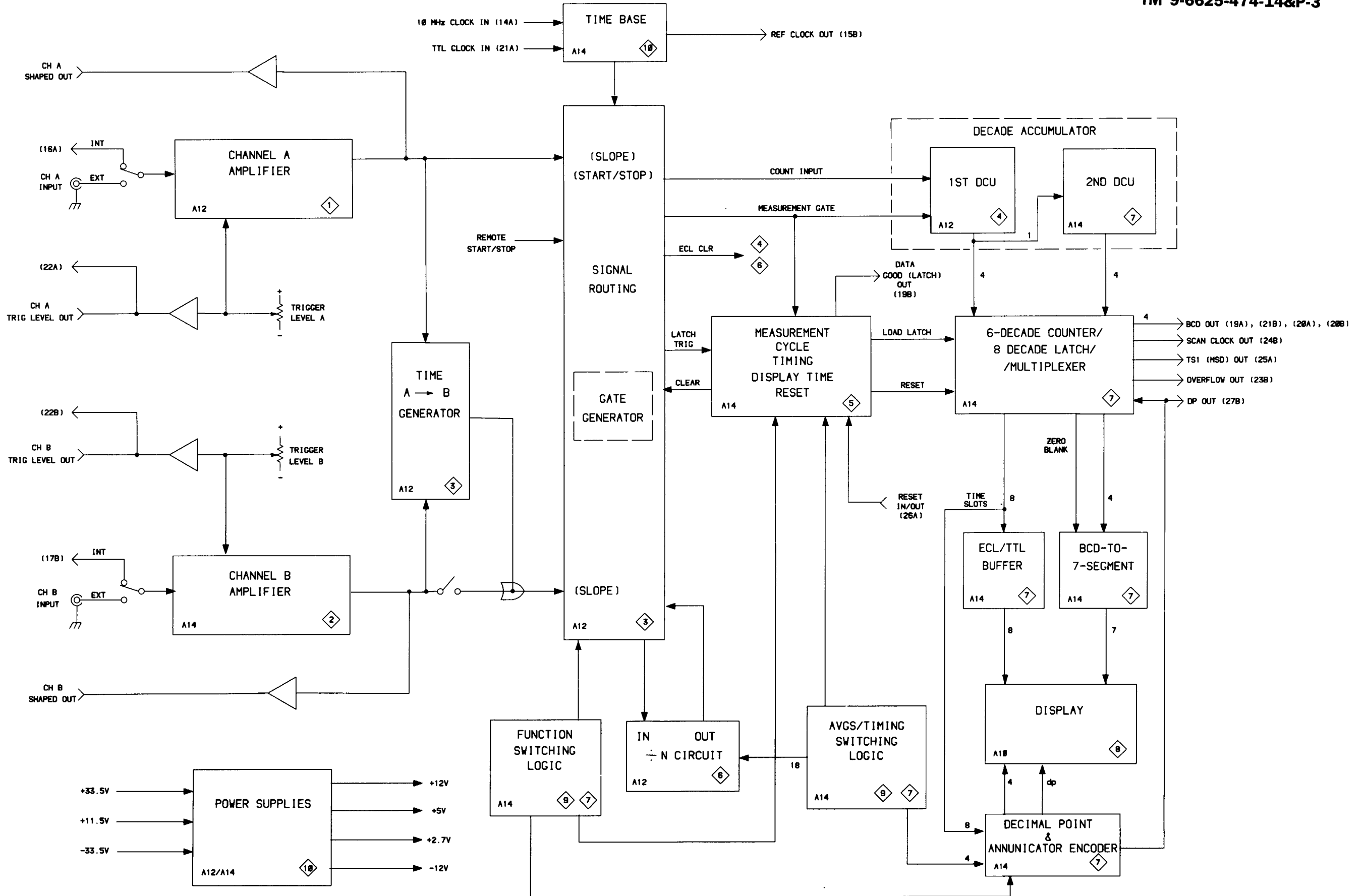
DC503A BLOCK DIAGRAM
