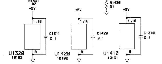
SIGNAL ROUTING, TIME A → B GENERATOR, & GATE GENERATOR
