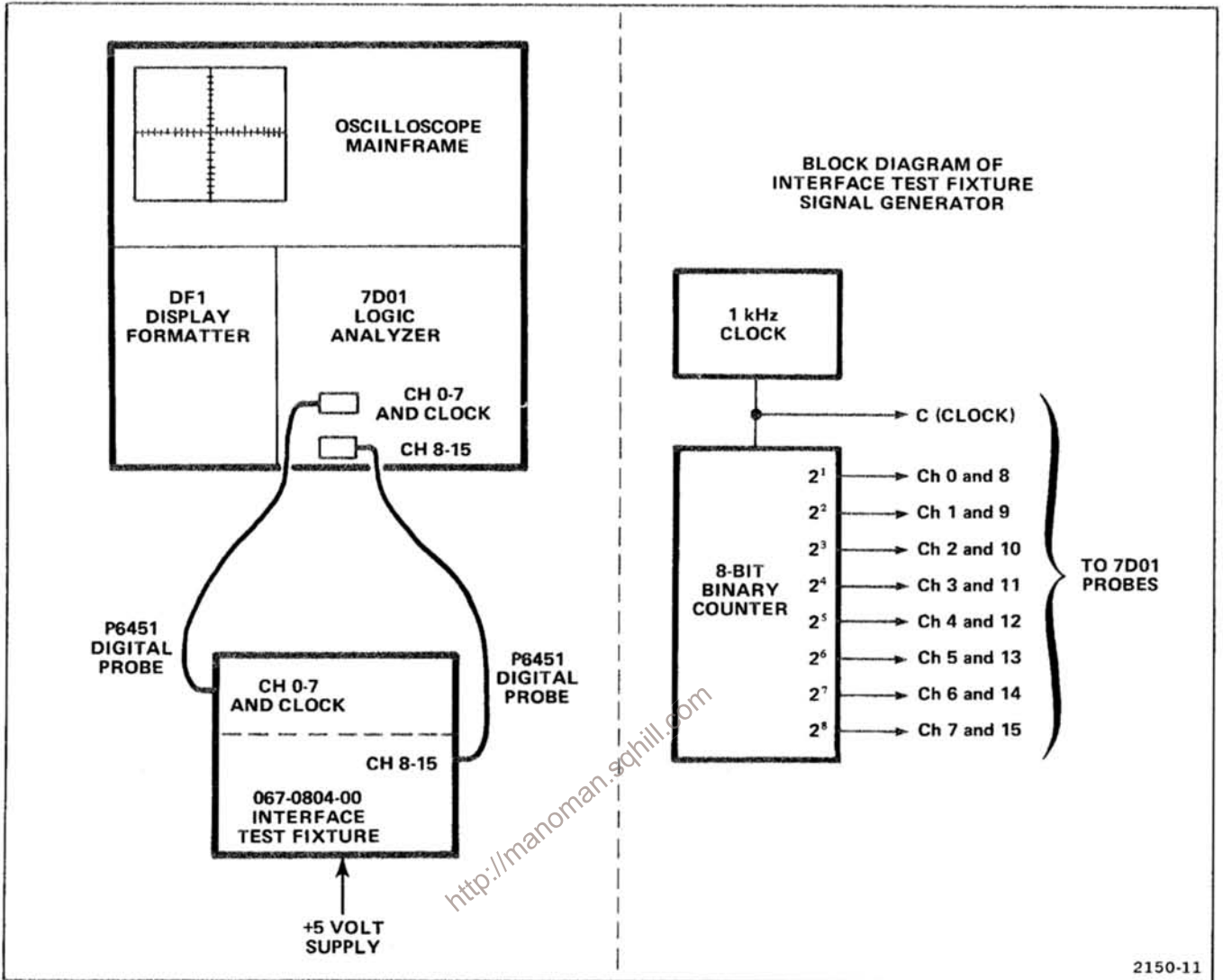
Figure 2-6. Test setup for Functional Check procedure.
