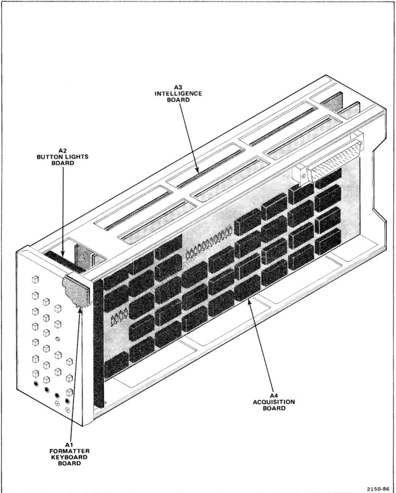
Figure 4-4. Circuit board locations.
