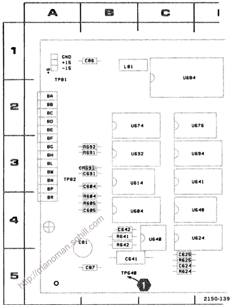
Figure 10-11. Partial A3--Intelligence circuit board. Component locations as viewed from the component side of the board.
