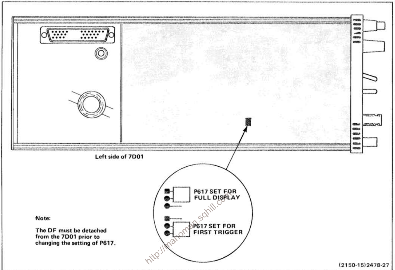
Figure 3-3. Location of 7D01 Full Display/First Trigger Selector.
