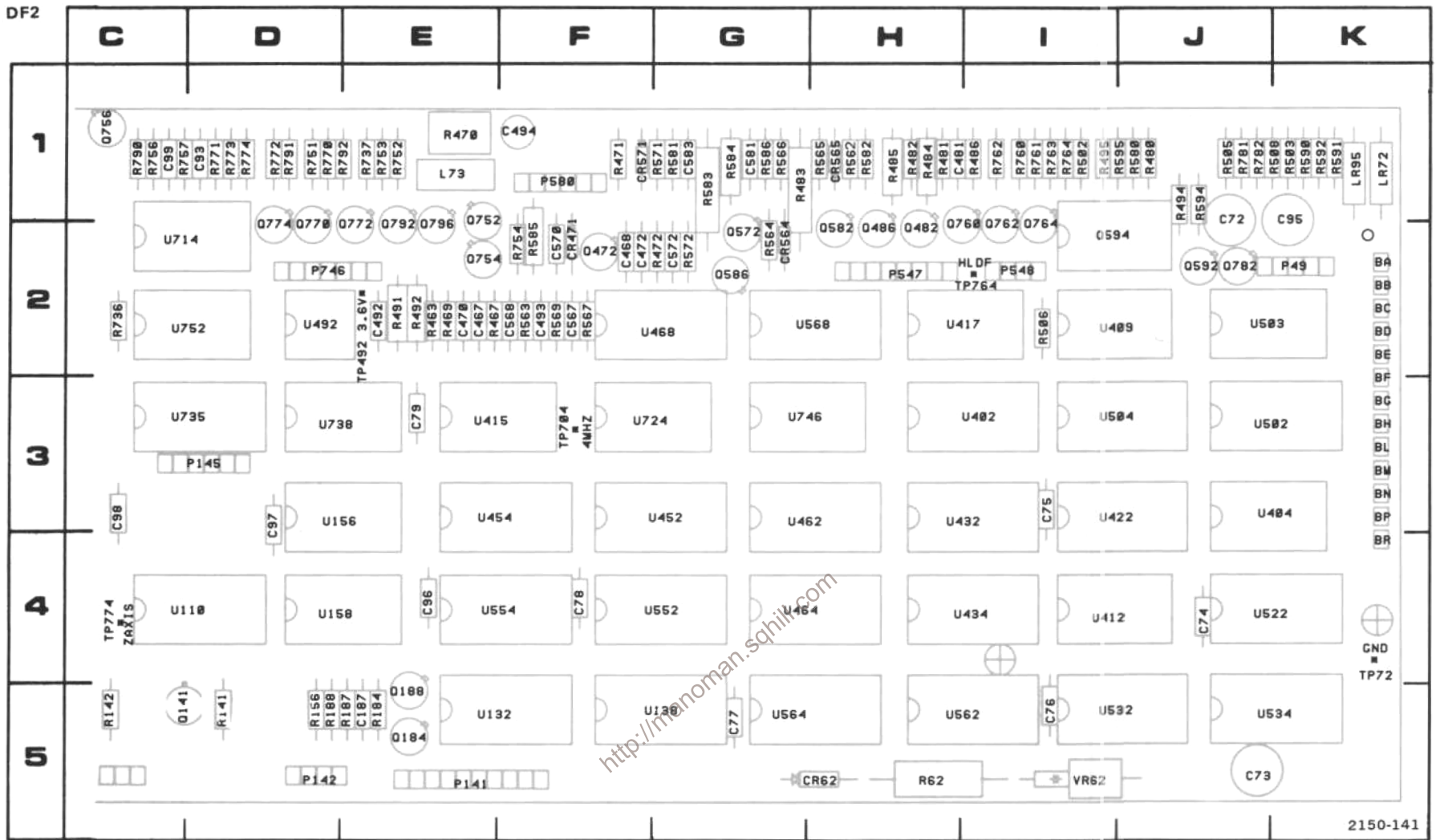
Figure 10-12. Partial A4—Acquisition circuit board. Component locations as viewed with board installed.
