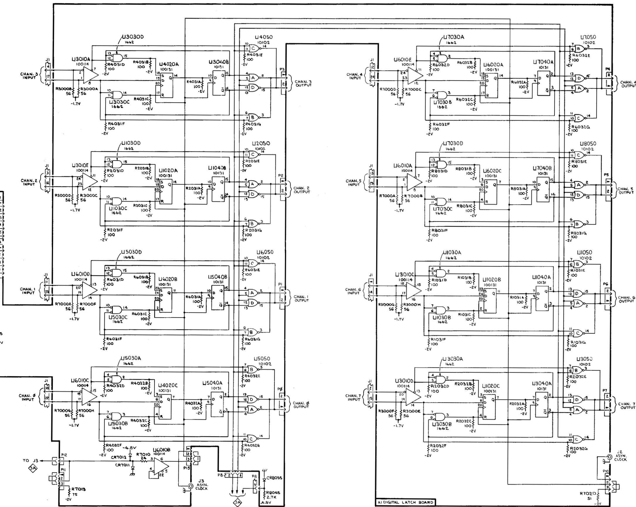
DIGITAL LATCH
