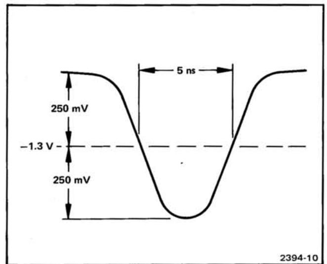
Fig. 3-5. 485 Oscilloscope Display.
