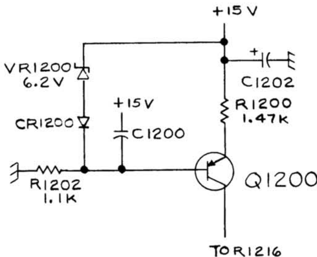
DIAGRAM 3 TRIG/GATE AND SINE SHAPER AMPLIFER - Partial
