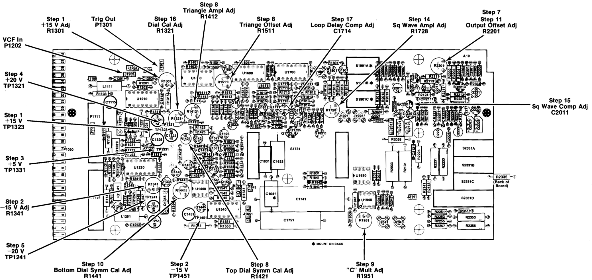
Fig. 8-2. Main Board.
