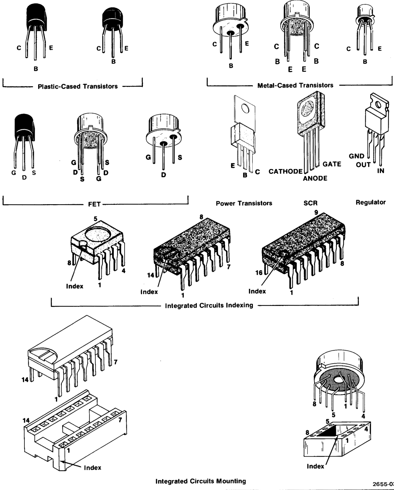
Fig. 5-1. Semiconductor Basing.
