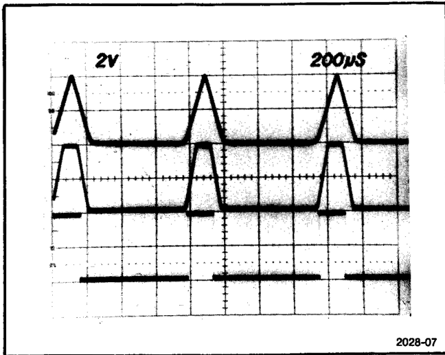
Fig. 2-9. VARIABLE RISE AND FALL TIMES. By varying the rise and fall times in the square wave mode various pulse shapes are formed.
