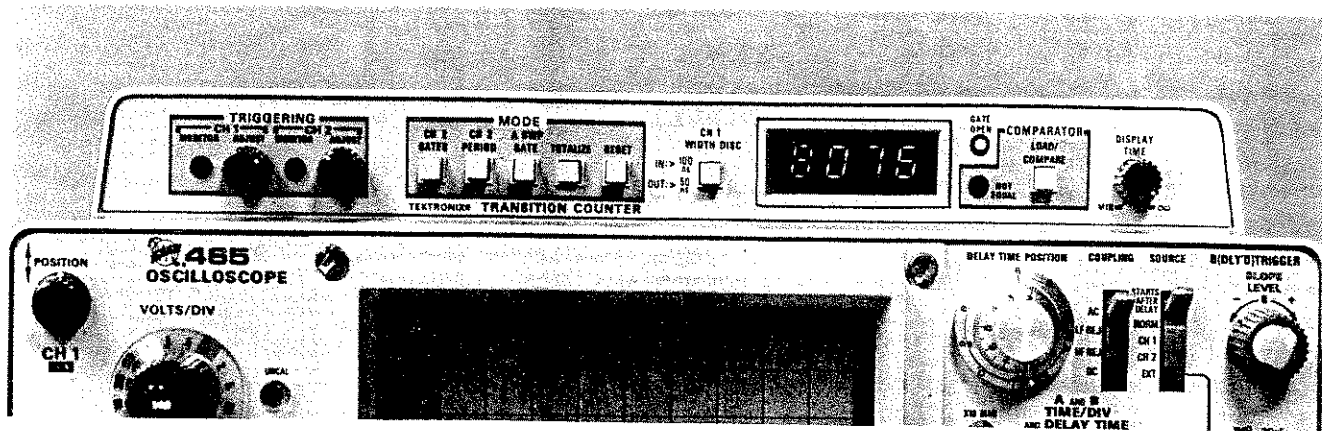
Fig. 1. The top of a 465 MOD 719A Oscilloscope, showing the controls and display window of a built-in digital counter. The oscilloscope probes may be used with the counter at the same time they are used for the scope. Input attenuators for the scope reduce the
