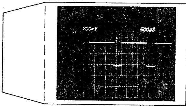
Fig. 12. Signal displayed using Variable Persistence storage. Note rising and falling portions are not visible.
