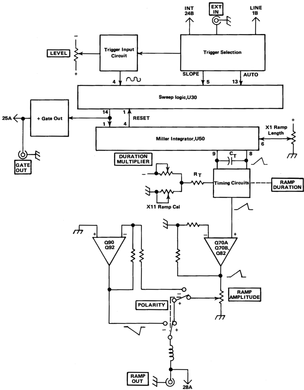
Fig. 5-1. Functional Block Diagram.
