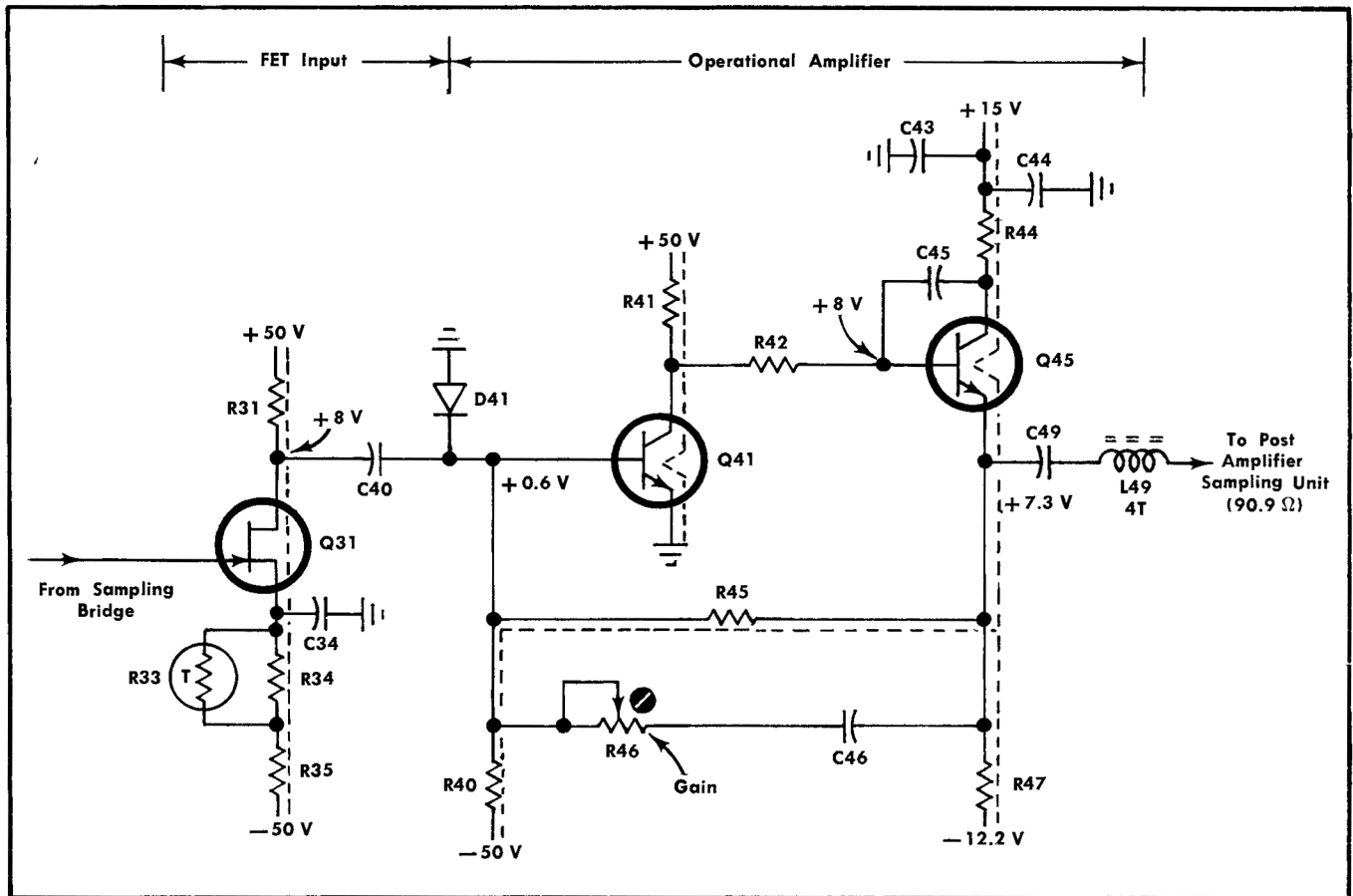
Fig. 3-3. Preamplifier circuit.
