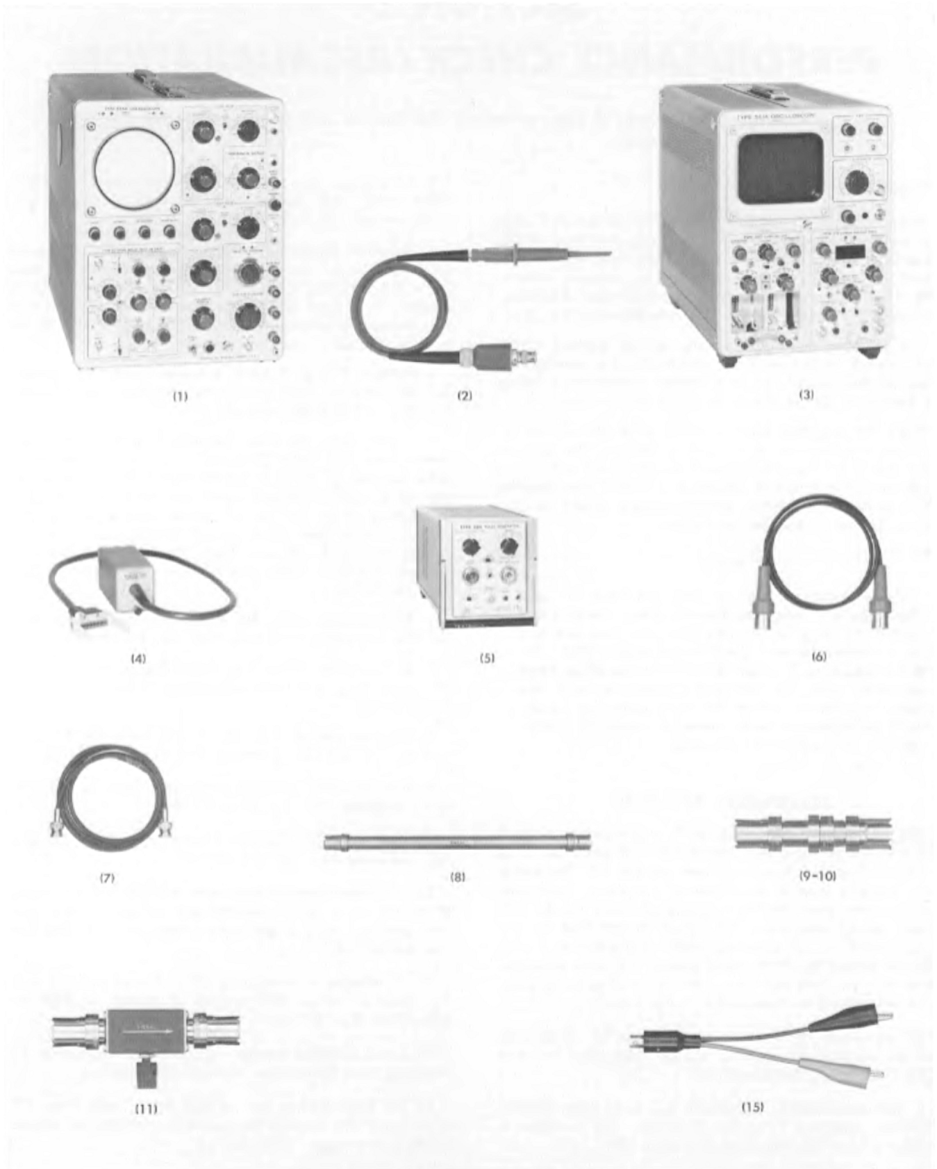
Fig. 5-1. Calibration Equipment.
