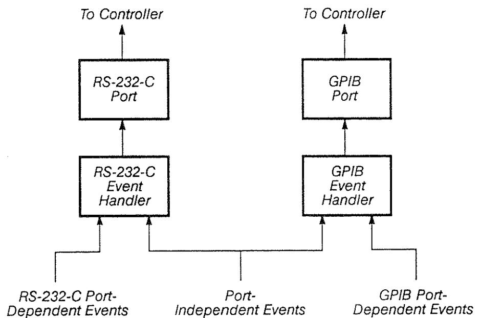
Remote Interface Status Reporting System Block Diagram
