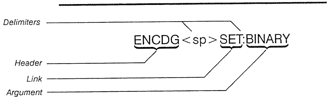
Example of Syntactic Elements
