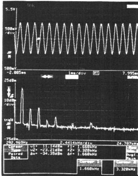
Figure 1. The TriStar Digital Signal Processor allows simultaneous display of "live" frequency-domain data concurrent with the real-time, time-domain signal.
