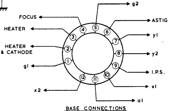
POWER SUPPLY & C.R.T. - D61
