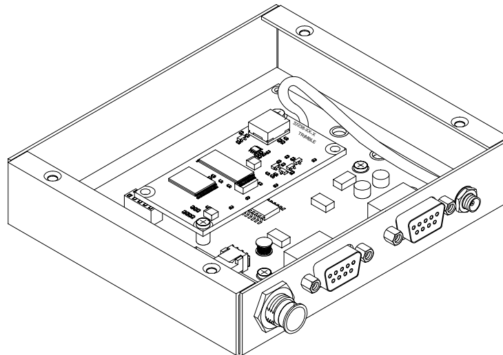
Figure 1-1. Receiver Module Installed in Interface Unit
