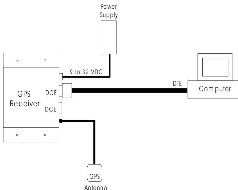
Figure 1-8. Interconnect Diagram
